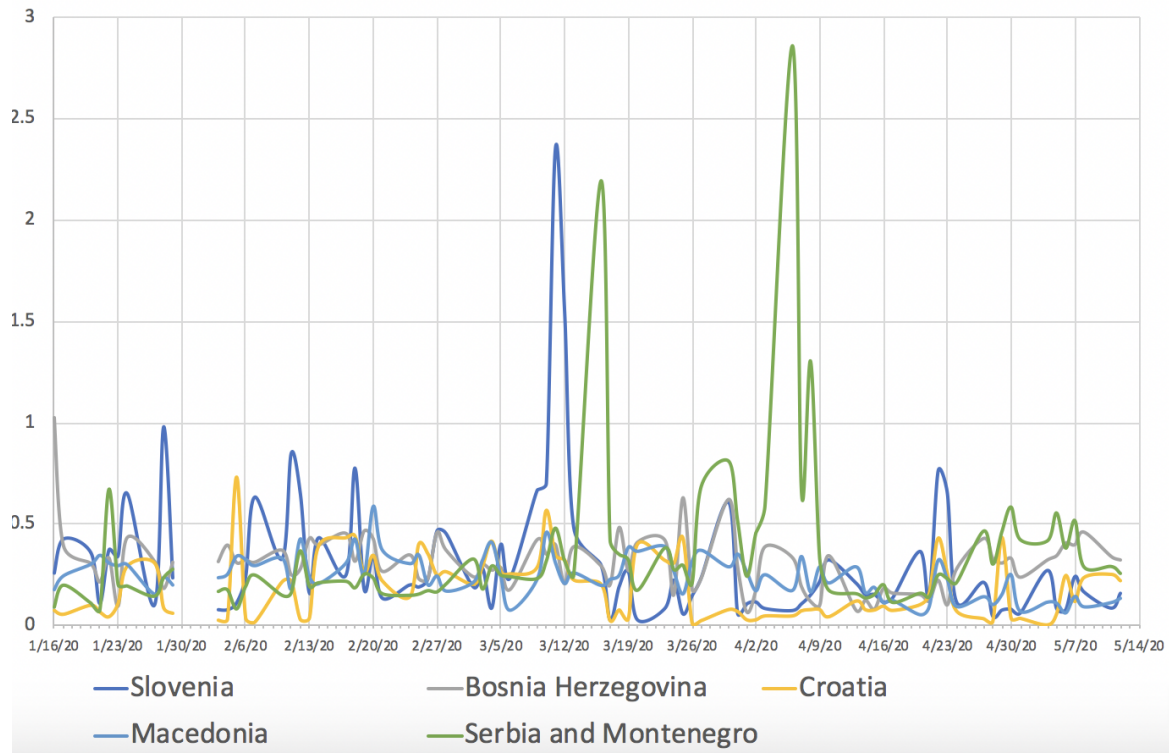
Balkans (without Albania) IPDV seen from SLAC
