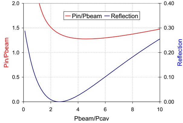
Figure 5.1: Efficiency of the transmitted power to the beam and reflected coefficient squared as a function of ratio of beam losses to cavity losses. Coupling factor \beta = 3.6 .
