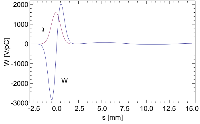
Figure 6.15: The wake of a \sigma_z = 0.5 mm Gaussian bunch in our model of the PEP-X vacuum chamber, which we use as a Green function wake in later instability calculations. Also shown is the bunch shape \lambda (with head to the left).
