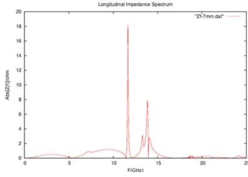
Figure 6.18: Longitudinal impedance spectrum of BPM.
