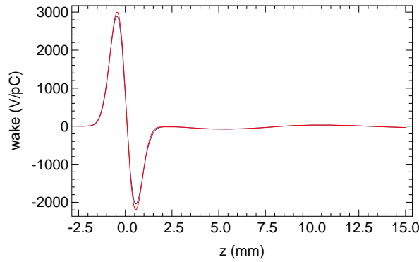
Figure 7.7: The total longitudinal wakefield of 0.5 mm bunch with (red line) and without (blue line) the CSR contribution.
