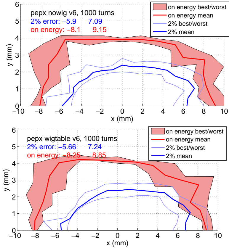
Figure 3.16: On and off-energy dynamic aperture with linear and nonlinear errors.
