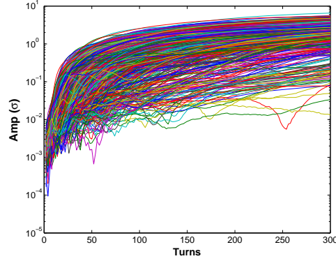
Figure 7.12: Simulated vertical amplitude of all bunches as a function of time. The beam consists of 19 bunch-trains. The amplitude is normalized by the beam size.
