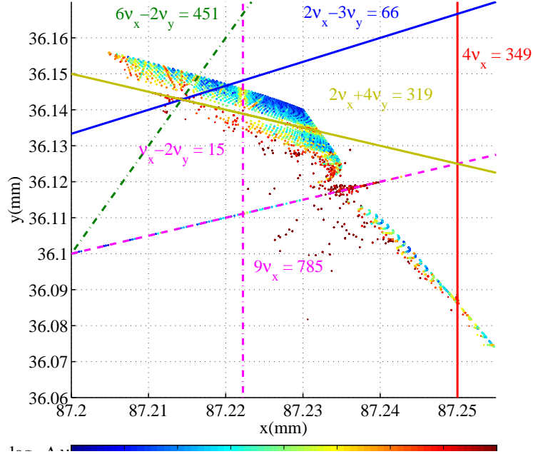
Figure 3.5: Frequency map of tune footprint .
