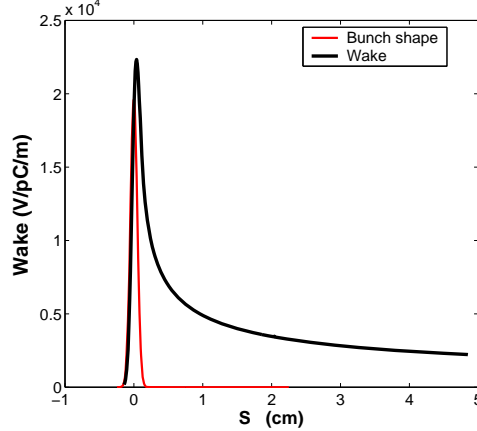
Figure 7.8: Transverse resistive wall wake convoluted with 0.5 mm Gaussian bunch.
