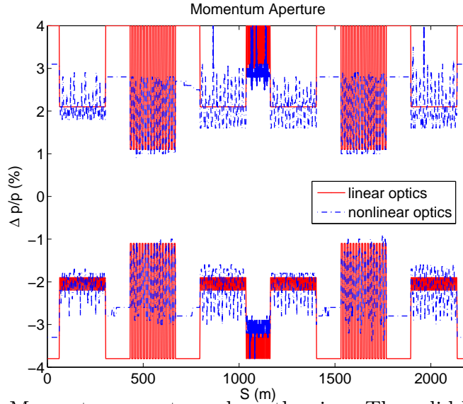
Figure 3.11: Momentum aperture along the ring. The solid line is the transverse momentum aperture of linear optics in Eq.(3.4). The dashed line is the transverse momentum aperture takes into consideration of nonlinear optics due to off momentum. Because the RF momentum of 5.6 % is larger than the transverse momentum. The transverse momentum aperture shows here is also the momentum aperture of PEP-X.
