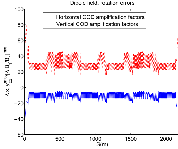
Figure 3.17: Dipole amplification factor.
