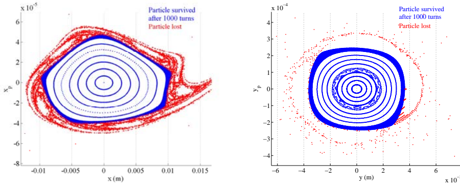
Figure 3.7: Phase space tracking of horizontal plane (left plot) and vertical plane (right plot) of on momentum particles. Each torus is constructed by tracking of 1000 turns.
