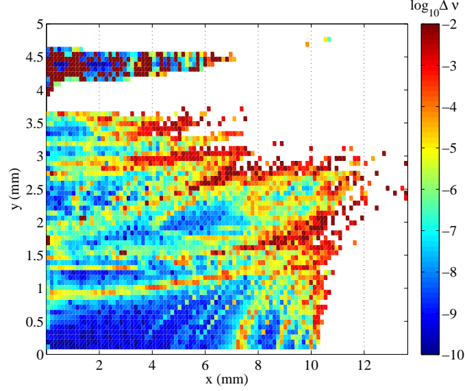
Figure 3.6: Frequency map of amplitude dependent.
