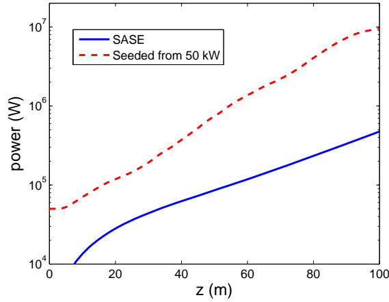
Figure 8.2: Power evolution for a soft x-ray SASE FEL at \lambda_r = 3.3 nm. For comparison, we also included a seeded FEL simulation (see Table 8.1 and discussions in Sec. ??).
