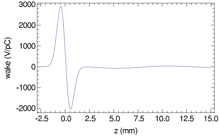
Figure 7.1: Longitudinal wakefield for a 0.5 mm bunch. Positive values of the wake correspond to energy loss, and positive values of the coordinate z is behind the source particle.
