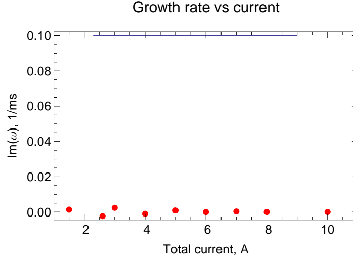
Figure 7.3: The growth rate of the microwave instability as a function of a total beam current in the ring.
