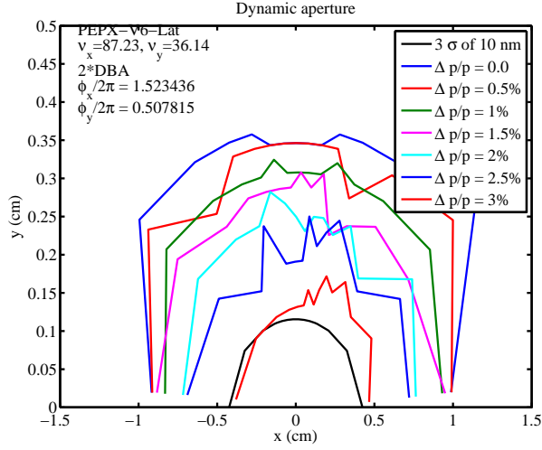
Figure 3.4: Dynamic aperture tracking of the bare lattice at different energy.
