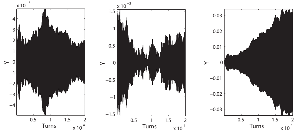
Figure 7.10: Simulated dipole oscillations in vertical plane for different bunch currents: (left) 0.78 mA; (middle) 0.79 mA and (right) 0.80 mA
