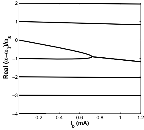
Figure 7.9: TMCI in PEP-X due to the resistive wall impedance
