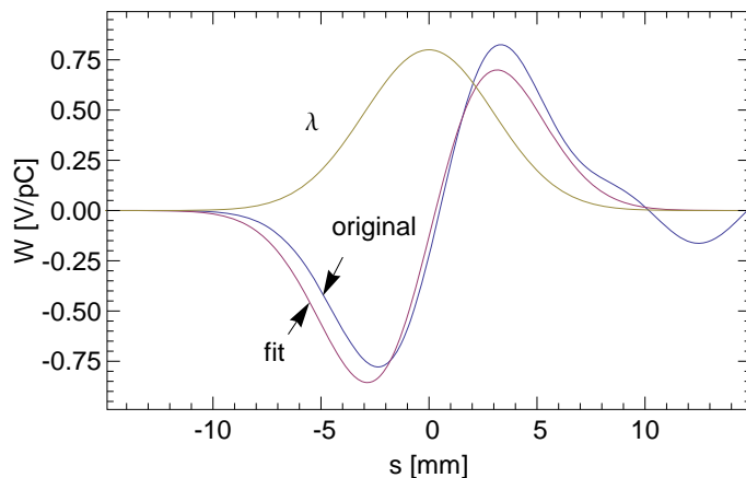
Figure 6.13: The wake for a pair of undulator transitions, for a \sigma_z = 3 mm Gaussian bunch (blue), and the fit to a series R + L wake (red). Also shown is the bunch shape \lambda (with head to the left).
