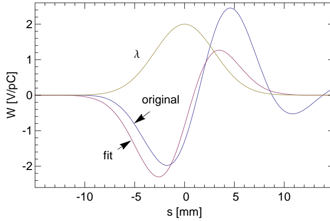
Figure 6.14: The wake for a pair of wiggler transitions, for a \sigma_z = 3 mm Gaussian bunch (blue), and the fit to a series R + L wake (red). Also shown is the bunch shape \lambda (with head to the left).
