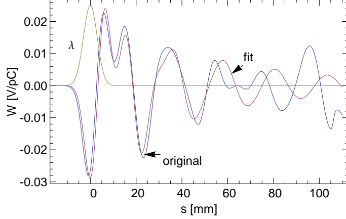
Figure 6.12: The BPM wake for a \sigma_z = 3 mm Gaussian bunch (blue), and the two resonator fit (red). Also shown is the bunch shape \lambda (with head to the left).
