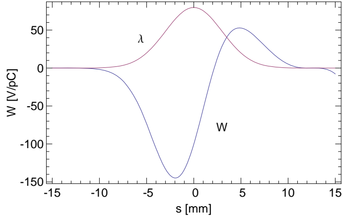
Figure 6.16: The wake of a nominal \sigma_z = 3 mm Gaussian bunch in our model of the PEP-X vacuum chamber. Also shown is the bunch shape \lambda (with head to the left).
