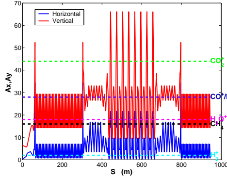
Figure 7.11: Critical mass number along the ring. The mass number of H_2 , CH_4 , H_2O , CO and CO_2 is marked in the plot.
