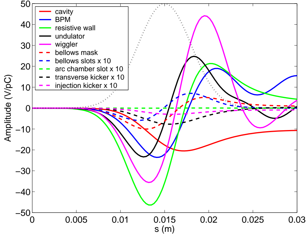
Figure 6.10: Contributions of vacuum chamber components to the total longitudinal short-range wakefield of the ring. Note that the wakefields of the kickers, arc chamber and bellows slots are scaled by a factor of 10.
