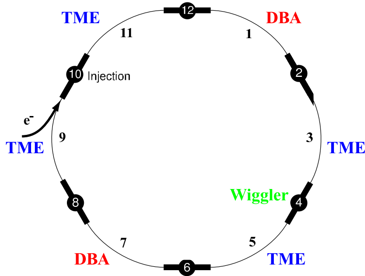
Figure 2.1: PEP-X layout with 2 DBA arcs, 4 TME arcs and 6 straight sections.
