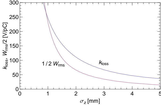
Figure 6.17: Minus the first moment of the wake (the loss factor k_{loss} ) and the second moment of the wake W_{rms} as functions of bunch length (for a Gaussian bunch) induced by the PEP-X impedance.
