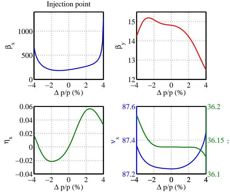
Figure 3.9: Optics functions at injection point as function of off momentum \delta .
