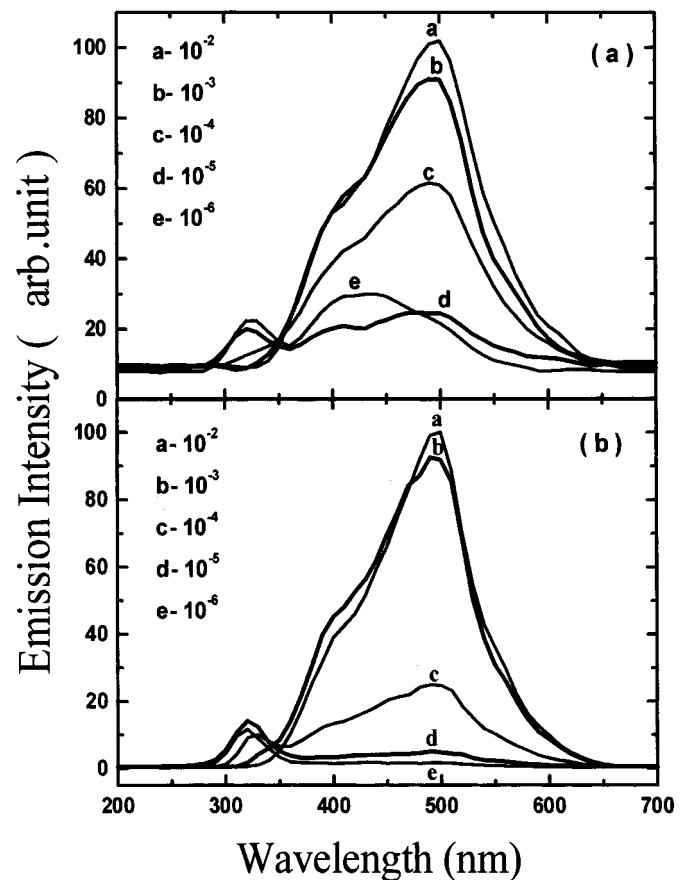
Fig. 1. Measured emission spectra of the CsI(Tl) crystal with [Tl + ] of 10 -6 , 10 -5 , 10 -4 , 10 -3 , and 10 -2 mol under (a) gamma-rays and (b) alpha particles excitations.
