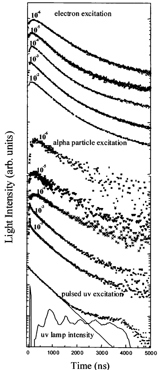
Fig. 3. Decay curves of the CsI crystals with 10^{-6} , 10^{-5} , 10^{-4} , 10^{-3} , and 10^{-2} mol under electron and alpha particle excitations. The decay curve of the CsI crystal with 10^{-3} mol under pulsed UV excitation is also shown together with the time profile of the pulsed UV lamp. The solid line represents the fitted decay curve for an exponential function for the time range up to 1500 ns.
