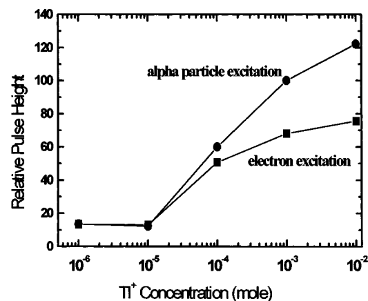
Fig. 2. Relative pulse height against [Tl + ] under electron and alpha particle excitations. Pulse heights were normalized at the lowest [Tl + ] = 10 -6 mol.
