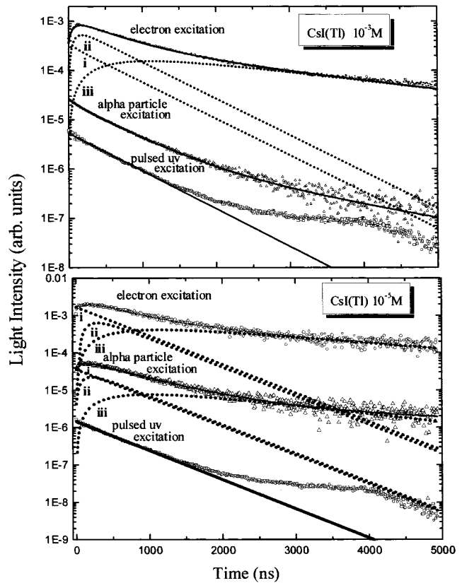
Fig. 4. Decay curves and their fitted curves of CsI crystals with [TI^+] of 10^{-3} mol (no rising part) and 10^{-5} mol (rising part) under electrons excitation compared with those of alpha particle and pulsed UV excitations.
