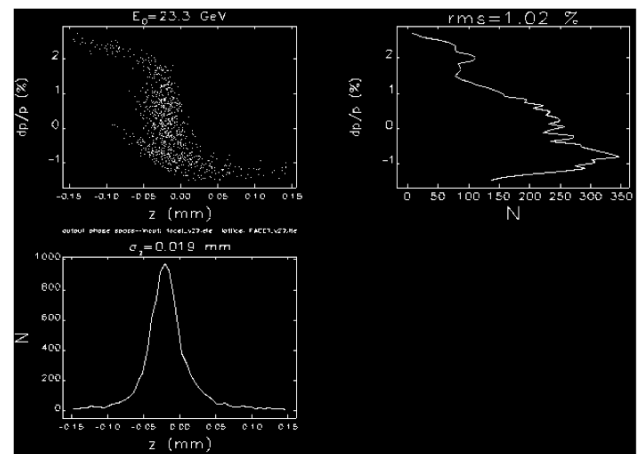
Figure 4: The simulated longitudinal phase space, energy spectrum and current profile at the location of BLEN for the FACET beam.
