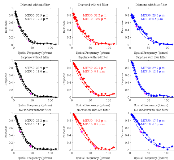
Figure 6: Resolution of the Nikkor 105mm f/2.8D lens at a magnification of 1:1 and an aperture of f/11 . Solid lines are third order polynomial fits to the CTF data (*) and dashed lines are the MTF curves derived from CTF.
