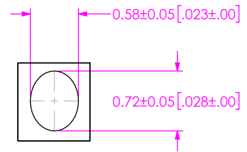
DETAIL 'B' SCALE 16:1
