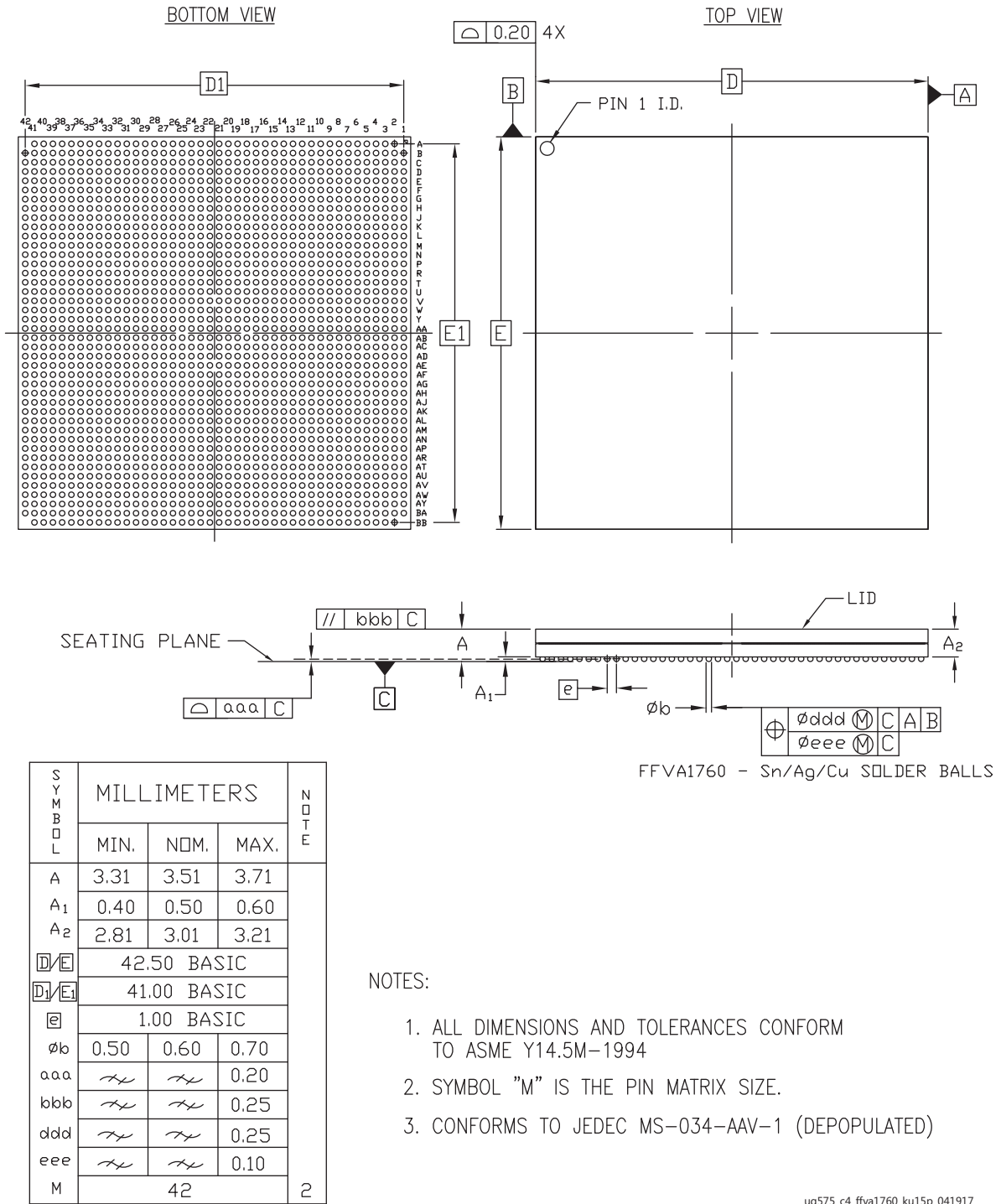
Figure 4-27: Package Dimensions for FFVA1760 (XCKU15P)
