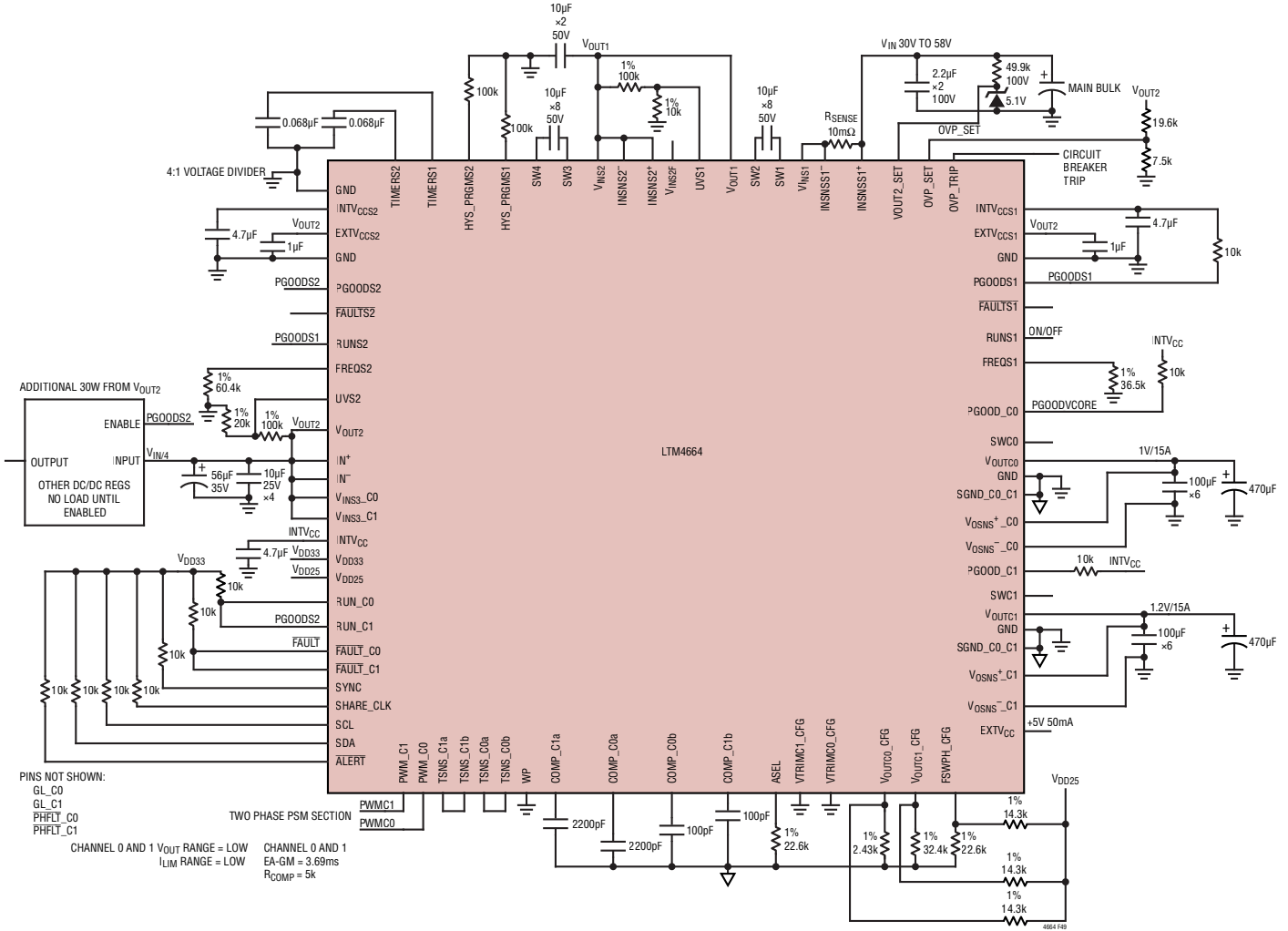
Figure 49. 30V – 58V to 1V and 1.2V at 15A, with Additional 30W from V OUT2 . Integrated Power System Management Features Accessible Over 2-Wire I 2 C/SMBus/PMBus Serial Interface. For Evaluation and More Information, See Demo Boards DC2143
