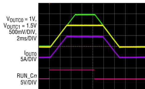
48V IN , 10A LOAD ON V OUT0 , NO LOAD ON V OUTC1 , TON_RISE 0 = 3ms, TON_RISE 1 = 4.5ms, TOFF_DELAY 1 = 0ms, TOFF_DELAY 0 = 1.5ms TOFF_FALL 1 = 4.5ms, TOFF_FALL 0 = 3ms, ON_OFF_CONFIG n = 0x1E
