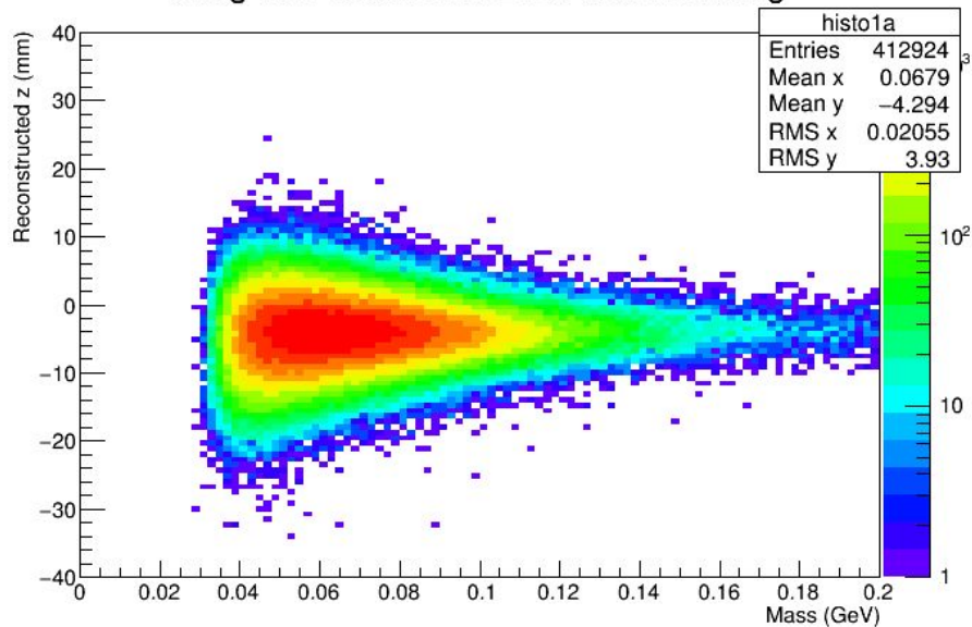
tritrig-wab-beam 10% L1L2 with Hit Killing
