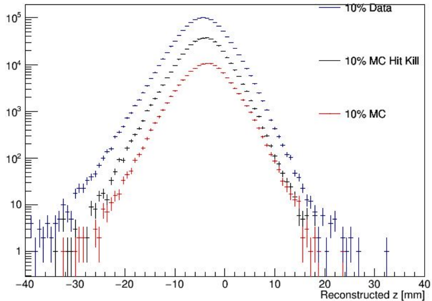
Reconstructed z
