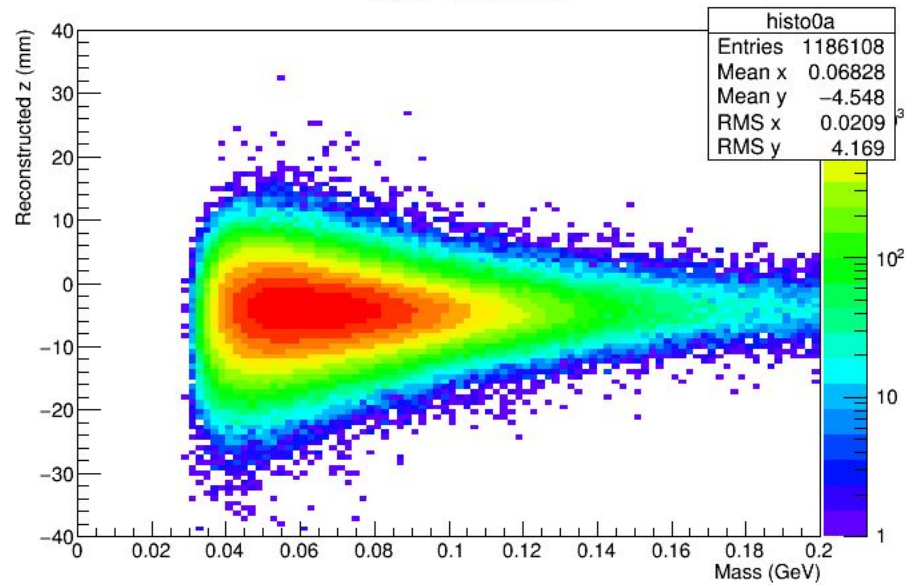
Data 10% L1L2
