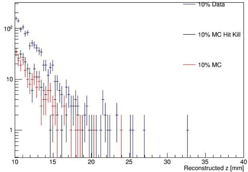
Reconstructed z
