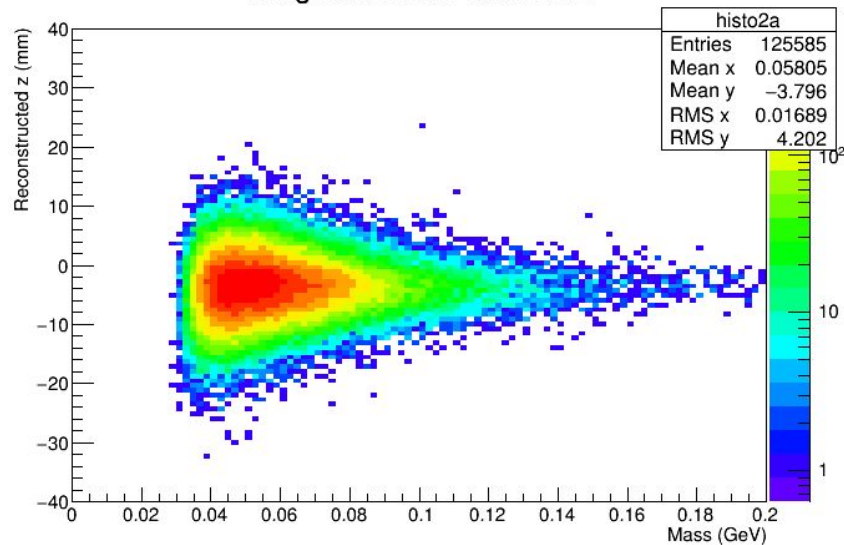
tritrig-wab-beam 10% L1L2
