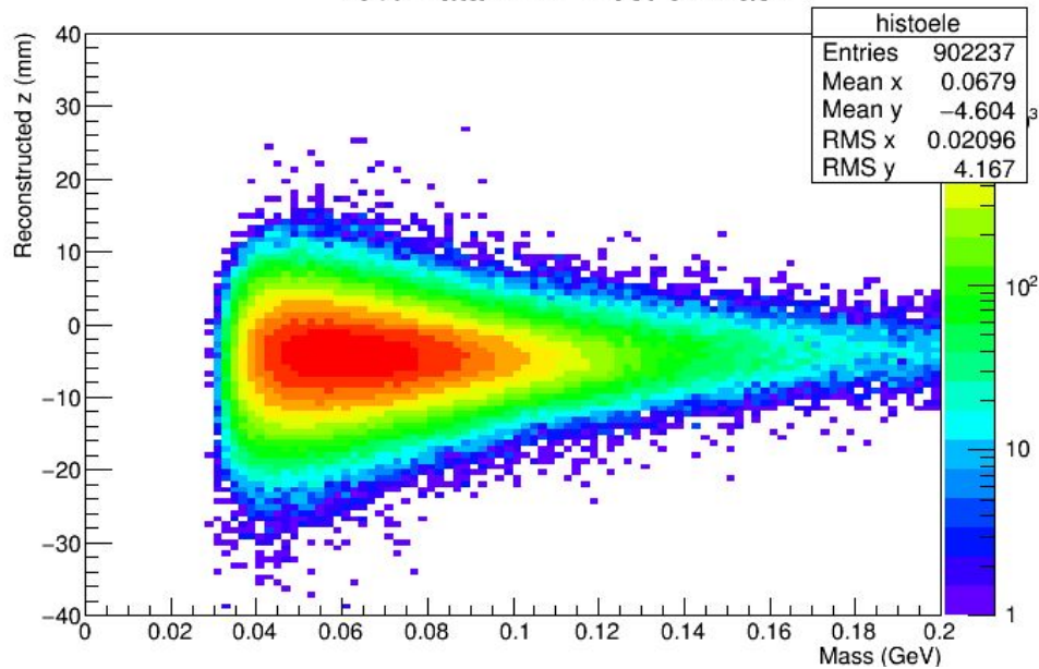
10% Data L1L2 Electron Has L1
