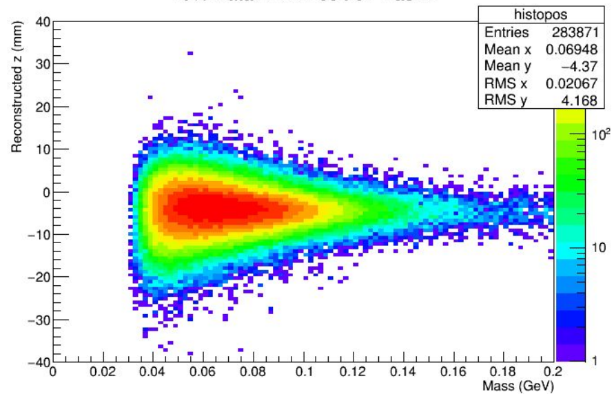
10% Data L1L2 Positron Has L1
