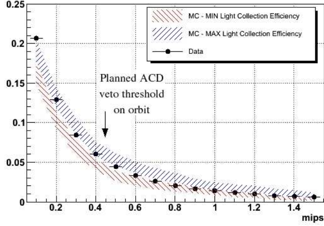
Figure 1: Backsplash distribution for an ACD tile as obtained from beam test data (black points) and Monte Carlo expectations. In every case, backlash is expressed as the fraction of events for which the signal in the tile is above a given threshold. The error bars in the data are statistical ( 1\sigma ). Monte Carlo simulations consider two extreme scenarios of light collection inefficiency through the tile edge. In the MIN light collection efficiency scenario, the efficiency decreases linearly from 100% (3 cm away from the edge) to 70% at the tile edge. In the MAX case, the collection efficiency decreases linearly from 100% (0.5 cm away from the edge) to 95% at the tile edge. Both scenarios are shown in the backlash distribution as “bands” that bracket the expected backlash distribution. The width of each band is given by twice the statistical error ( 2\sigma ) obtained from the simulation.
