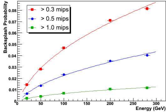
Figure 2: Energy dependence of backlash in tile 110 for different thresholds. The data is reasonably well fitted by a function of the form \sqrt{E} .
