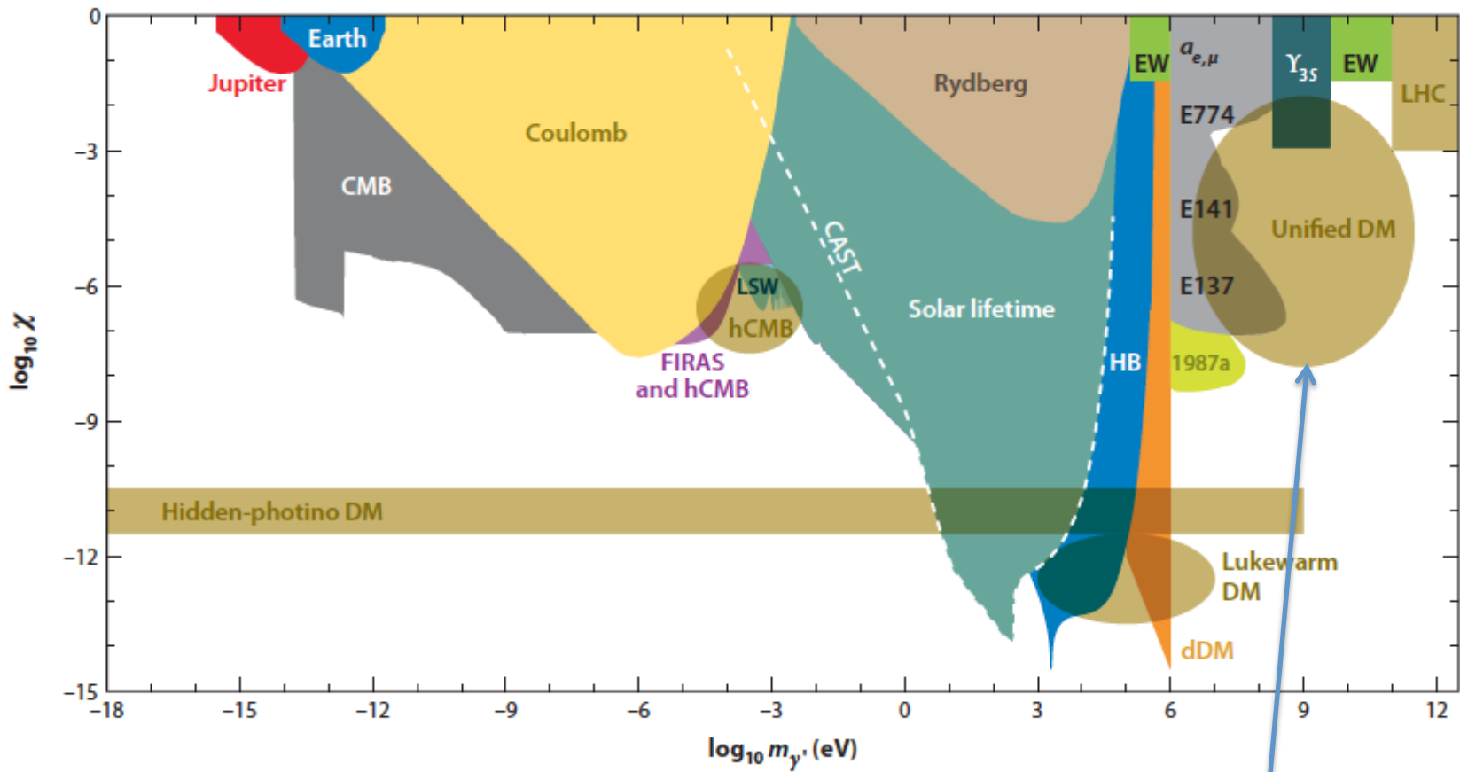
Jaeckel and Ringwald, Annu. Rev. Nucl. Part. Sci. 2010.60:405-437
