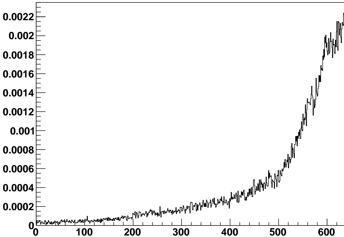
module_L4t_halfmodule_stereo_hole_sensor0 - Occupancy
