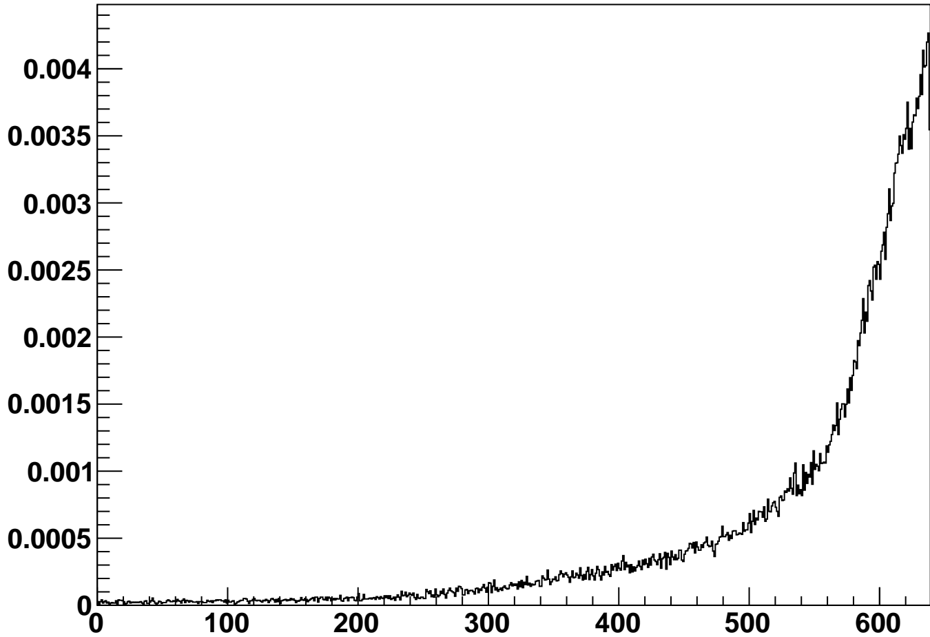
module_L3t_halfmodule_stereo_sensor0 - Occupancy
