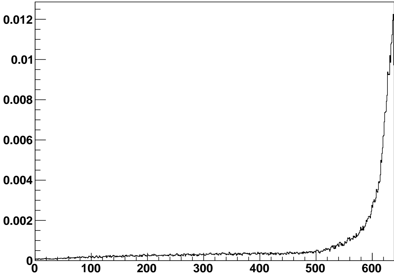
module_L1t_halfmodule_stereo_sensor0 - Occupancy
