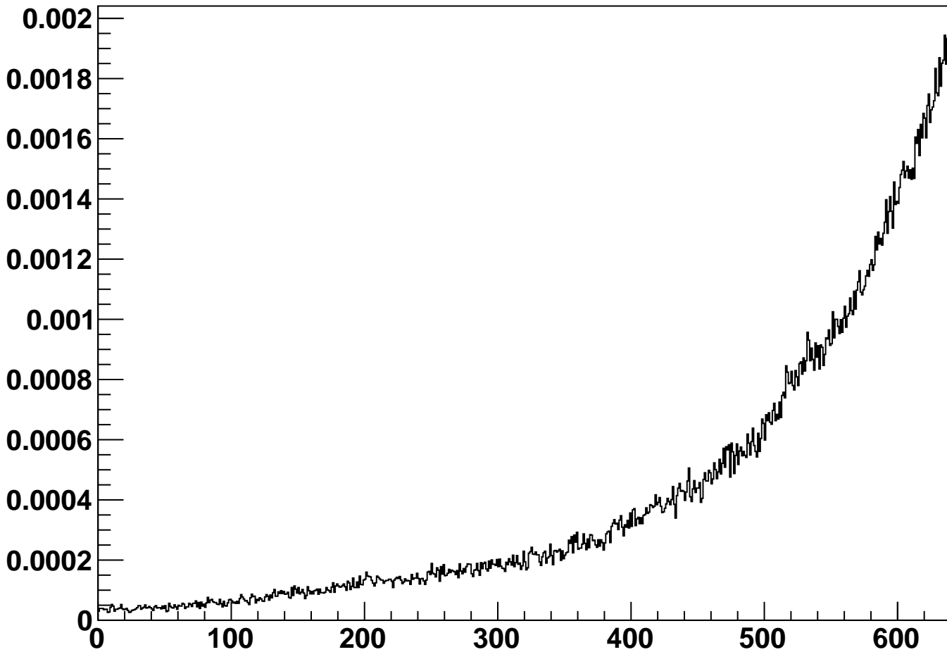
module_L5t_halfmodule_stereo_hole_sensor0 - Occupancy
