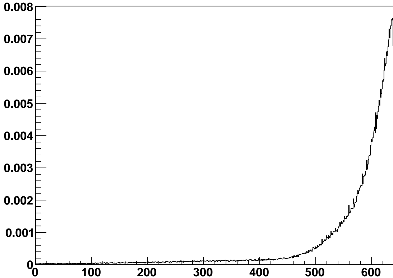
module_L2t_halfmodule_stereo_sensor0 - Occupancy
