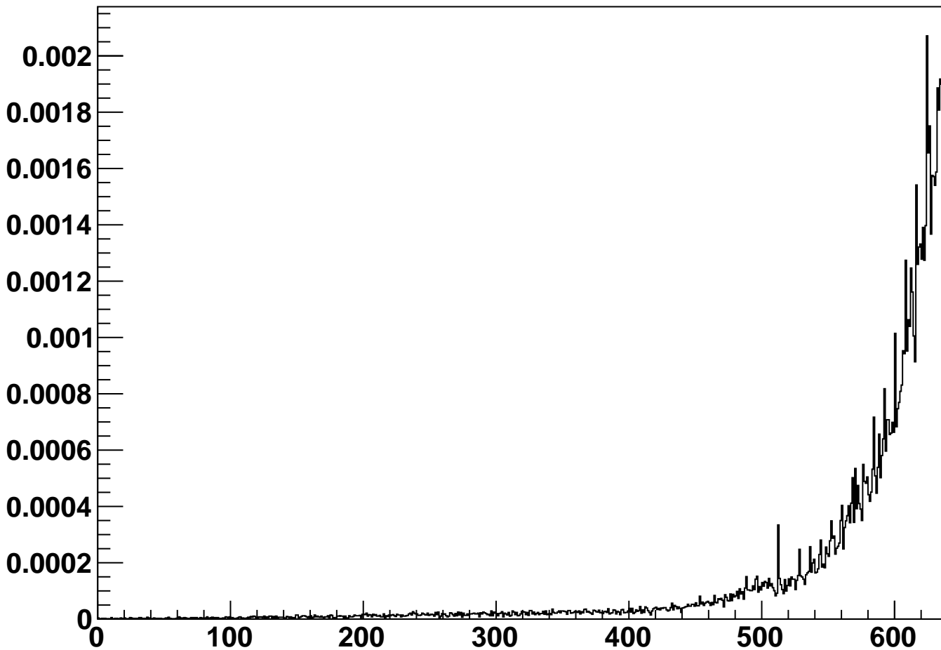
module_L2b_halfmodule_stereo_sensor0 - Cluster Occupancy
