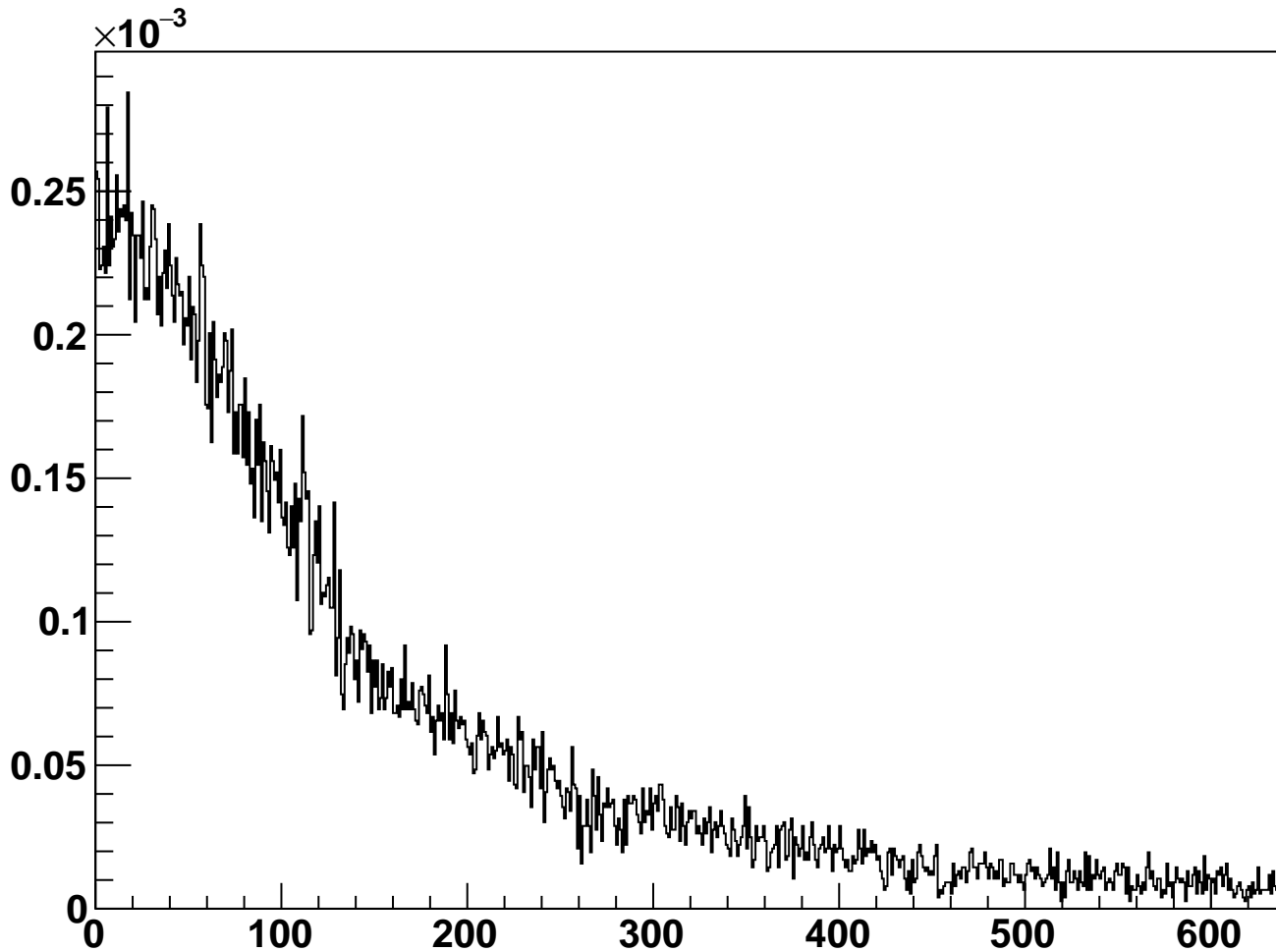
module_L6t_halfmodule_axial_hole_sensor0 - Cluster Occupancy
