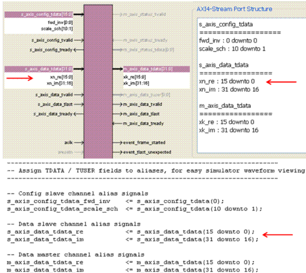
Figure 4-9: TDATA Port Structure
