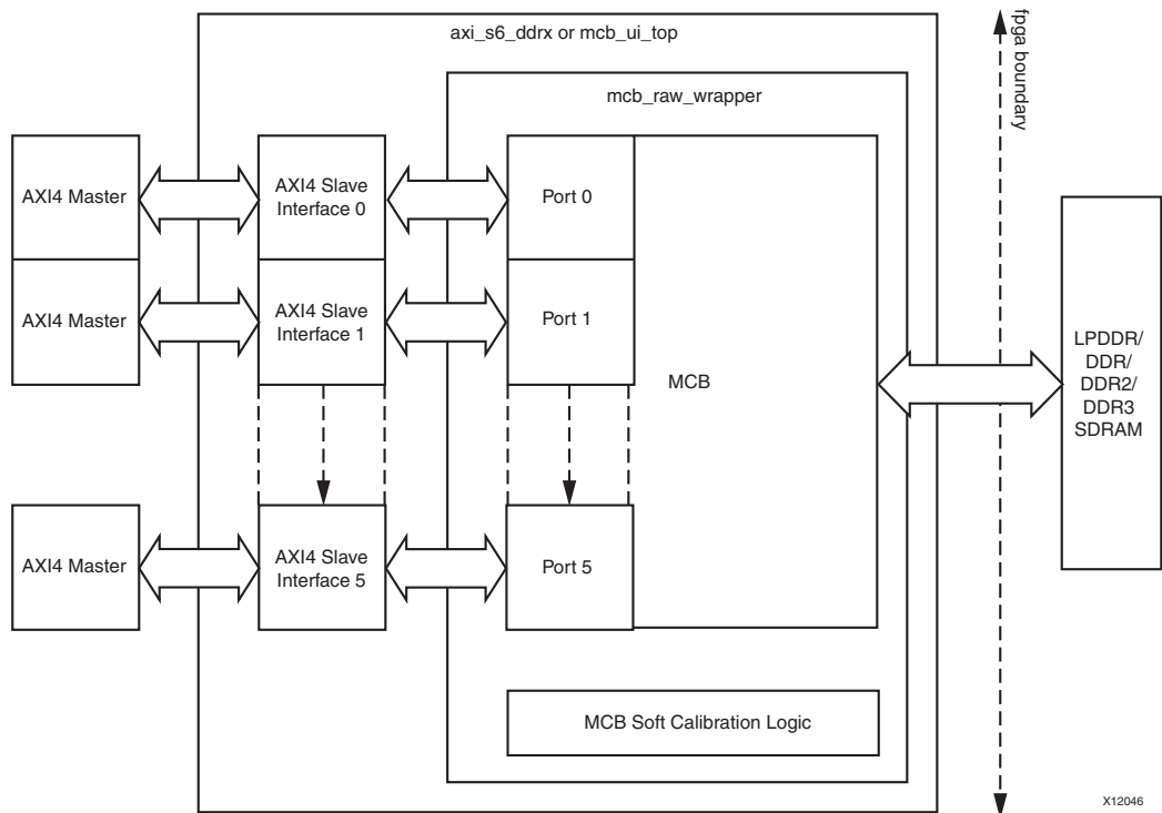
Figure 2-24: Spartan-6 Memory Solution Block Diagram
