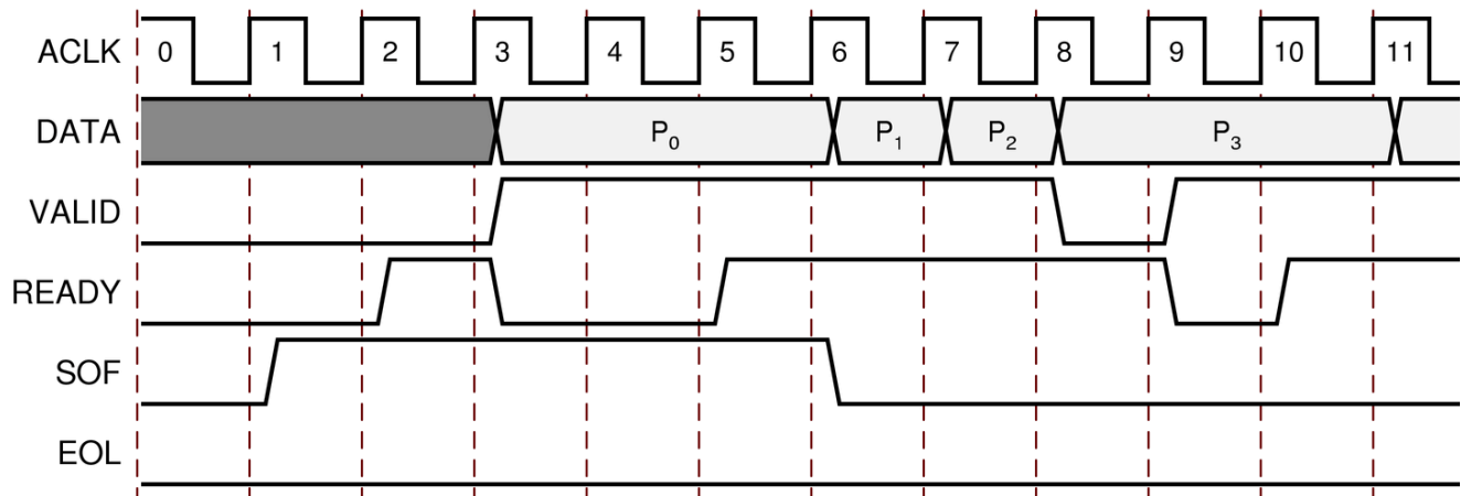
Figure 3-16: Use of EOL and SOF Signals
