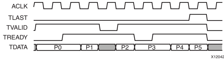
Figure 4-3: AXI4-Stream Waveform
