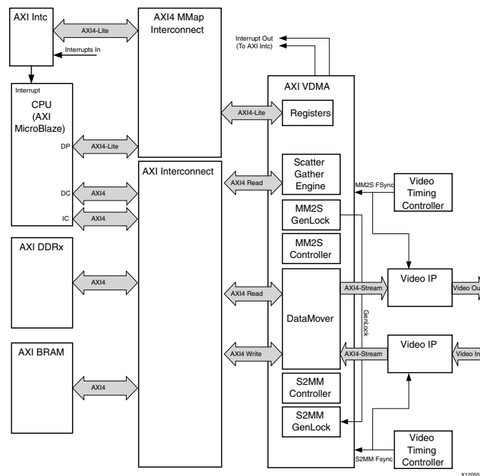
Figure 2-22: Typical Use Case for AXI VDMA and Video IP
