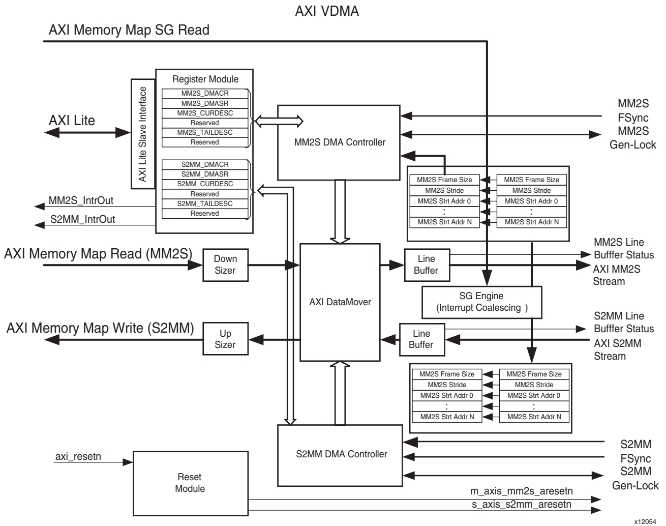
Figure 2-21: AXI VDMA High-Level Block Diagram
