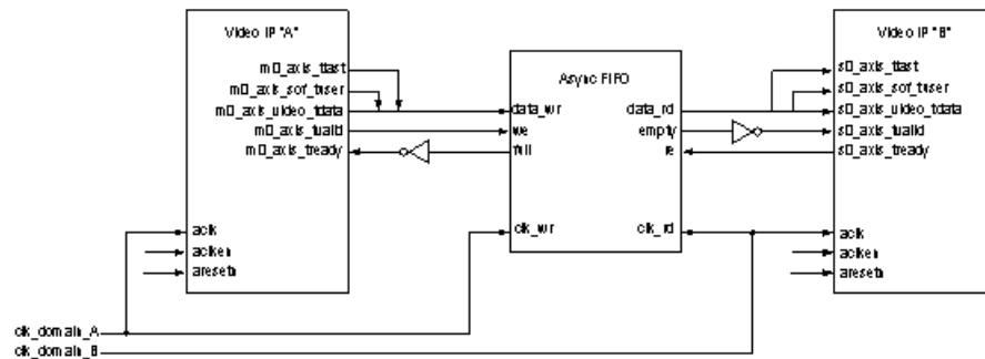
Figure 3-14: Connecting AXI4-Stream Video Interfaces in Different Clock Domains
