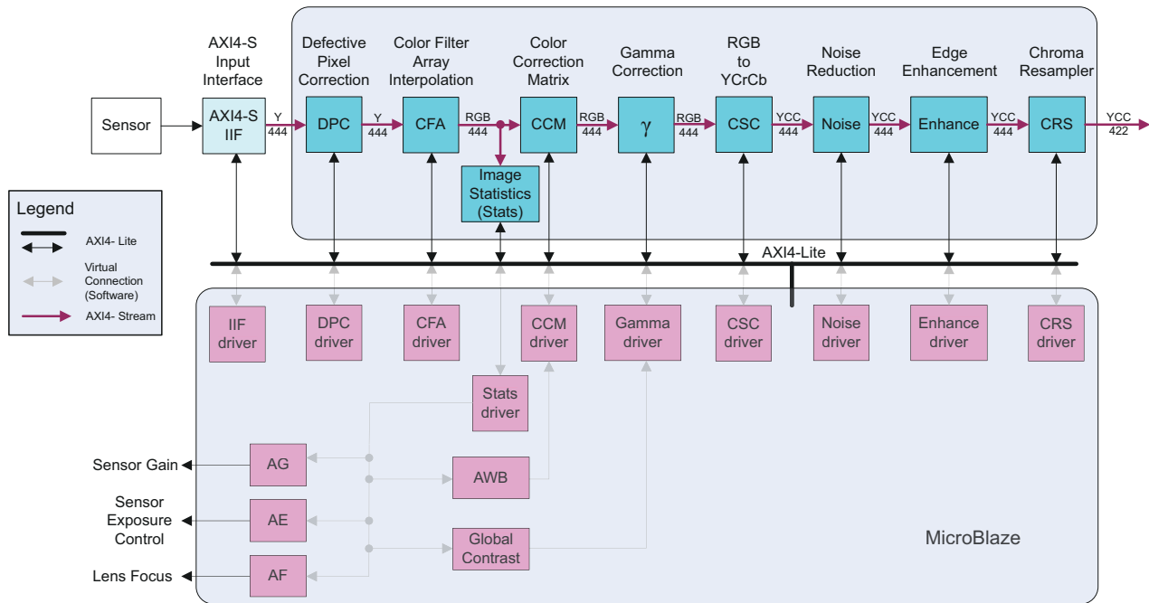
Figure 3-17: Image Processing Pipeline
