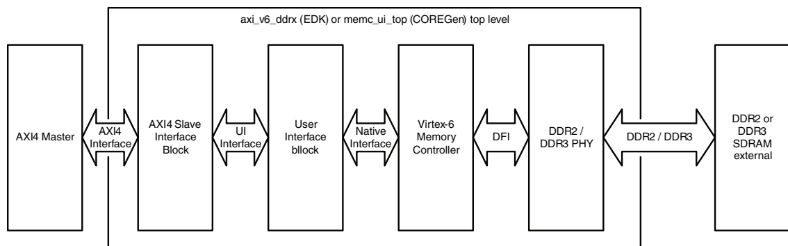
Figure 2-23: Virtex-6 Memory Control Block Diagram
