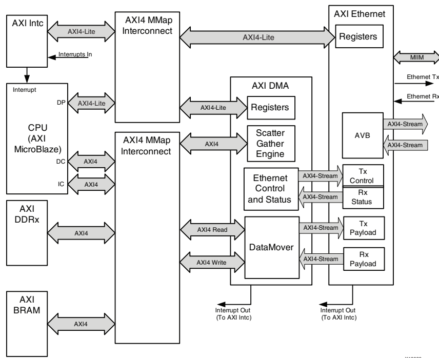
Figure 2-20: Typical Use Case for AXI DMA and AXI4 Ethernet
