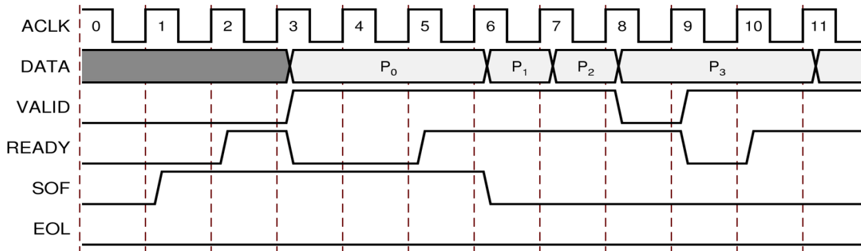
Figure 3-15: Example of Ready/Valid Handshake at Start of New Frame
