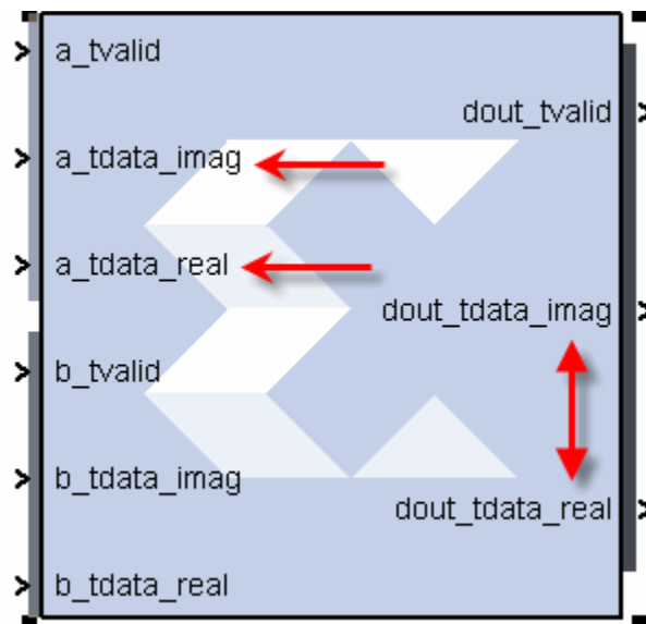
Figure 2-3: Multi-Channel TDATA
