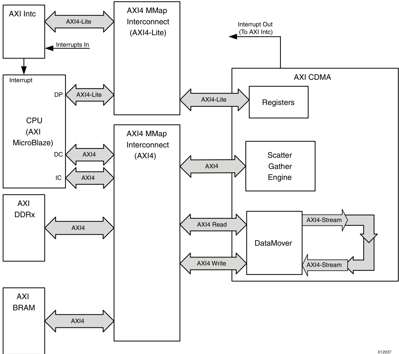
Figure 2-18: Typical Use Case for AXI Centralized DMA
