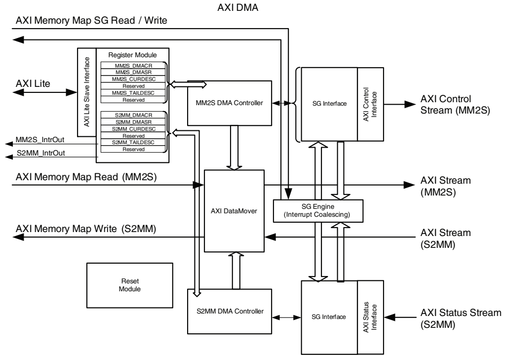
Figure 2-19: AXI DMA High Level Block Diagram
