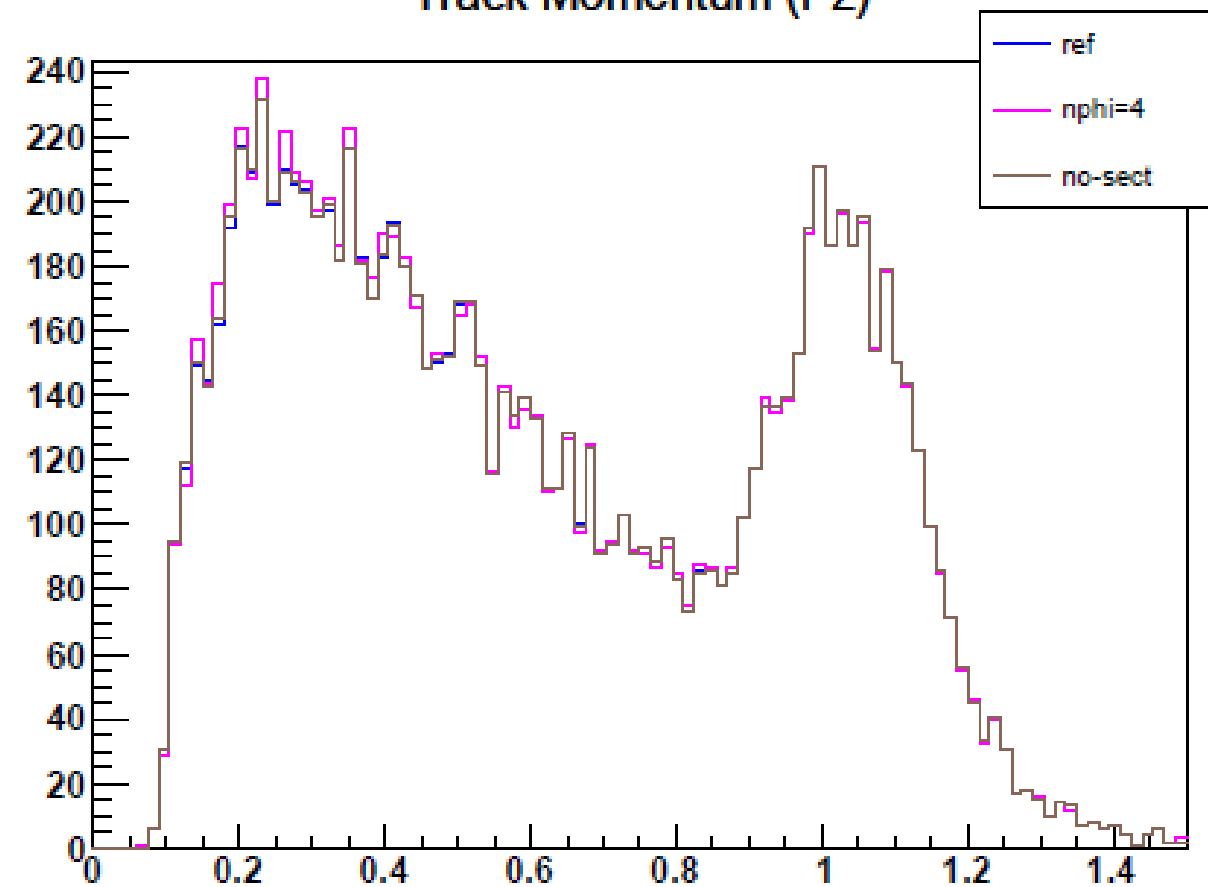
Track Momentum (Pz)
