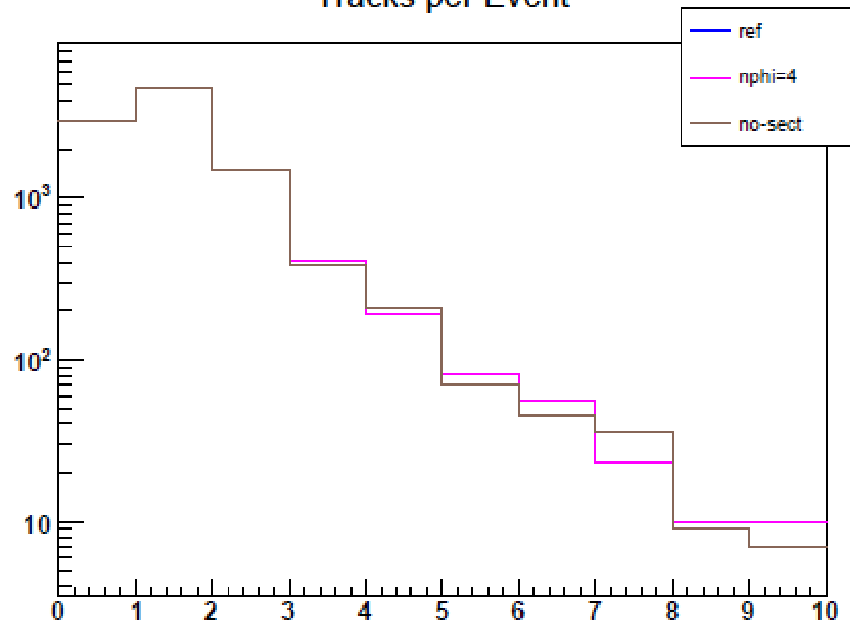
Tracks per Event
