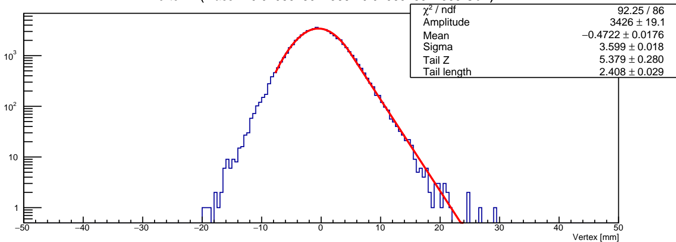
Vertex Z (mass in 0.0406578947368 - 0.0456578947368 GeV)
