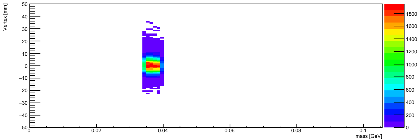
Vertex Z vs Mass (mass in 0.0343421052632 - 0.0393421052632 GeV)
