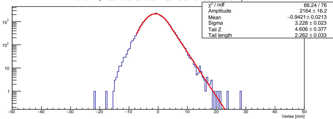
Vertex Z (mass in 0.0469736842105 - 0.0519736842105 GeV)
