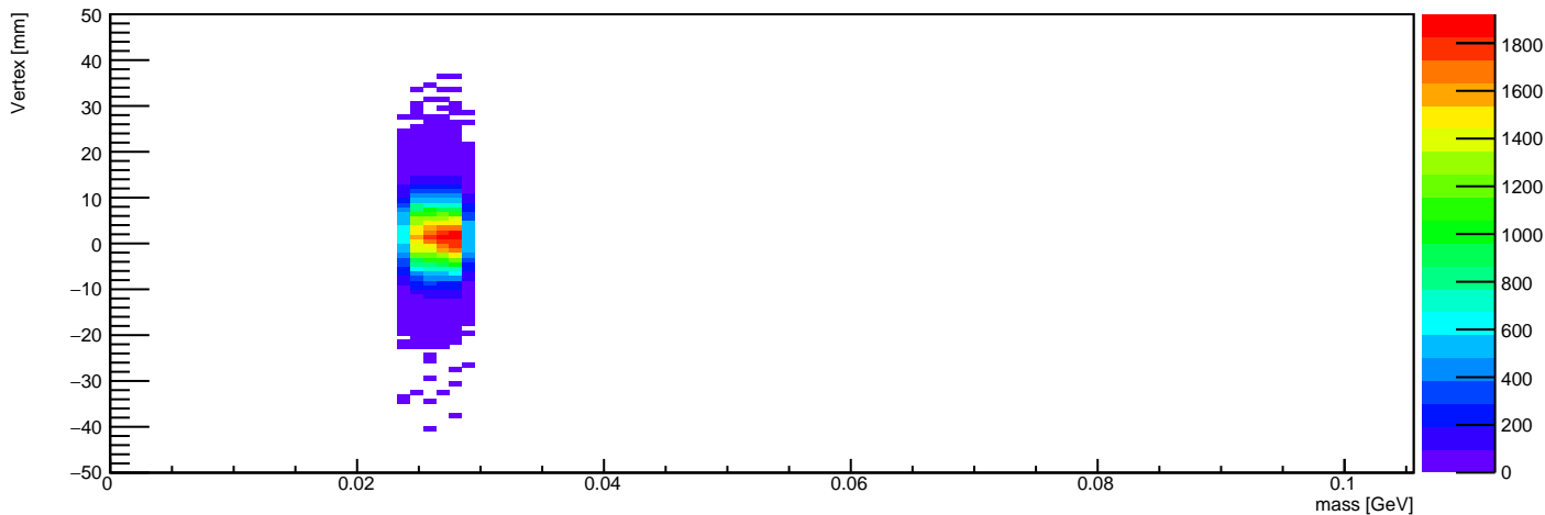
Vertex Z vs Mass (mass in 0.0238157894737 - 0.0288157894737 GeV)
