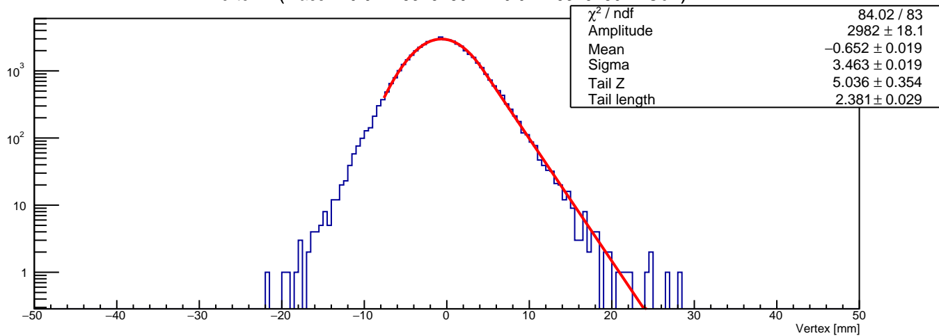
Vertex Z (mass in 0.0427631578947 - 0.0477631578947 GeV)
