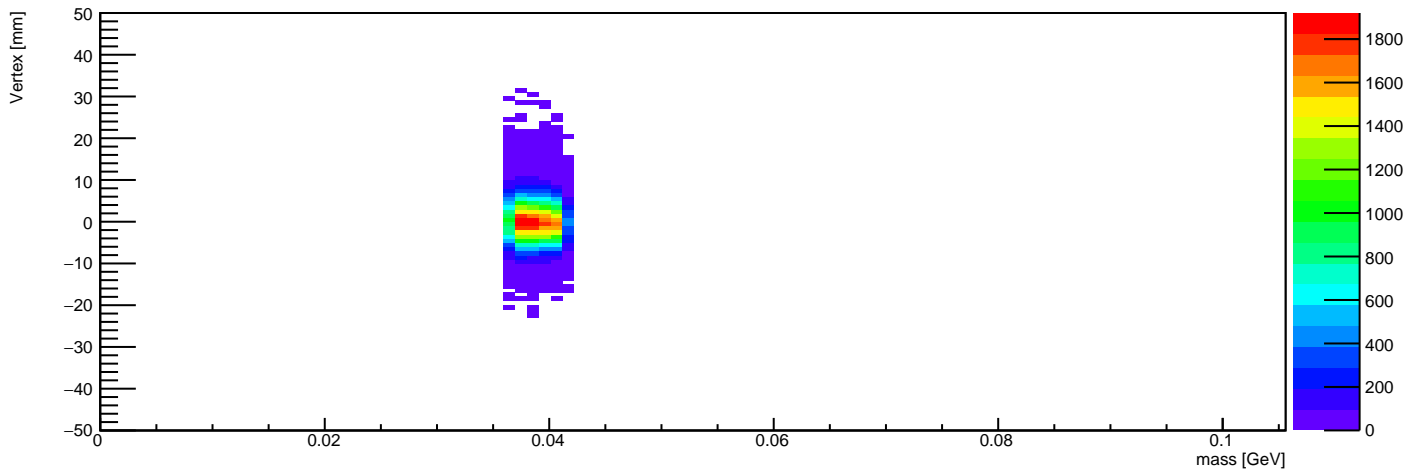
Vertex Z vs Mass (mass in 0.0364473684211 - 0.0414473684211 GeV)
