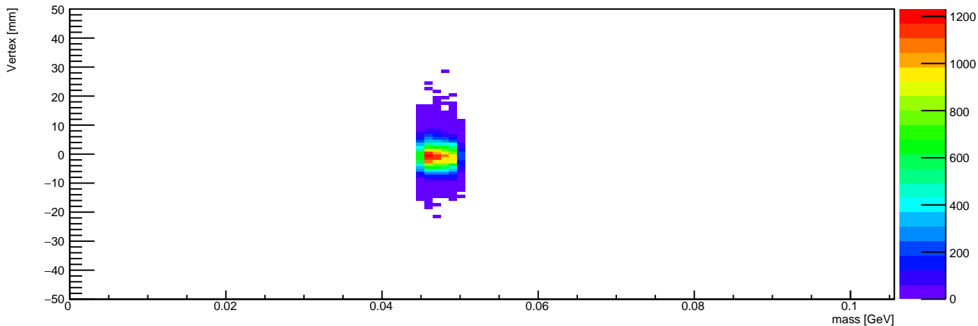
Vertex Z vs Mass (mass in 0.0448684210526 - 0.0498684210526 GeV)
