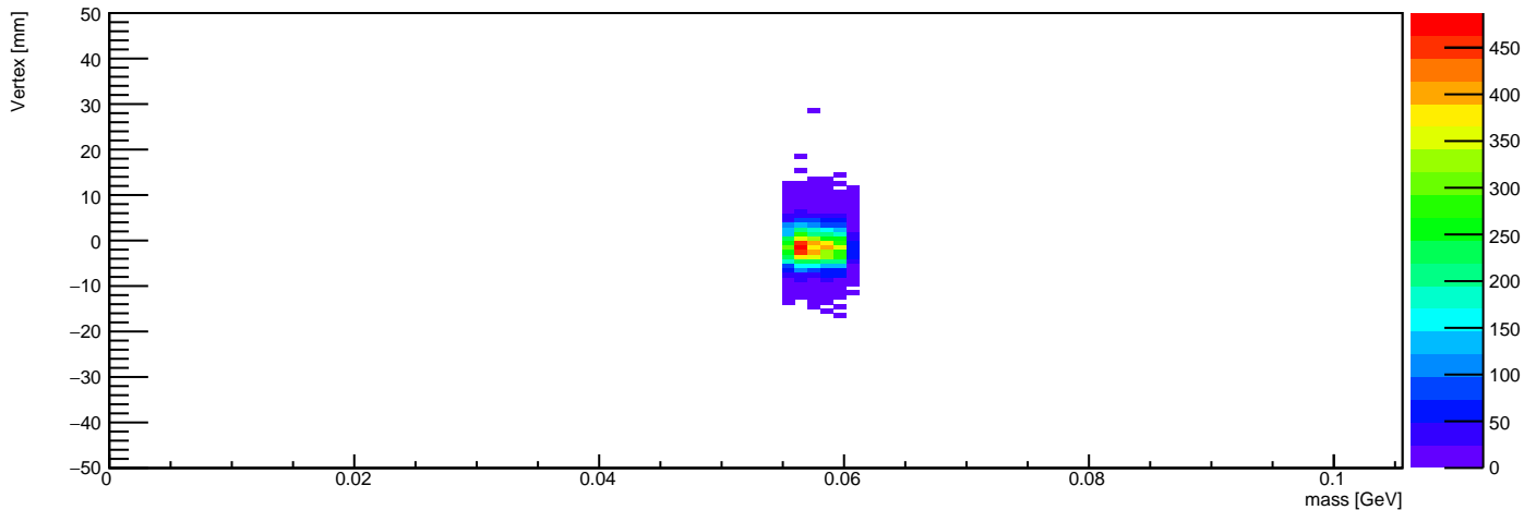
Vertex Z (mass in 0.0553947368421 - 0.0603947368421 GeV)
