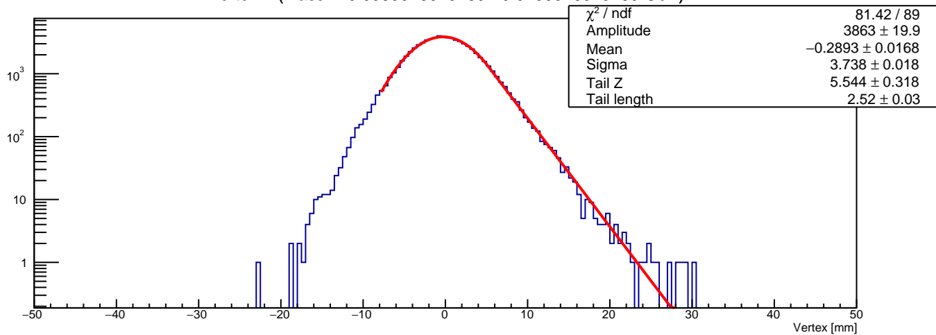
Vertex Z (mass in 0.0385526315789 - 0.0435526315789 GeV)
