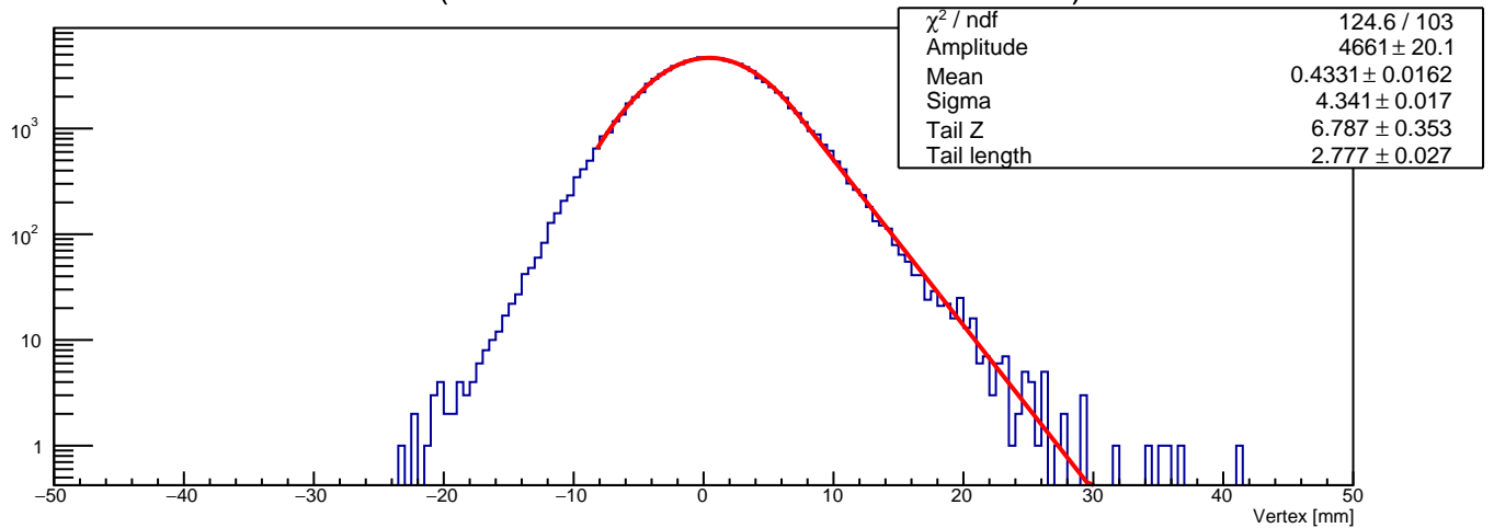
Vertex Z (mass in 0.0322368421053 - 0.0372368421053 GeV)
