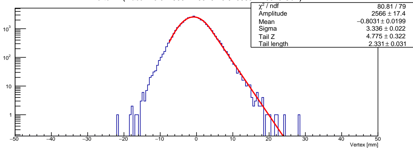
Vertex Z (mass in 0.0448684210526 - 0.0498684210526 GeV)
