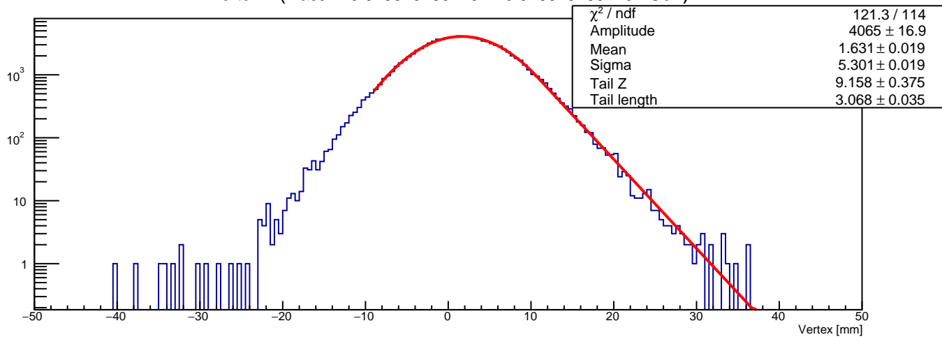
Vertex Z (mass in 0.0238157894737 - 0.0288157894737 GeV)
