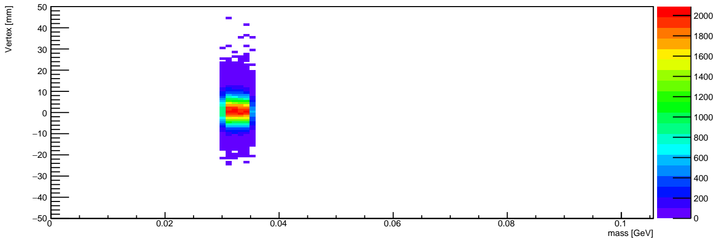
Vertex Z vs Mass (mass in 0.0301315789474 - 0.0351315789474 GeV)
