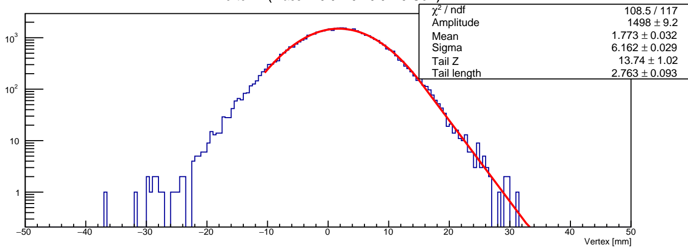
Vertex Z (mass in 0.0175 - 0.0225 GeV)
