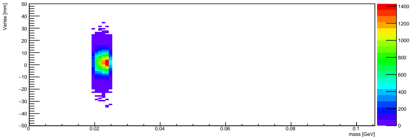
Vertex Z vs Mass (mass in 0.0196052631579 - 0.0246052631579 GeV)
