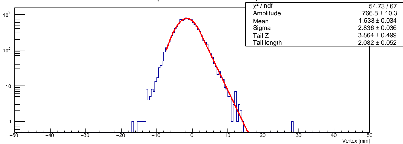
Vertex Z (mass in 0.0575 - 0.0625 GeV)
