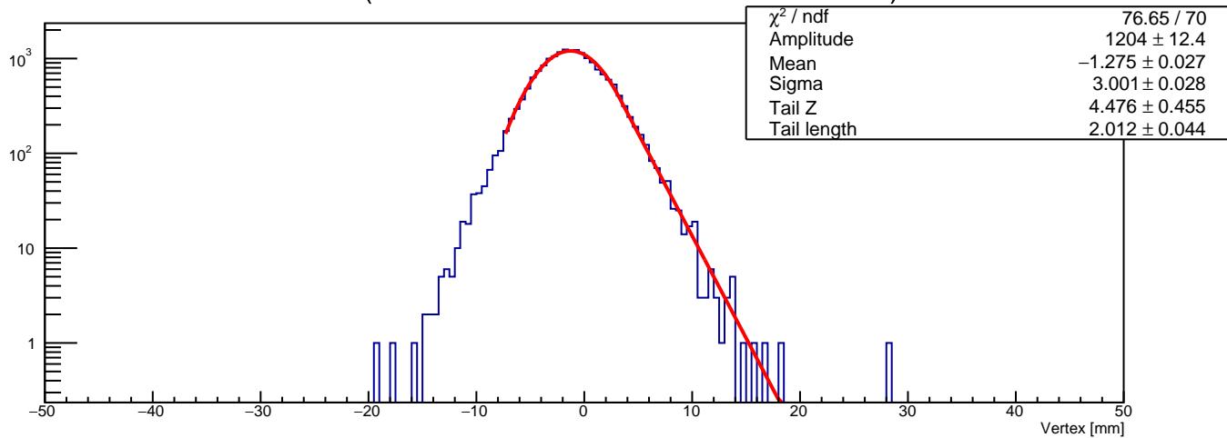
Vertex Z (mass in 0.0532894736842 - 0.0582894736842 GeV)
