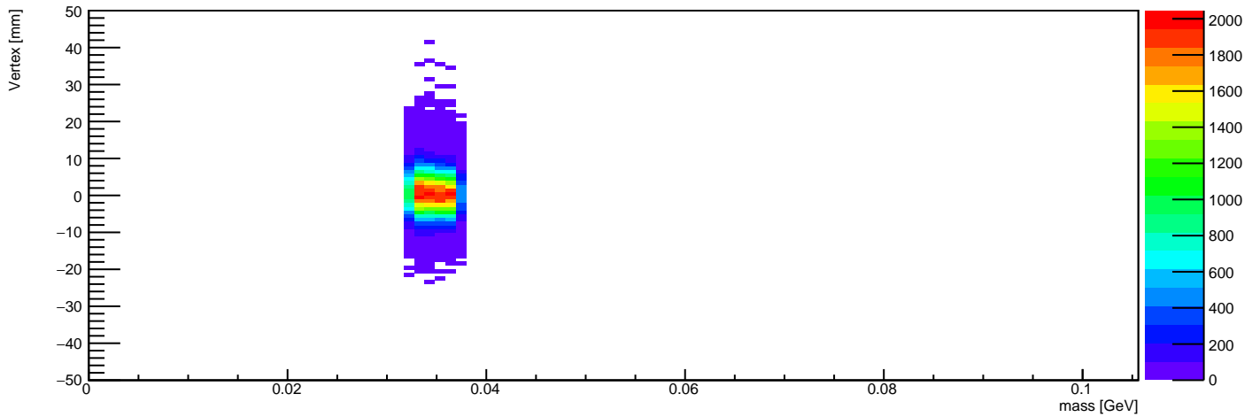
Vertex Z (mass in 0.0322368421053 - 0.0372368421053 GeV)
