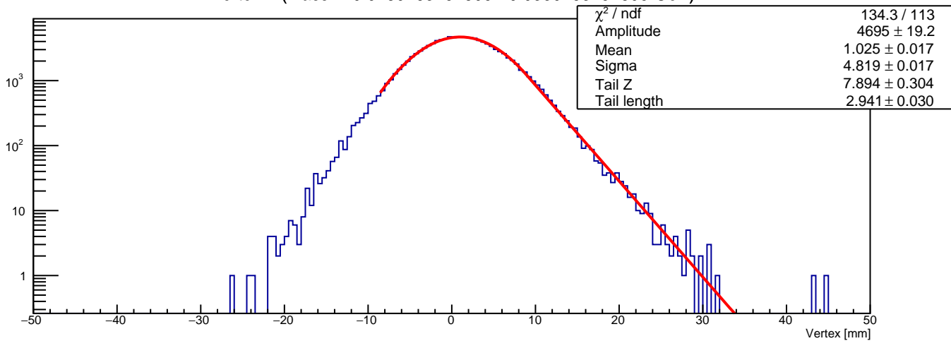
Vertex Z (mass in 0.0280263157895 - 0.0330263157895 GeV)
