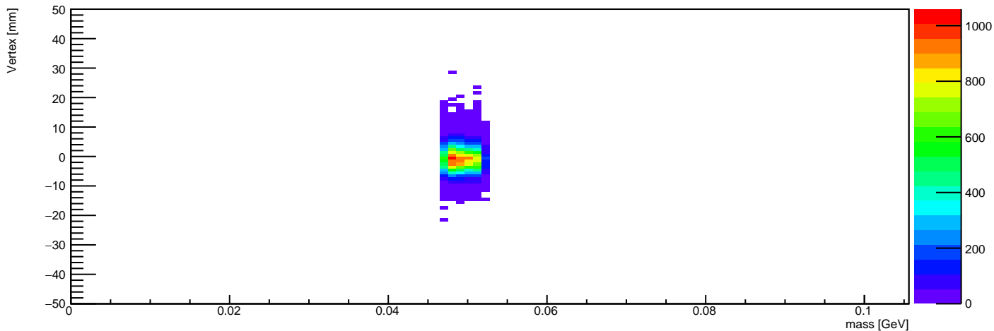
Vertex Z vs Mass (mass in 0.0469736842105 - 0.0519736842105 GeV)
