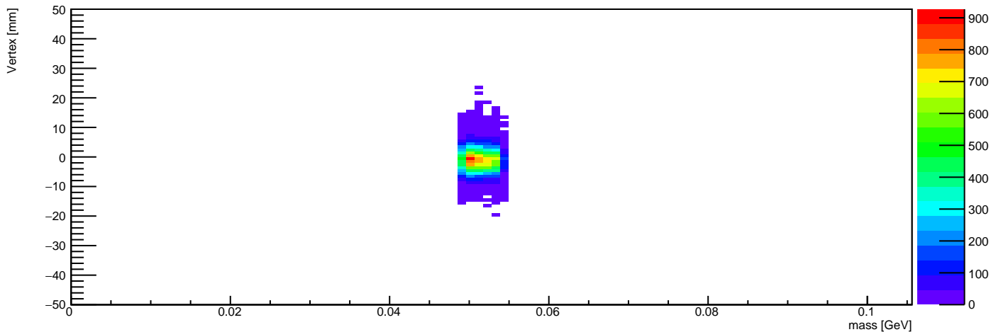
Vertex Z vs Mass (mass in 0.0490789473684 - 0.0540789473684 GeV)
