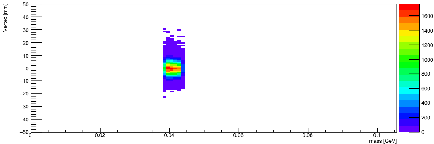
Vertex Z vs Mass (mass in 0.0385526315789 - 0.0435526315789 GeV)
