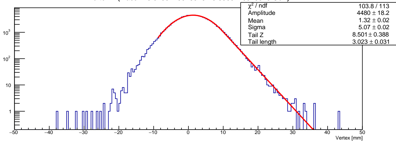
Vertex Z (mass in 0.0259210526316 - 0.0309210526316 GeV)
