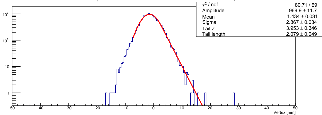
Vertex Z (mass in 0.0553947368421 - 0.0603947368421 GeV)
