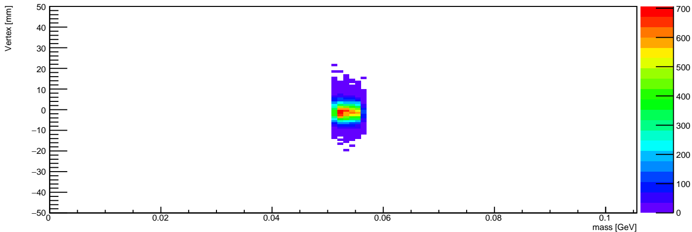
Vertex Z vs Mass (mass in 0.0511842105263 - 0.0561842105263 GeV)
