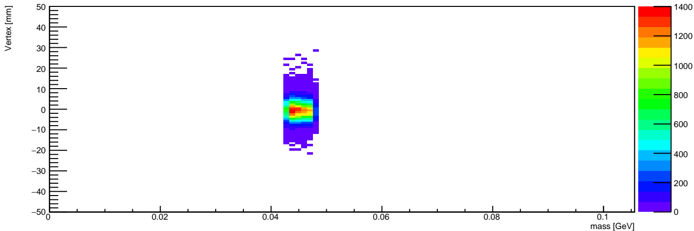
Vertex Z vs Mass (mass in 0.0427631578947 - 0.0477631578947 GeV)
