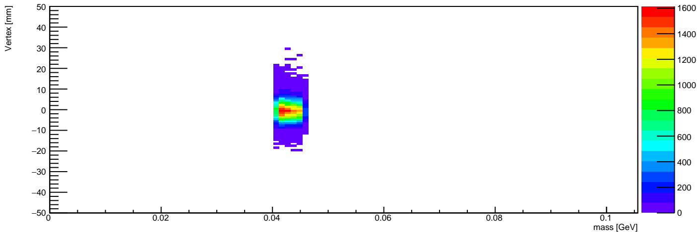
Vertex Z vs Mass (mass in 0.0406578947368 - 0.0456578947368 GeV)
