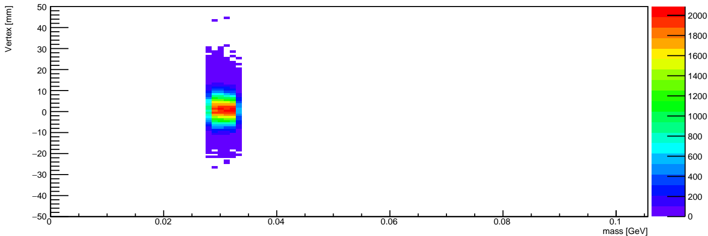
Vertex Z vs Mass (mass in 0.0280263157895 - 0.0330263157895 GeV)
