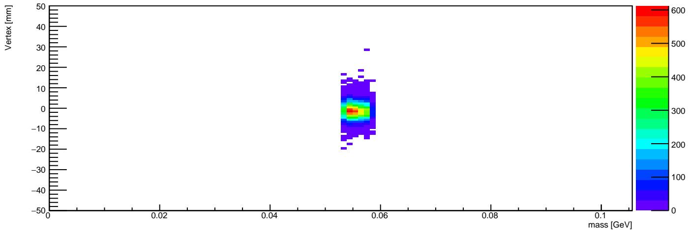
Vertex Z vs Mass (mass in 0.0532894736842 - 0.0582894736842 GeV)
