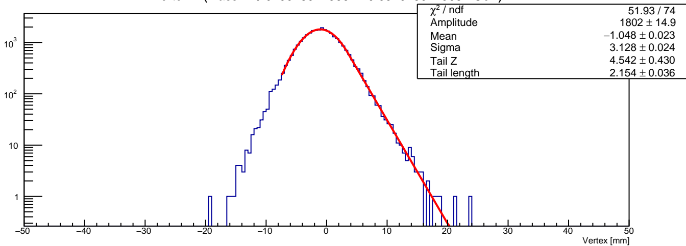
Vertex Z (mass in 0.0490789473684 - 0.0540789473684 GeV)
