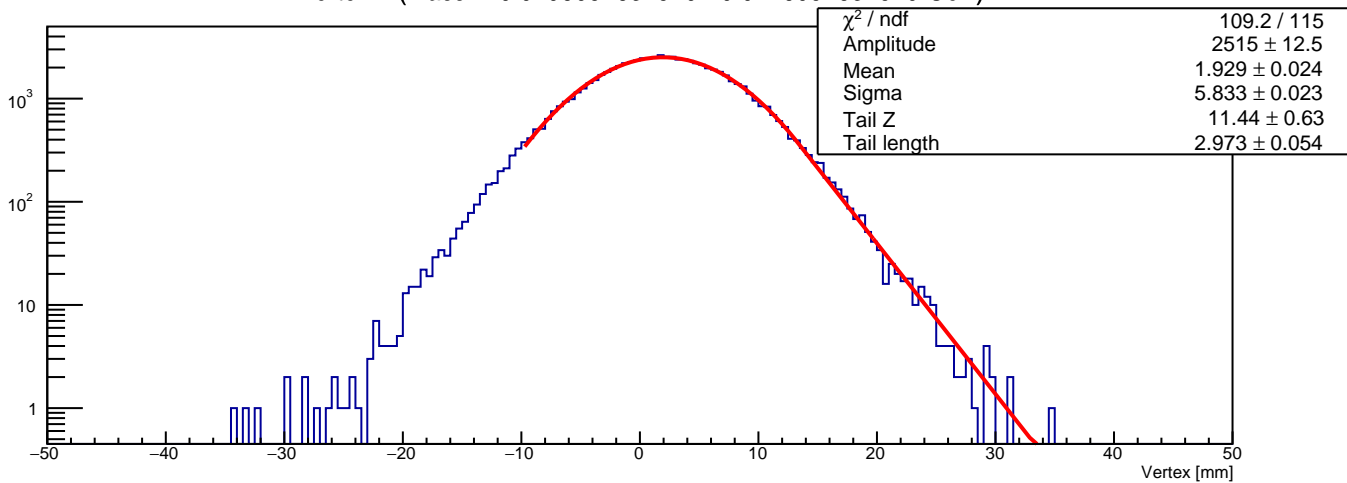
Vertex Z (mass in 0.0196052631579 - 0.0246052631579 GeV)
