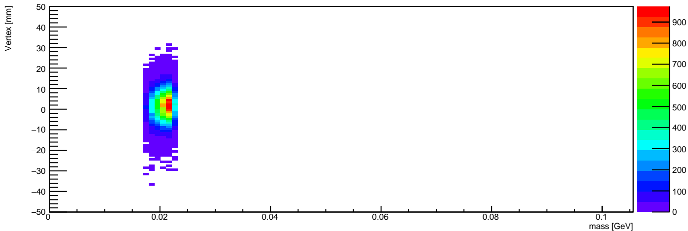
Vertex Z vs Mass (mass in 0.0175 - 0.0225 GeV)
