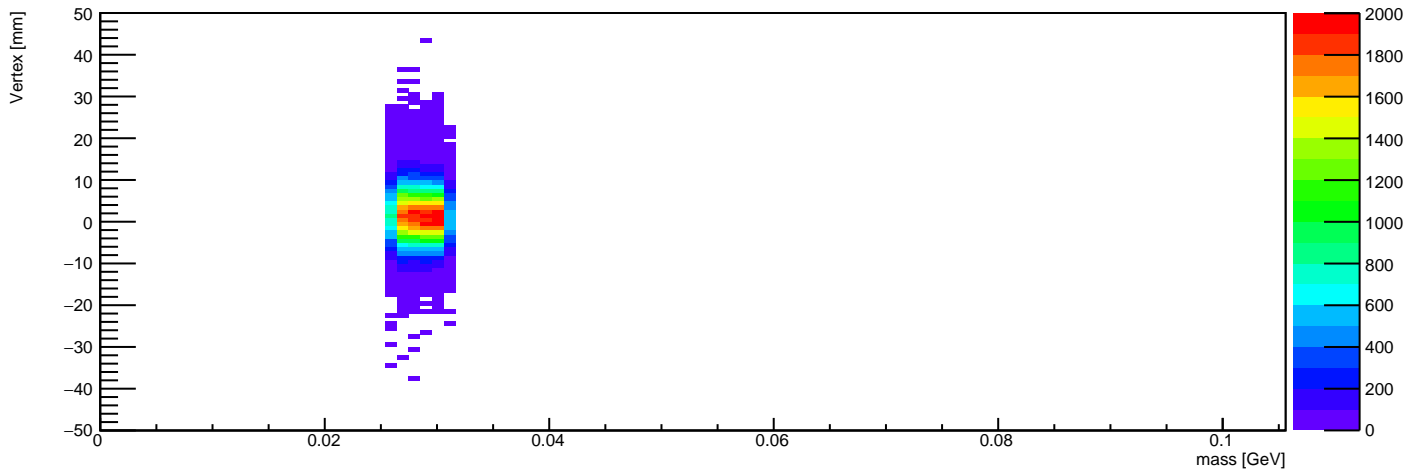
Vertex Z vs Mass (mass in 0.0259210526316 - 0.0309210526316 GeV)
