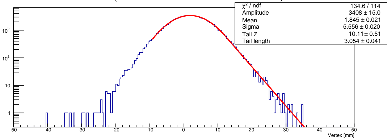
Vertex Z (mass in 0.0217105263158 - 0.0267105263158 GeV)
