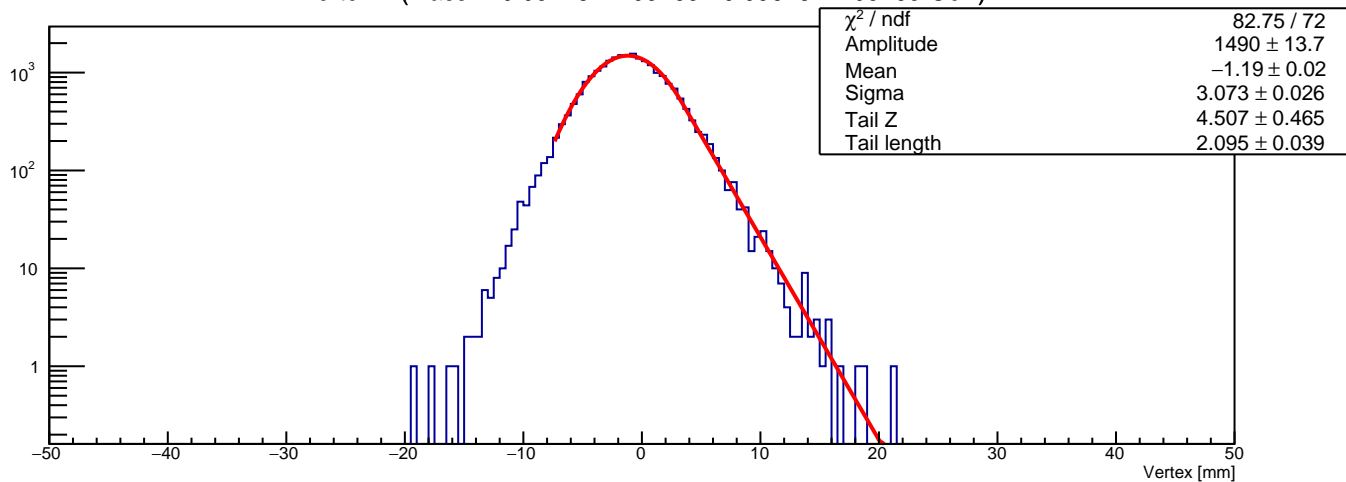
Vertex Z (mass in 0.0511842105263 - 0.0561842105263 GeV)
