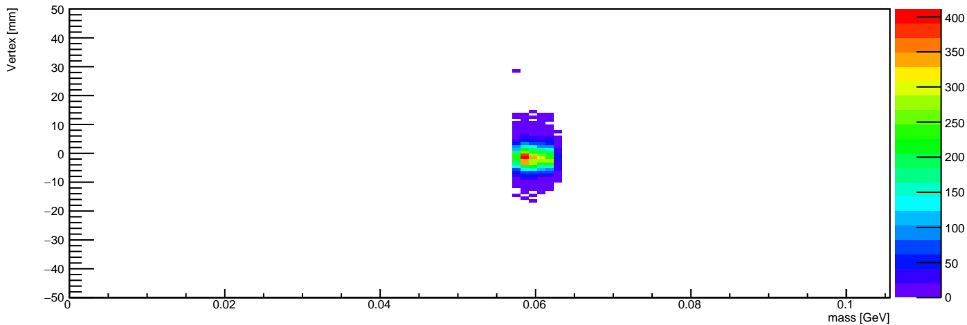
Vertex Z vs Mass (mass in 0.0575 - 0.0625 GeV)
