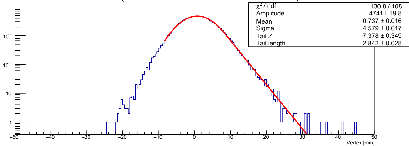
Vertex Z (mass in 0.0301315789474 - 0.0351315789474 GeV)
