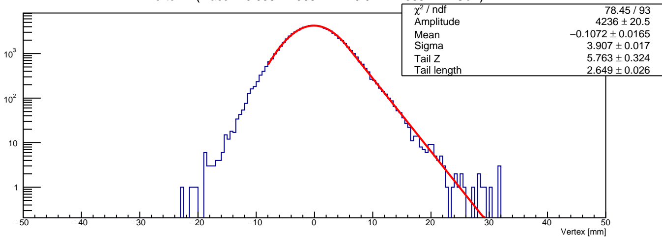
Vertex Z (mass in 0.0364473684211 - 0.0414473684211 GeV)
