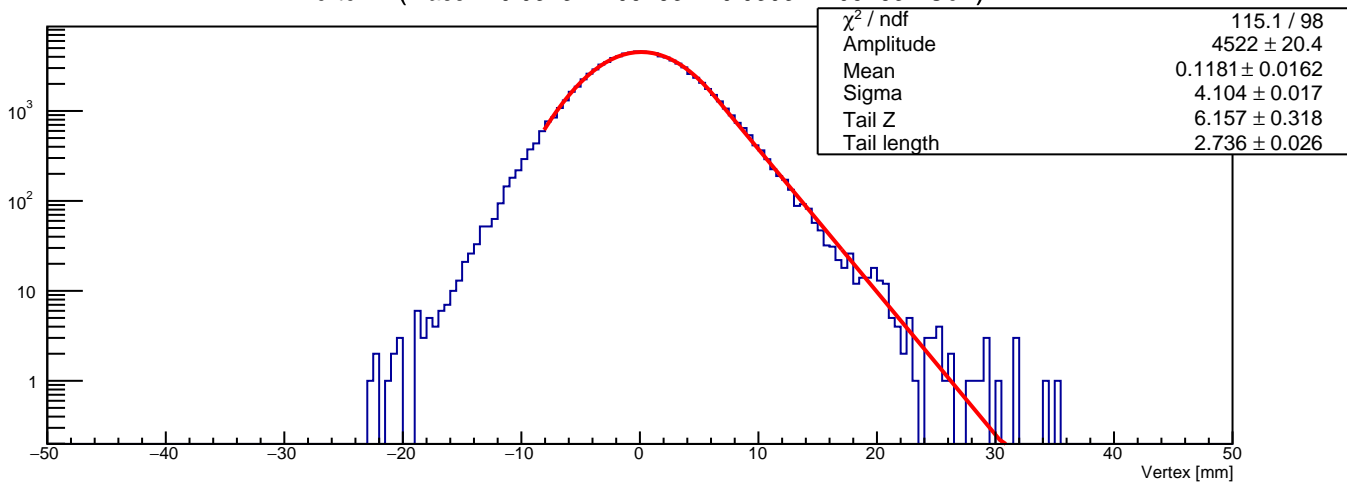
Vertex Z (mass in 0.0343421052632 - 0.0393421052632 GeV)
