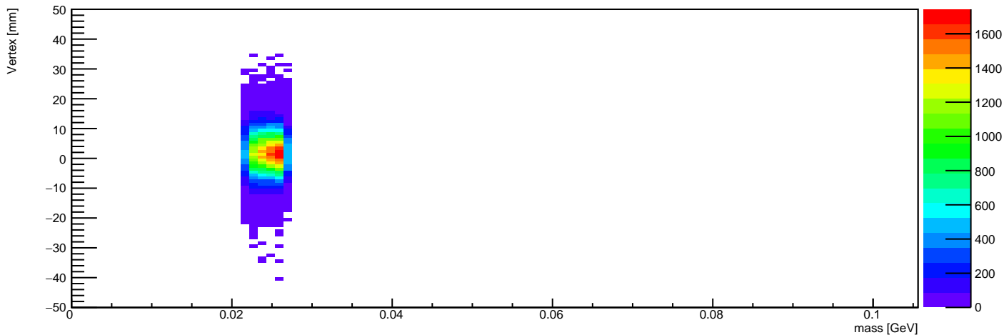
Vertex Z vs Mass (mass in 0.0217105263158 - 0.0267105263158 GeV)
