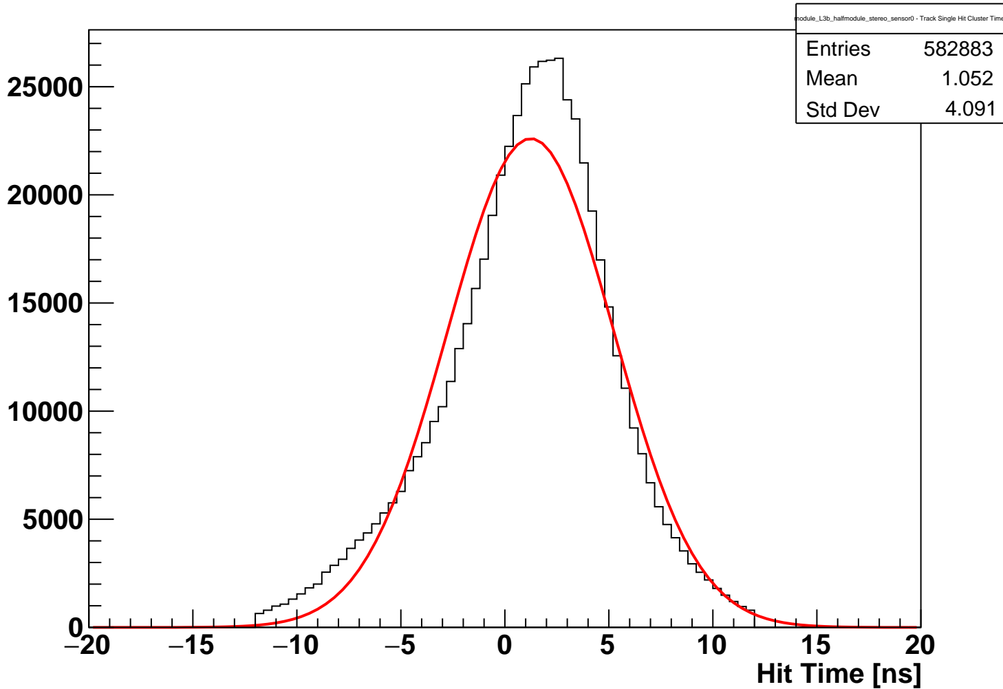
module_L3b_halfmodule_stereo_sensor0 Fitted Hit Time (hits on clean track)
