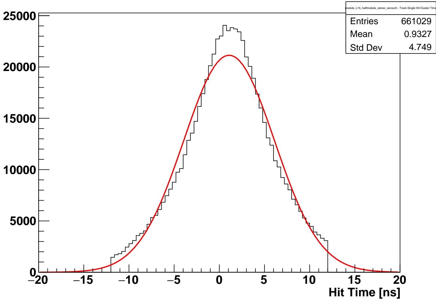
module_L1b_halfmodule_stereo_sensor0 Fitted Hit Time (hits on clean track)
