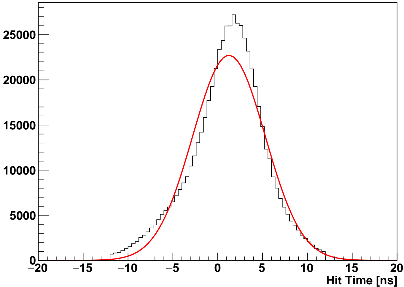
module_L3b_halfmodule_axial_sensor0 Fitted Hit Time (hits on clean track)
