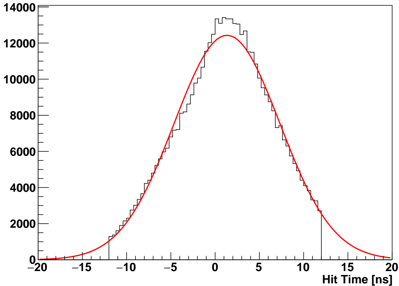
module_L1t_halfmodule_axial_sensor0 Fitted Hit Time (hits on clean track)
