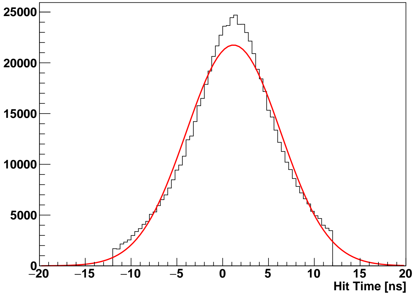
module_L1b_halfmodule_axial_sensor0 Fitted Hit Time (hits on clean track)
