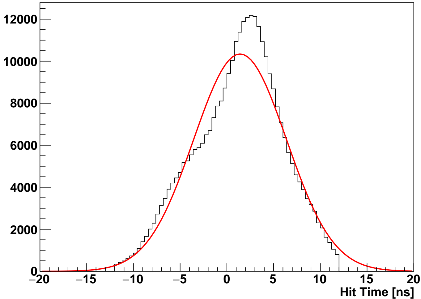
module_L6t_halfmodule_axial_hole_sensor0 Fitted Hit Time (hits on clean track)
