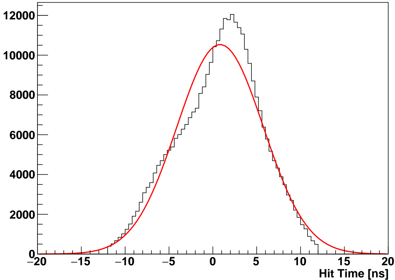
module_L4t_halfmodule_stereo_hole_sensor0 Fitted Hit Time (hits on clean track)
