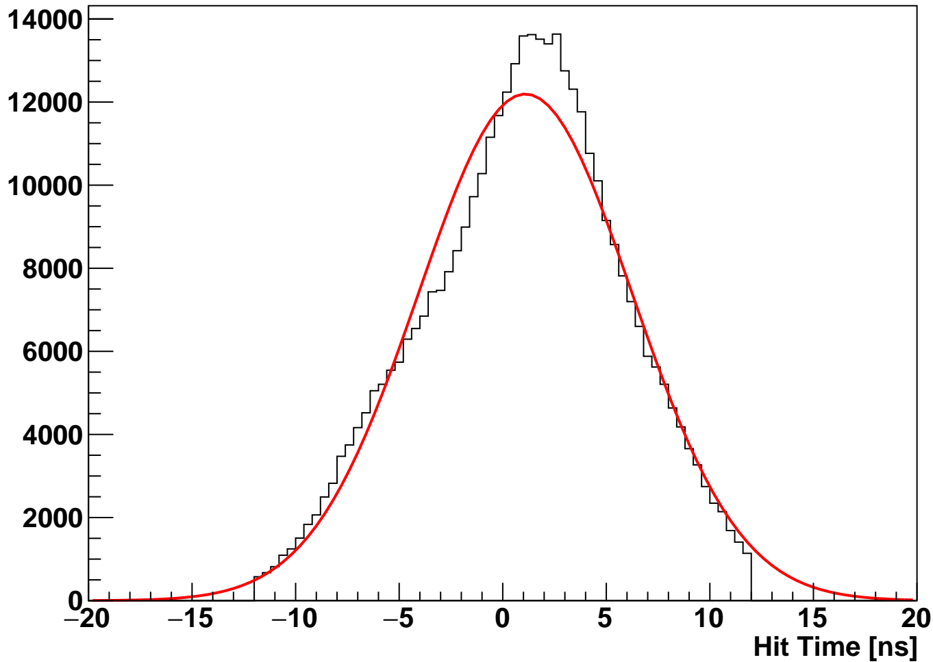
module_L2t_halfmodule_axial_sensor0 Fitted Hit Time (hits on clean track)
