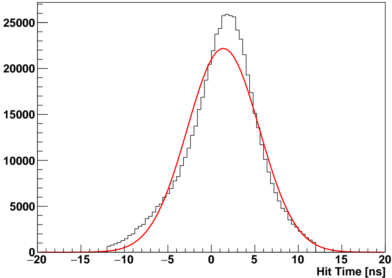
module_L2b_halfmodule_stereo_sensor0 Fitted Hit Time (hits on clean track)
