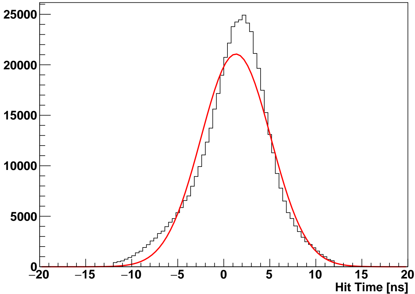
module_L4b_halfmodule_axial_hole_sensor0 Fitted Hit Time (hits on clean track)
