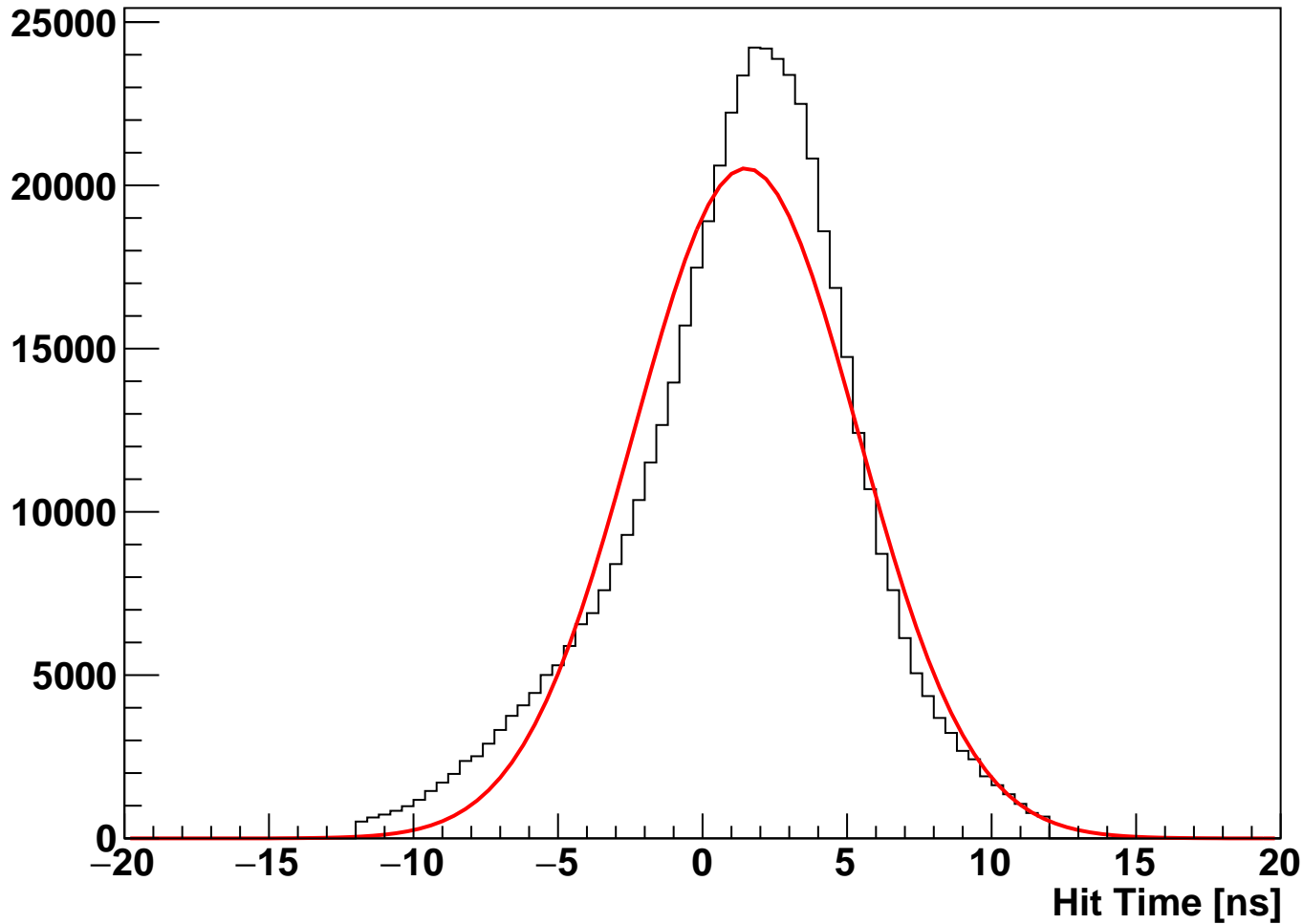
module_L6b_halfmodule_stereo_hole_sensor0 Fitted Hit Time (hits on clean track)
