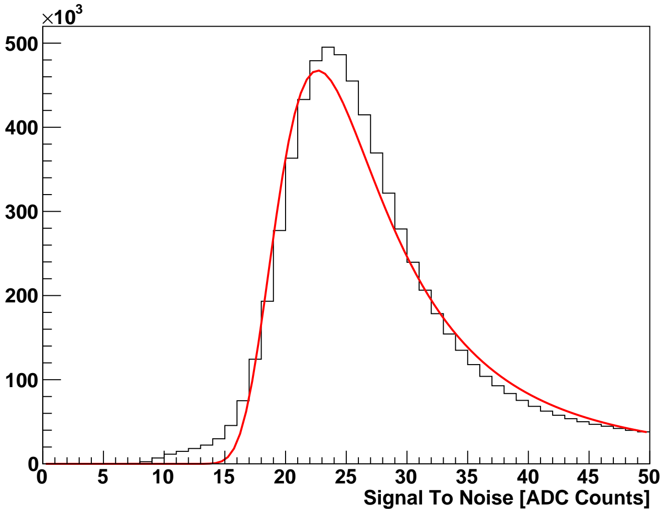
module_L6b_halfmodule_axial_hole_sensor0 Fitted Signal To Noise (hits on clean track)
