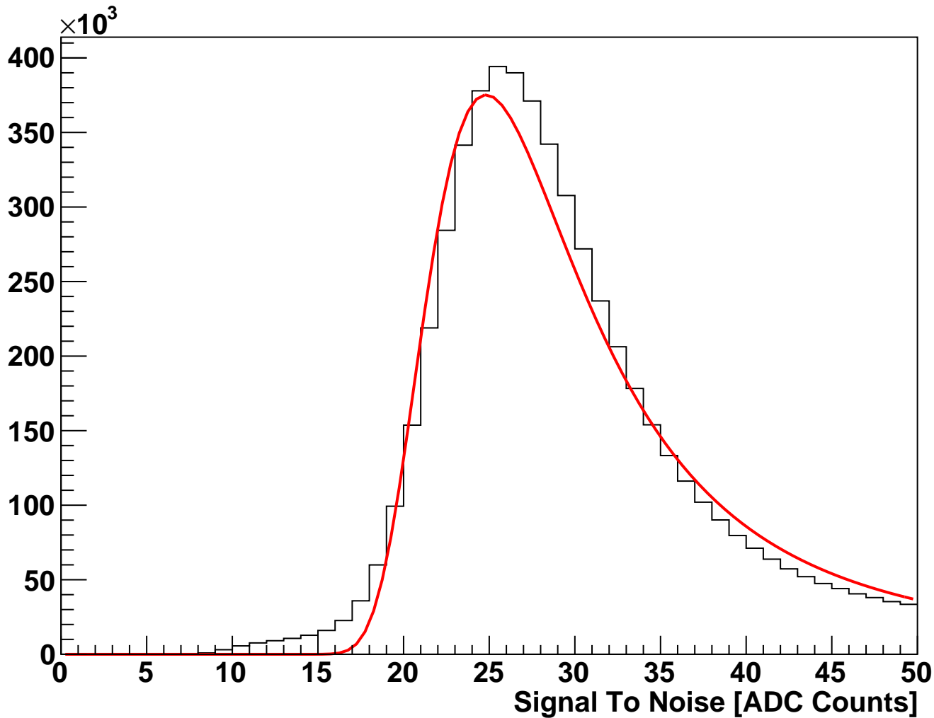
module_L6t_halfmodule_axial_hole_sensor0 Fitted Signal To Noise (hits on clean track)
