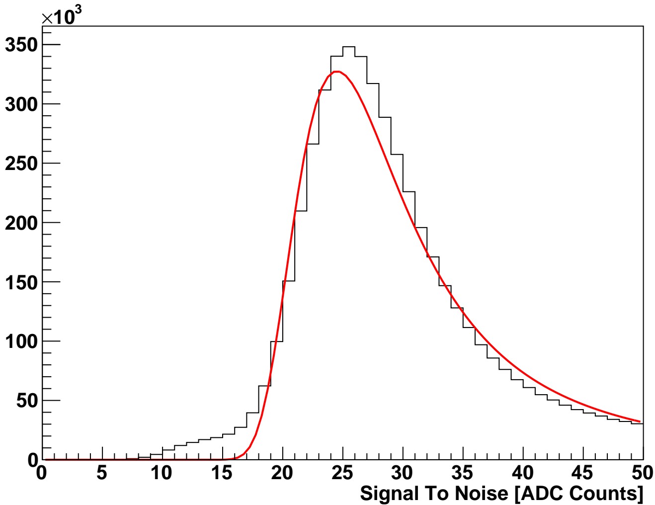
module_L6t_halfmodule_stereo_hole_sensor0 Fitted Signal To Noise (hits on clean track)
