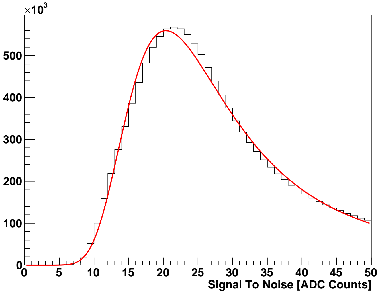
module_L1b_halfmodule_axial_sensor0 Fitted Signal To Noise (hits on clean track)
