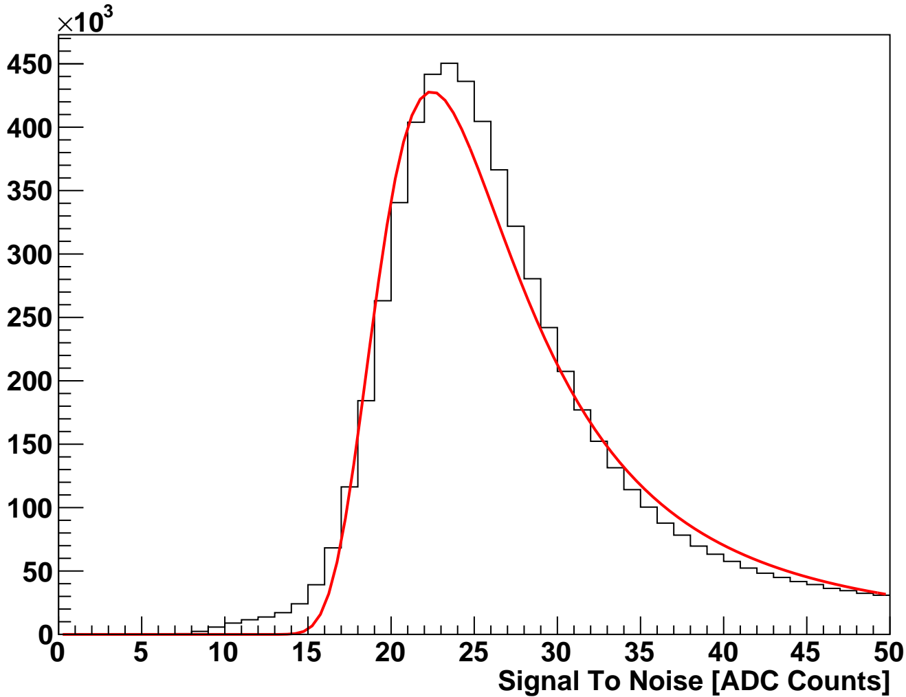
module_L5t_halfmodule_axial_hole_sensor0 Fitted Signal To Noise (hits on clean track)
