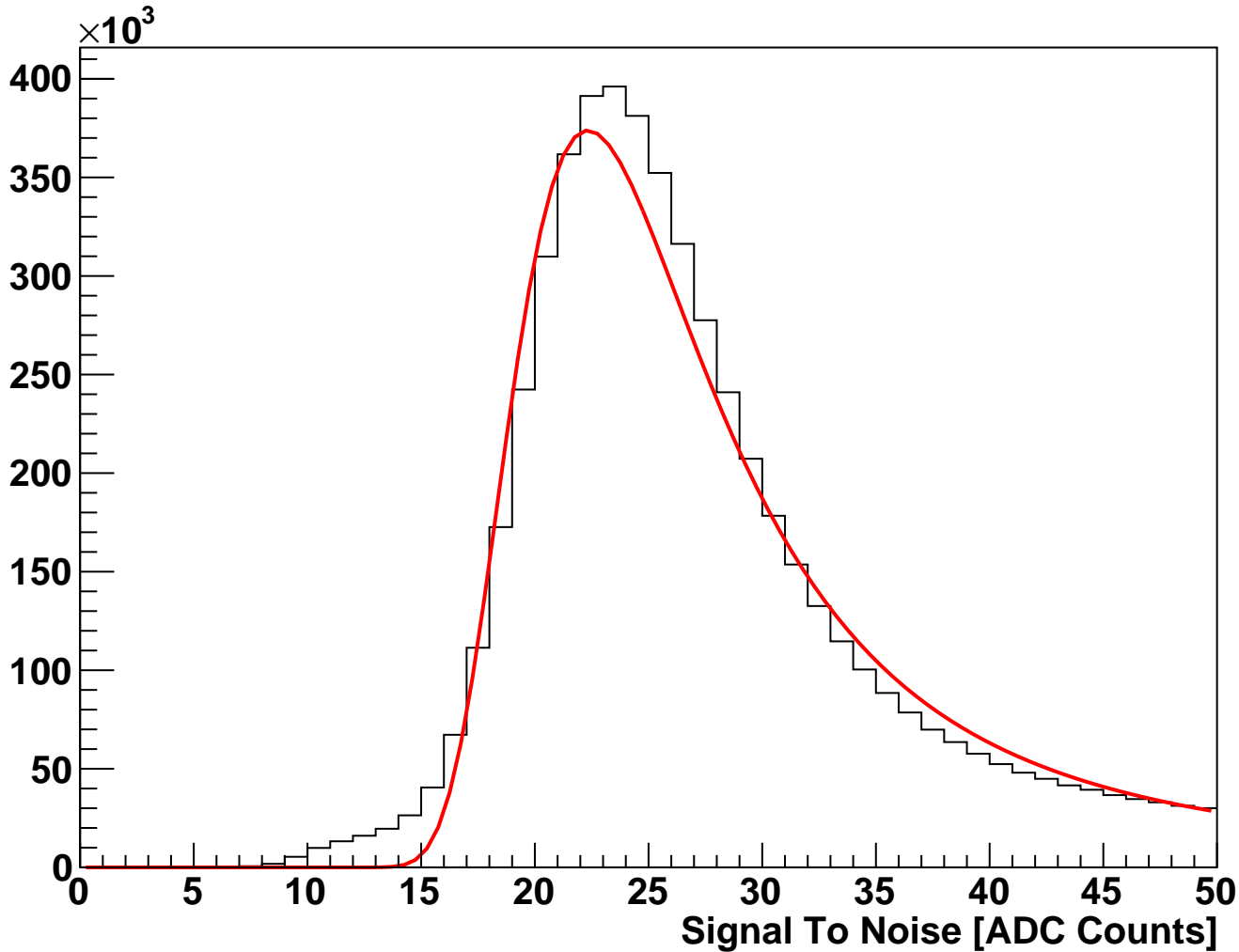
module_L5t_halfmodule_stereo_hole_sensor0 Fitted Signal To Noise (hits on clean track)
