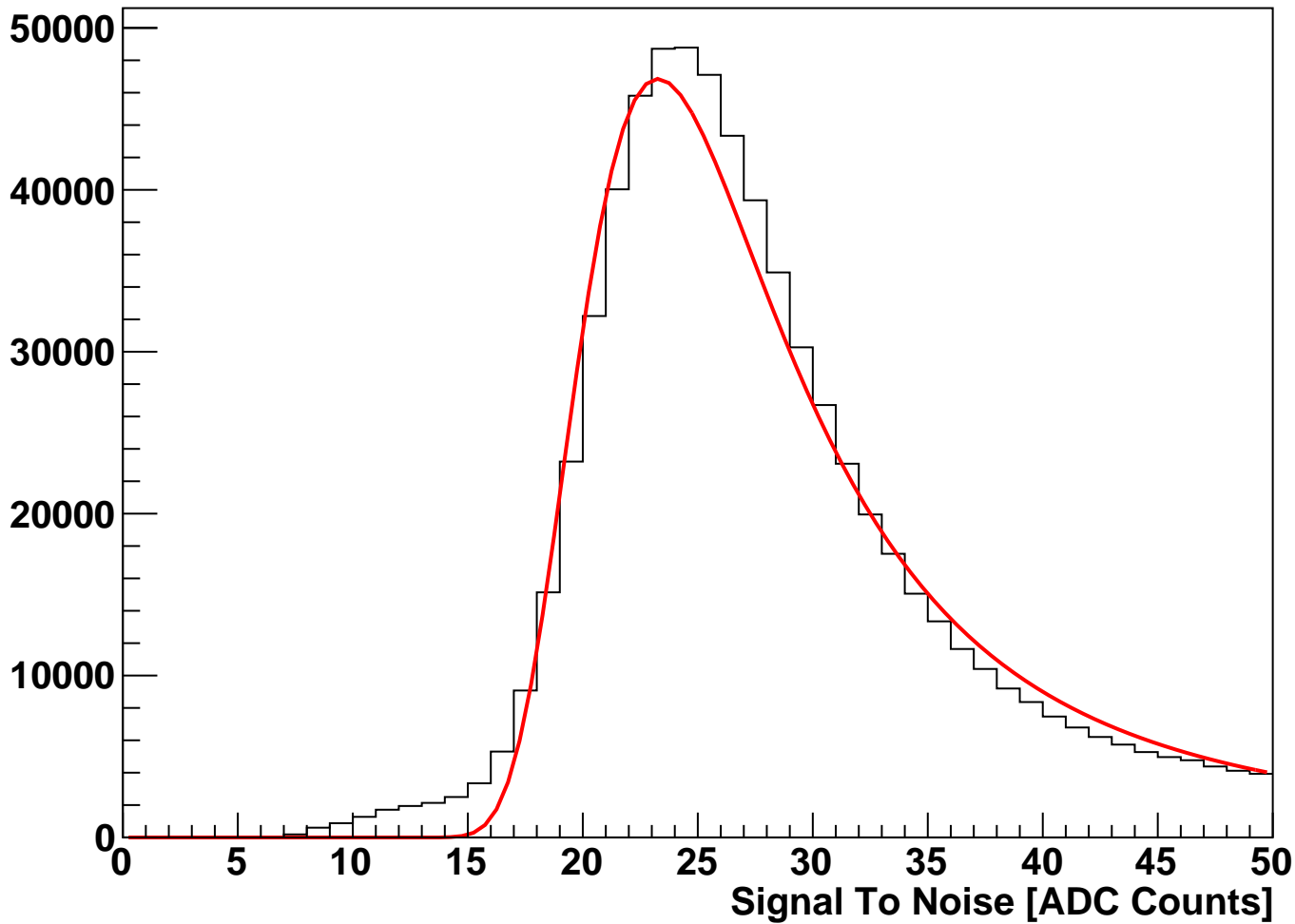
module_L6t_halfmodule_axial_slot_sensor0 Fitted Signal To Noise (hits on clean track)
