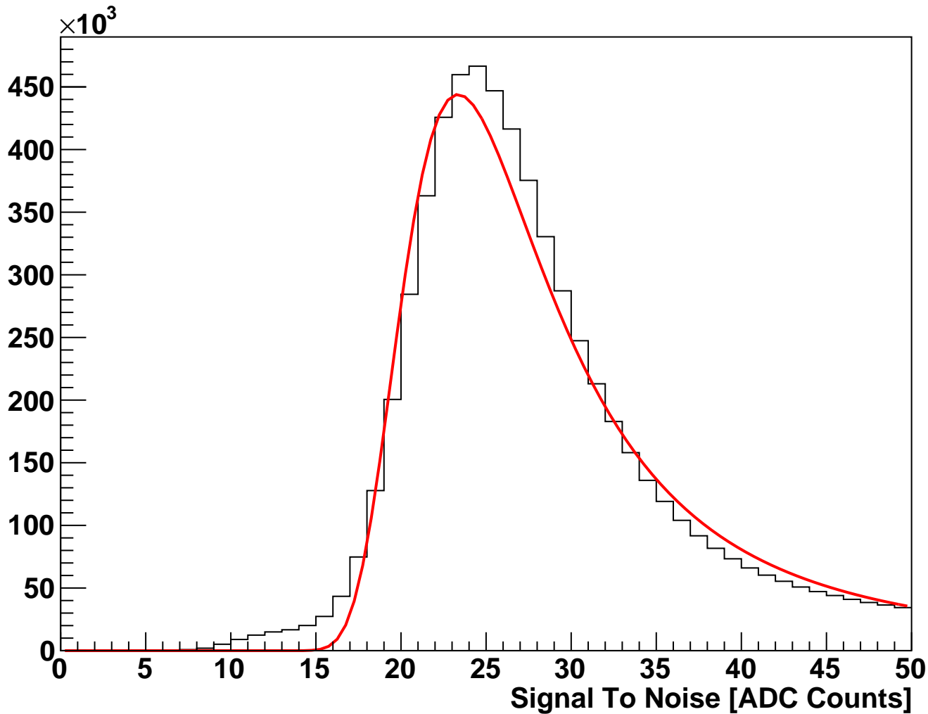
module_L5b_halfmodule_stereo_hole_sensor0 Fitted Signal To Noise (hits on clean track)
