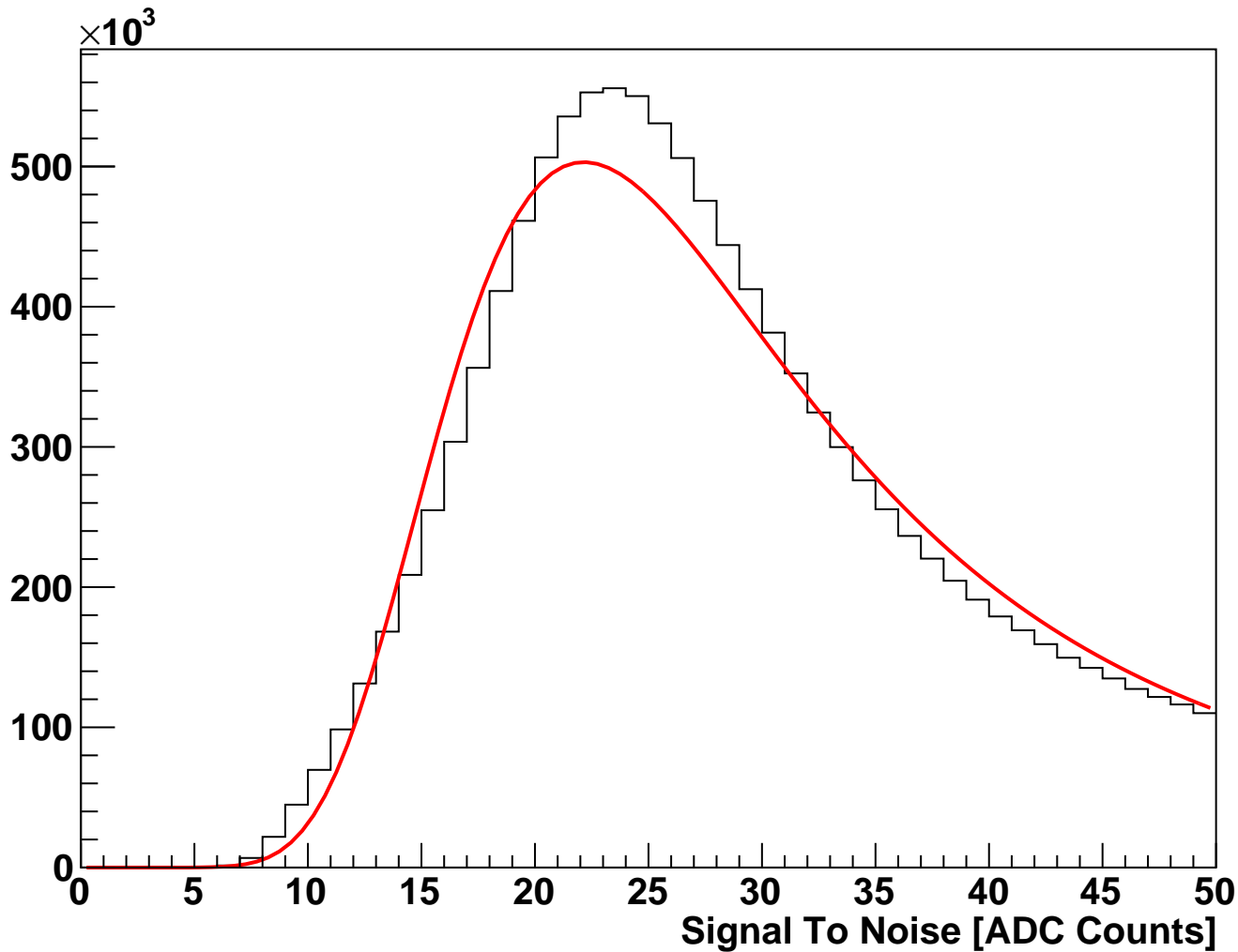
module_L1b_halfmodule_stereo_sensor0 Fitted Signal To Noise (hits on clean track)
