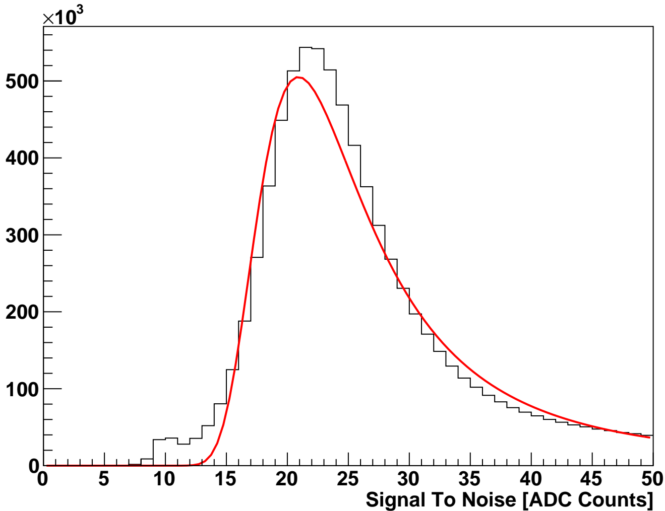
module_L3b_halfmodule_stereo_sensor0 Fitted Signal To Noise (hits on clean track)
