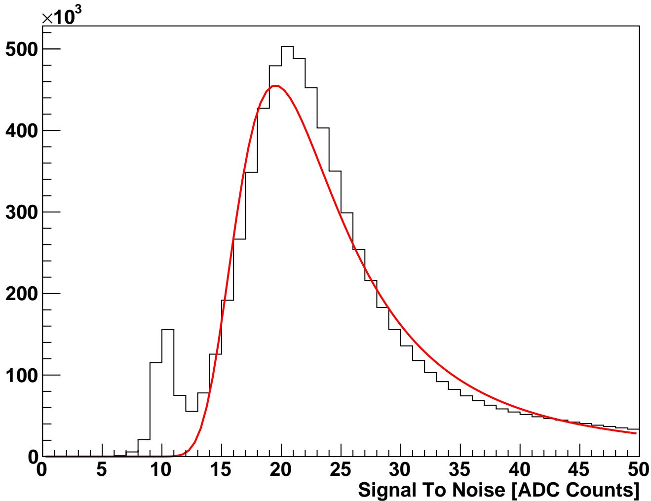
module_L3t_halfmodule_stereo_sensor0 Fitted Signal To Noise (hits on clean track)
