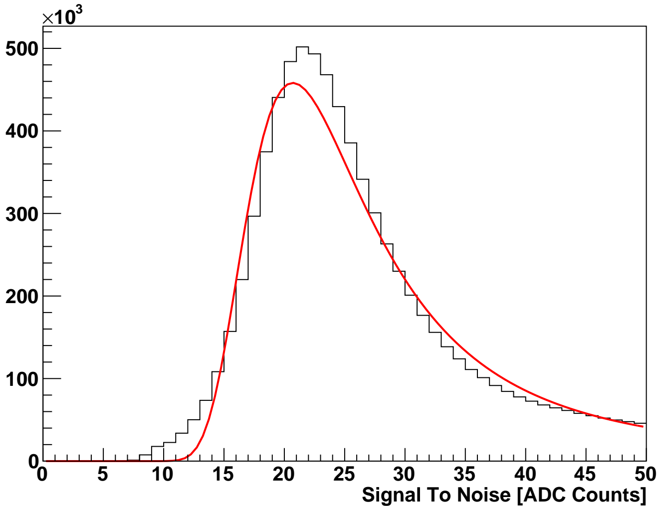
module_L2t_halfmodule_stereo_sensor0 Fitted Signal To Noise (hits on clean track)
