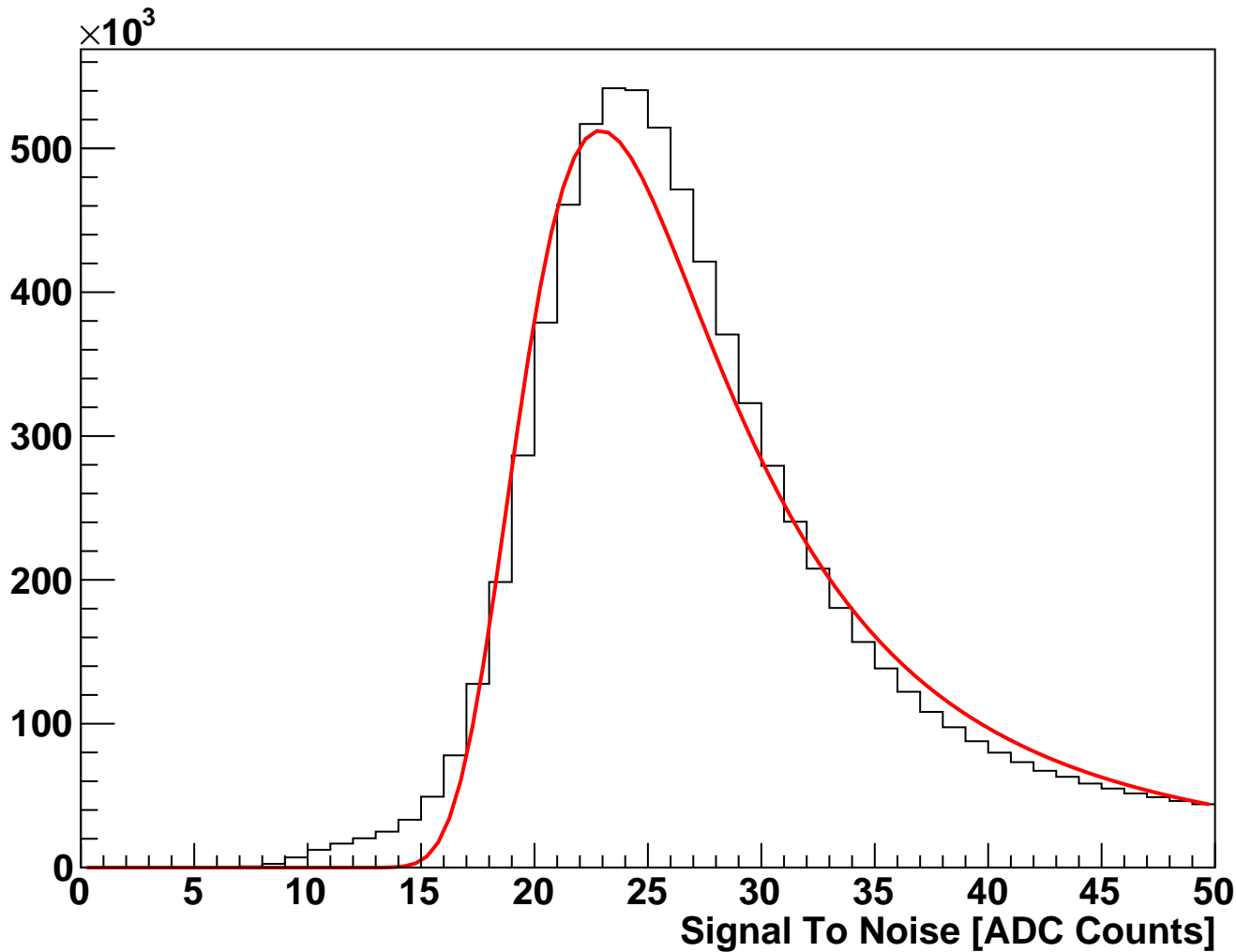
module_L5b_halfmodule_axial_hole_sensor0 Fitted Signal To Noise (hits on clean track)
