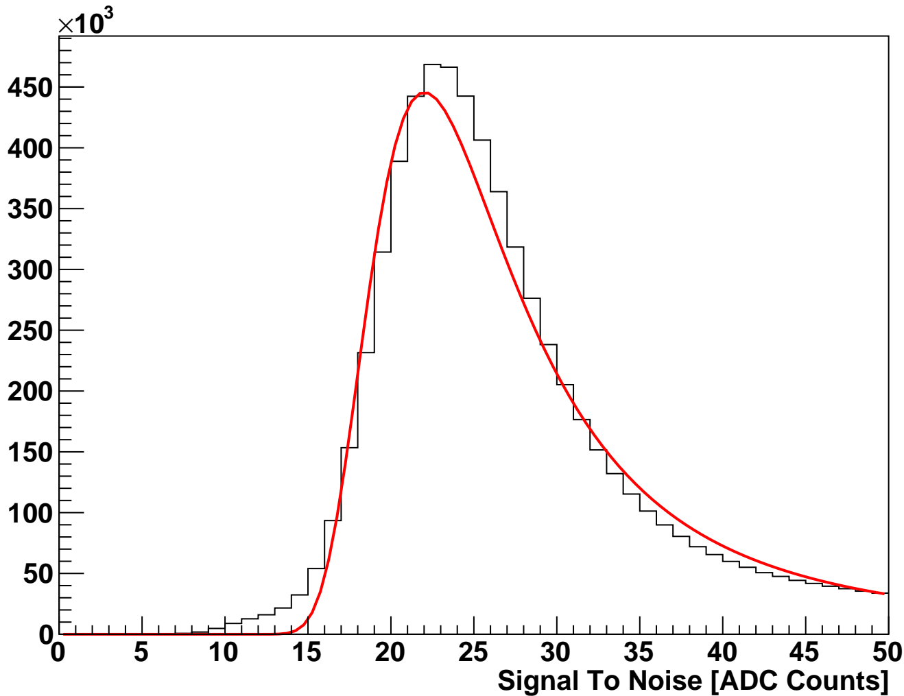
module_L4b_halfmodule_stereo_hole_sensor0 Fitted Signal To Noise (hits on clean track)
