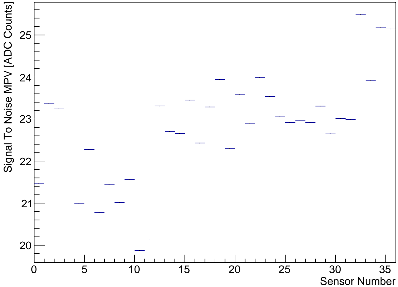
Fitted Signal To Noise MPV (hits on clean track)
