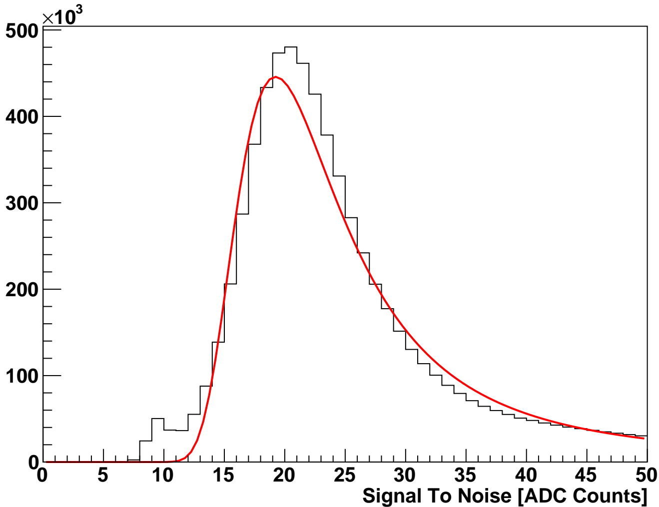
module_L3t_halfmodule_axial_sensor0 Fitted Signal To Noise (hits on clean track)
