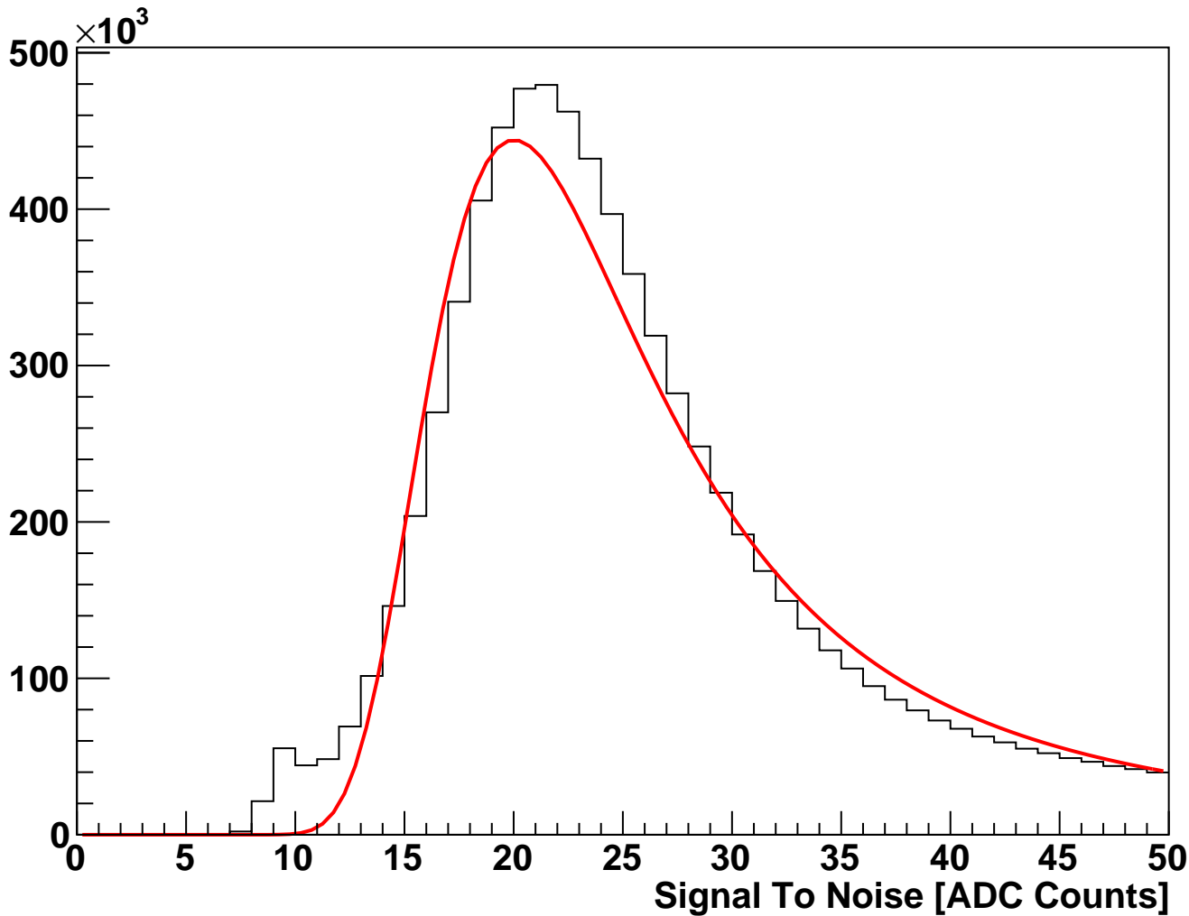
module_L2t_halfmodule_axial_sensor0 Fitted Signal To Noise (hits on clean track)
