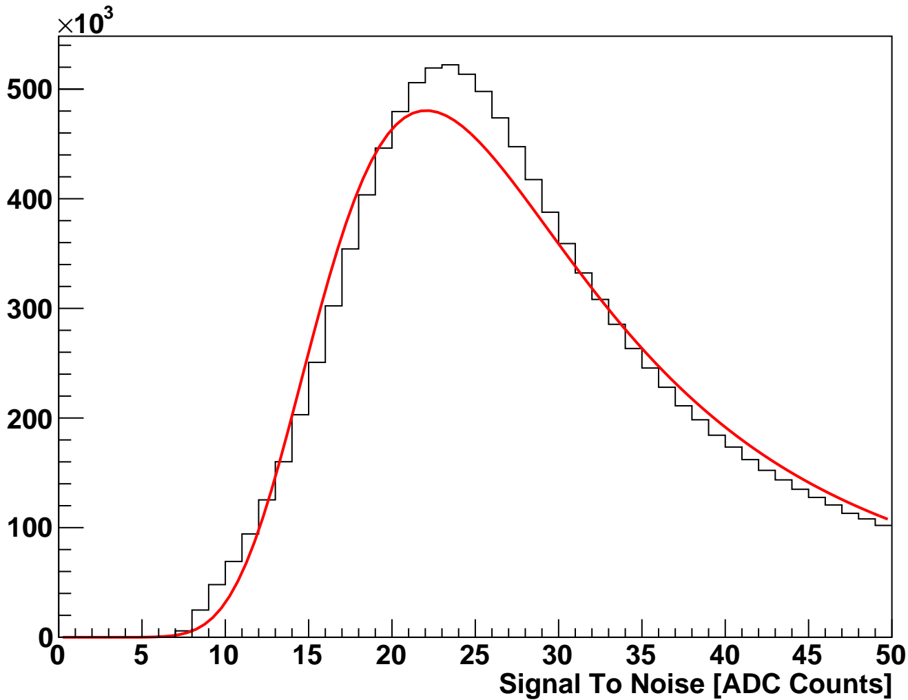
module_L1t_halfmodule_axial_sensor0 Fitted Signal To Noise (hits on clean track)
