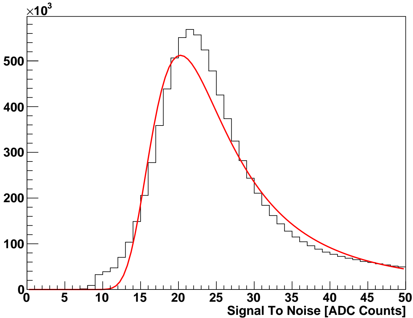
module_L3b_halfmodule_axial_sensor0 Fitted Signal To Noise (hits on clean track)
