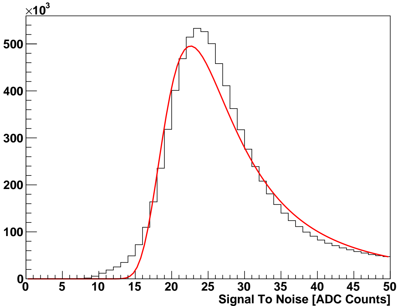
module_L4b_halfmodule_axial_hole_sensor0 Fitted Signal To Noise (hits on clean track)
