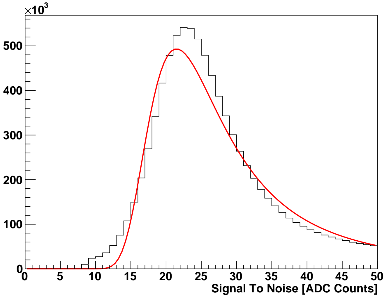
module_L2b_halfmodule_stereo_sensor0 Fitted Signal To Noise (hits on clean track)
