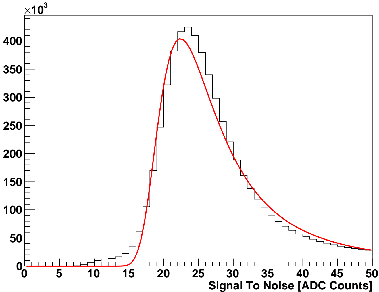
module_L6b_halfmodule_stereo_hole_sensor0 Fitted Signal To Noise (hits on clean track)
