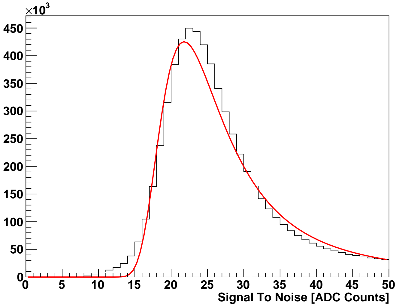
module_L4t_halfmodule_axial_hole_sensor0 Fitted Signal To Noise (hits on clean track)
