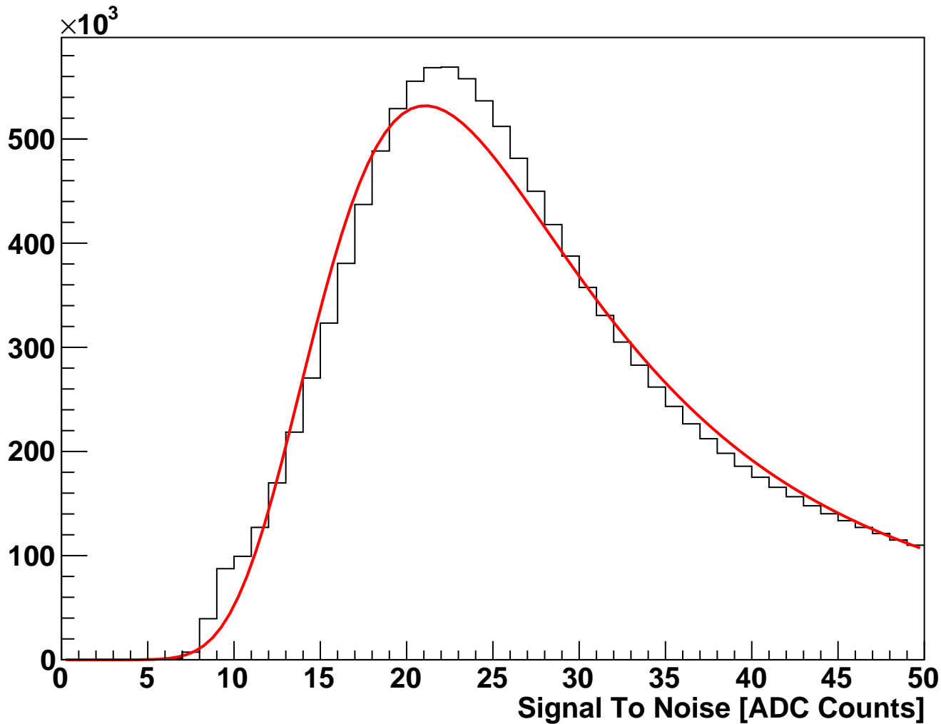
module_L1t_halfmodule_stereo_sensor0 Fitted Signal To Noise (hits on clean track)
