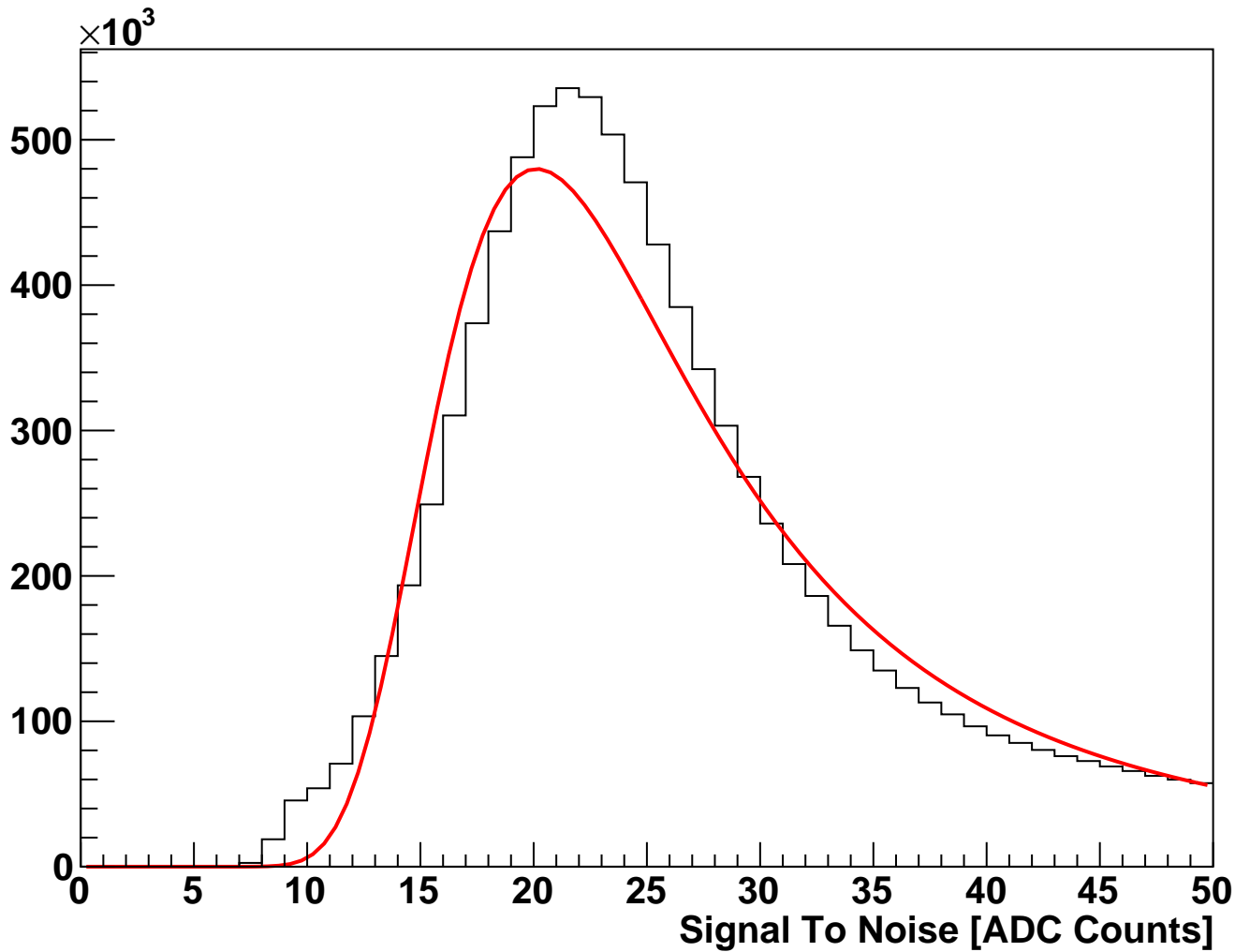
module_L2b_halfmodule_axial_sensor0 Fitted Signal To Noise (hits on clean track)
