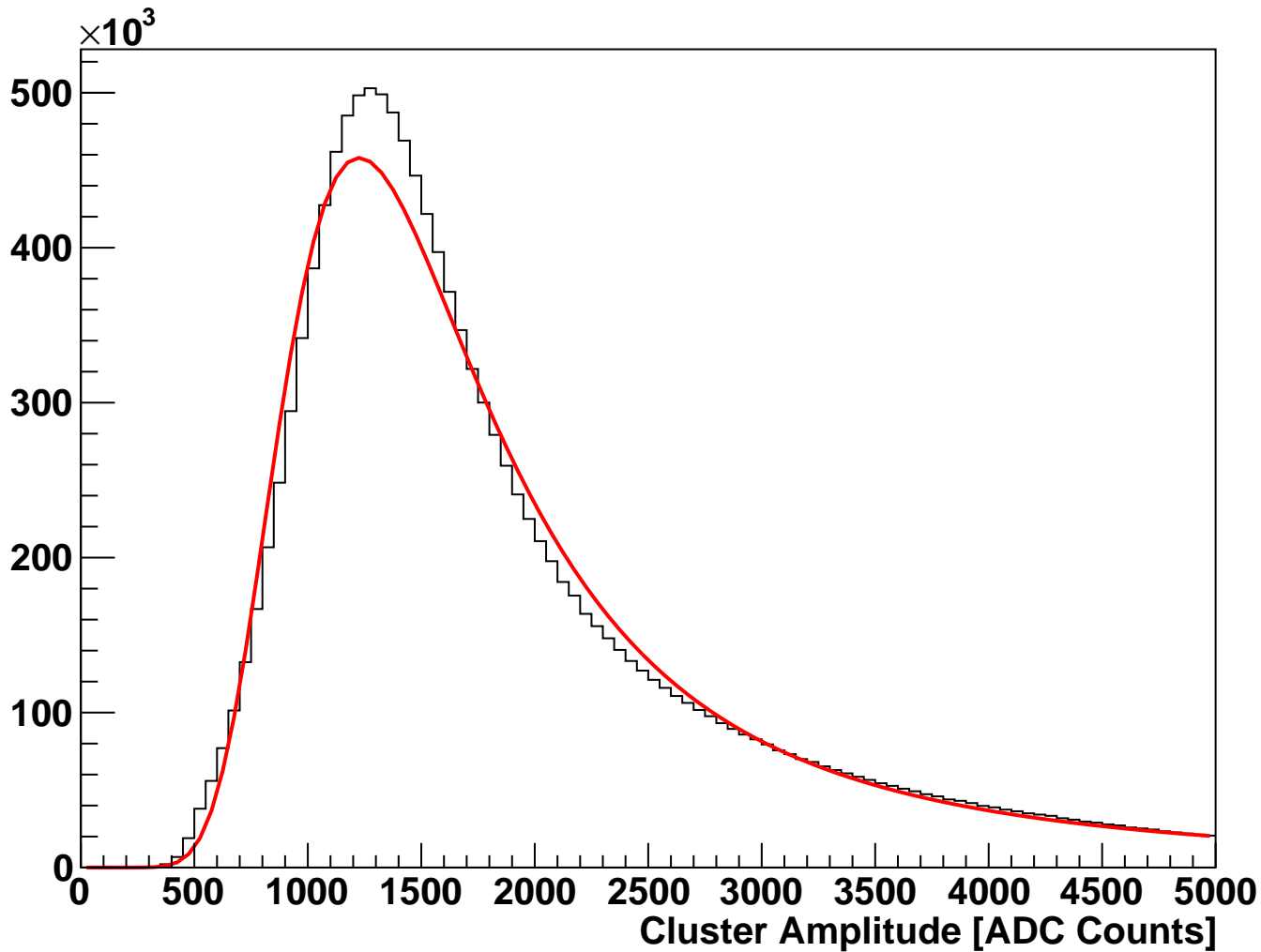
module_L1b_halfmodule_stereo_sensor0 Fitted Cluster Amplitude (hits on clean track)
