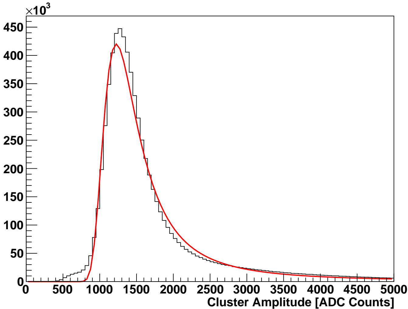
module_L5b_halfmodule_stereo_hole_sensor0 Fitted Cluster Amplitude (hits on clean track)
