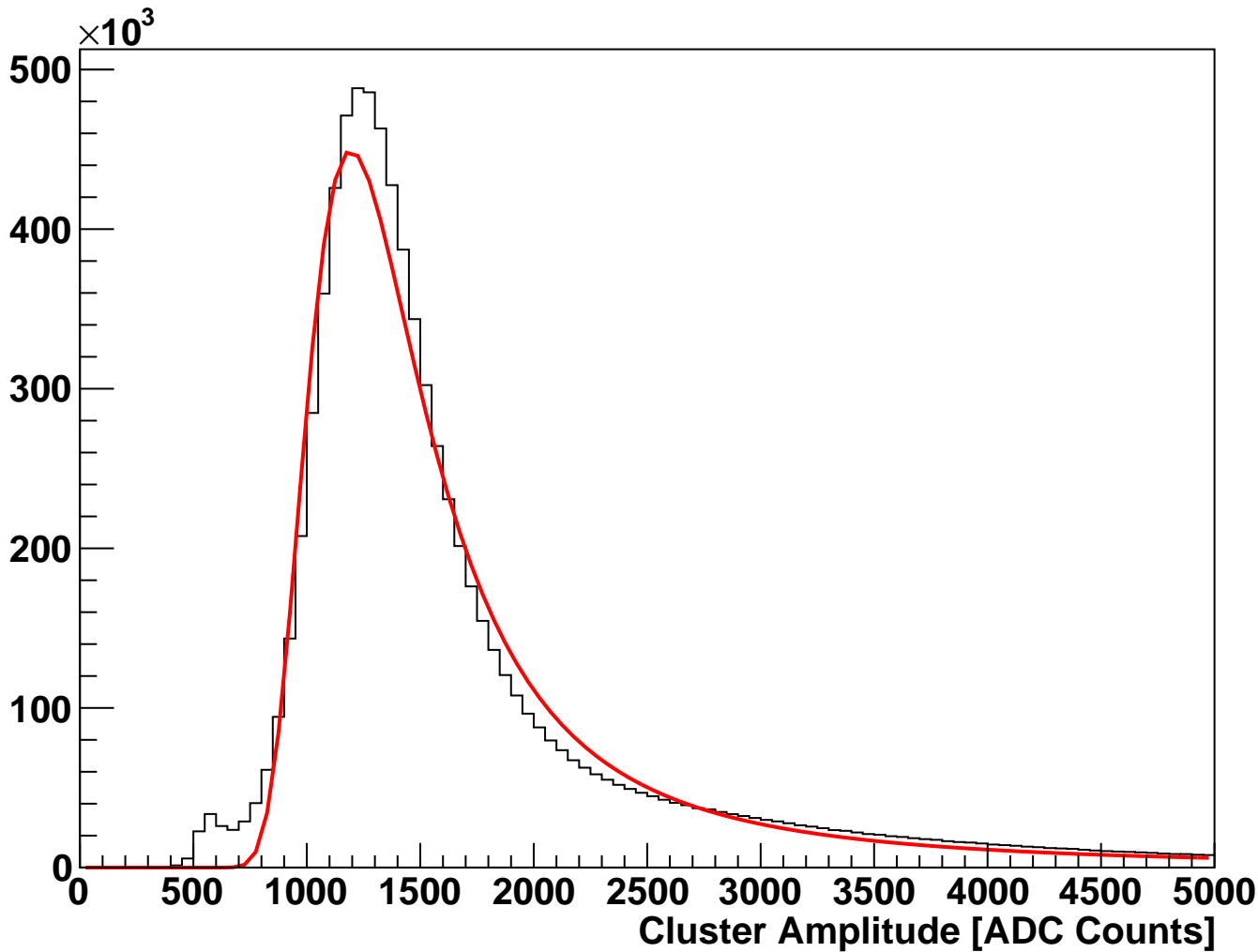
module_L3b_halfmodule_stereo_sensor0 Fitted Cluster Amplitude (hits on clean track)
