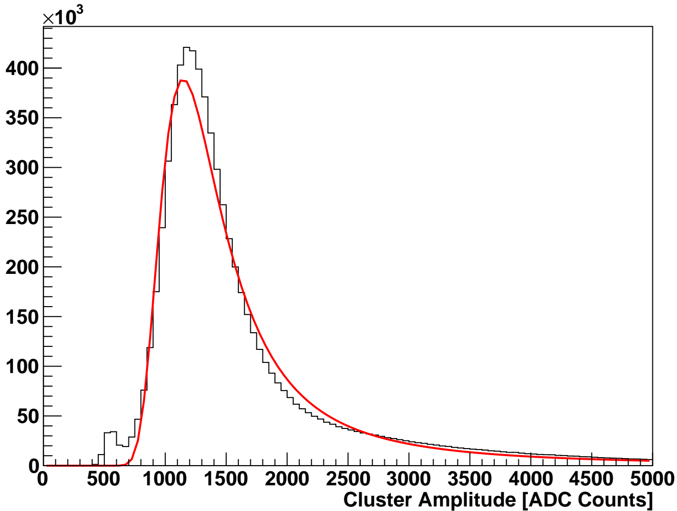
module_L3t_halfmodule_axial_sensor0 Fitted Cluster Amplitude (hits on clean track)
