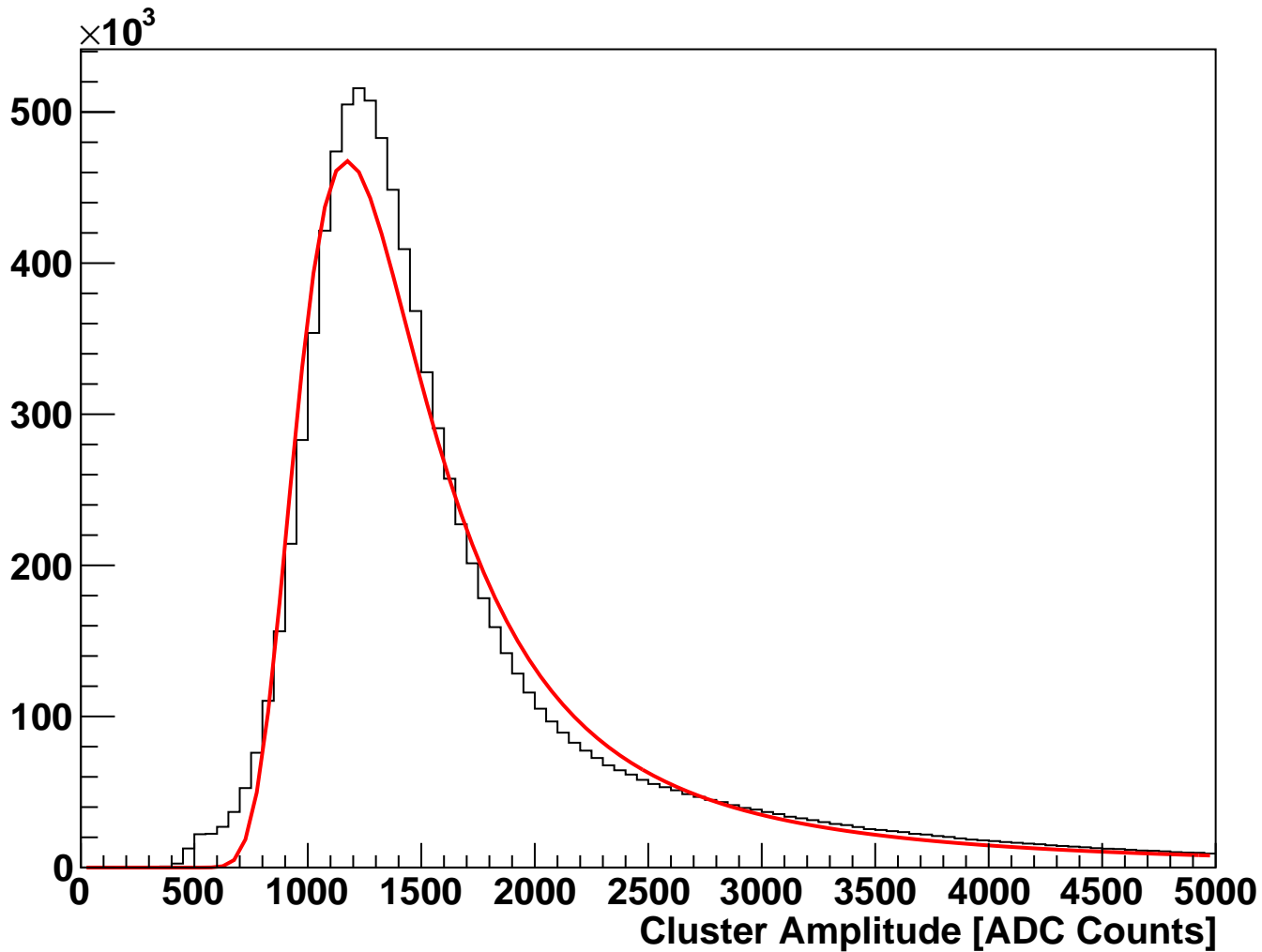
module_L2b_halfmodule_stereo_sensor0 Fitted Cluster Amplitude (hits on clean track)
