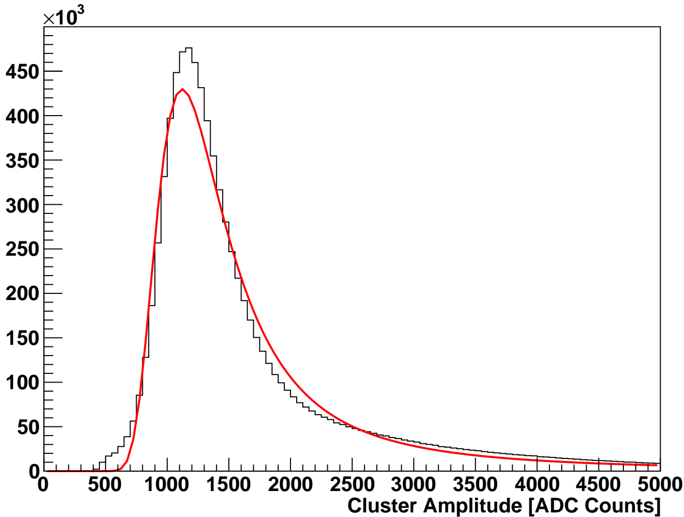
module_L2t_halfmodule_stereo_sensor0 Fitted Cluster Amplitude (hits on clean track)
