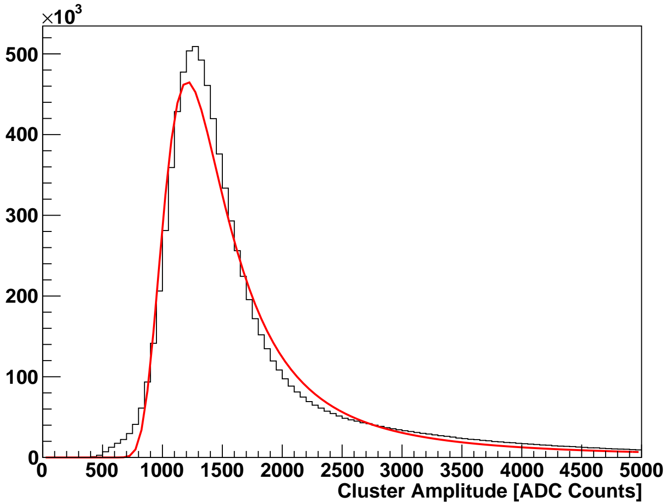
module_L4b_halfmodule_axial_hole_sensor0 Fitted Cluster Amplitude (hits on clean track)
