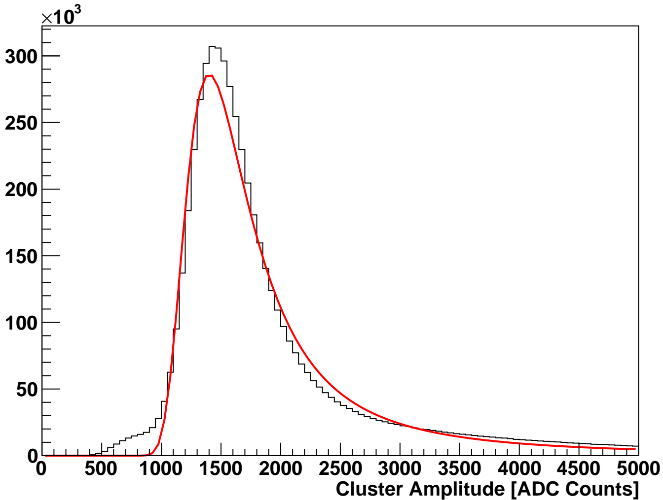
module_L6t_halfmodule_stereo_hole_sensor0 Fitted Cluster Amplitude (hits on clean track)
