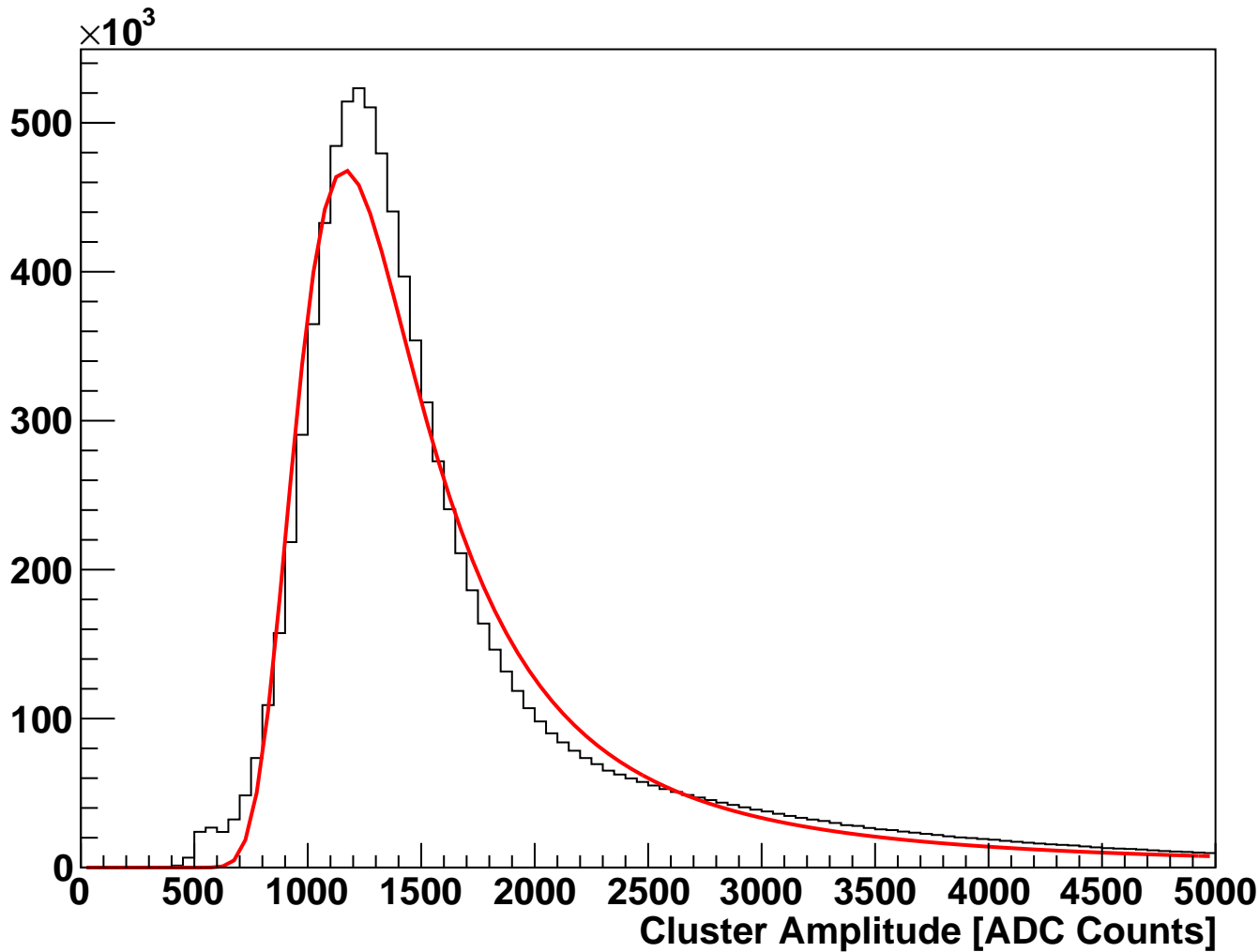
module_L3b_halfmodule_axial_sensor0 Fitted Cluster Amplitude (hits on clean track)
