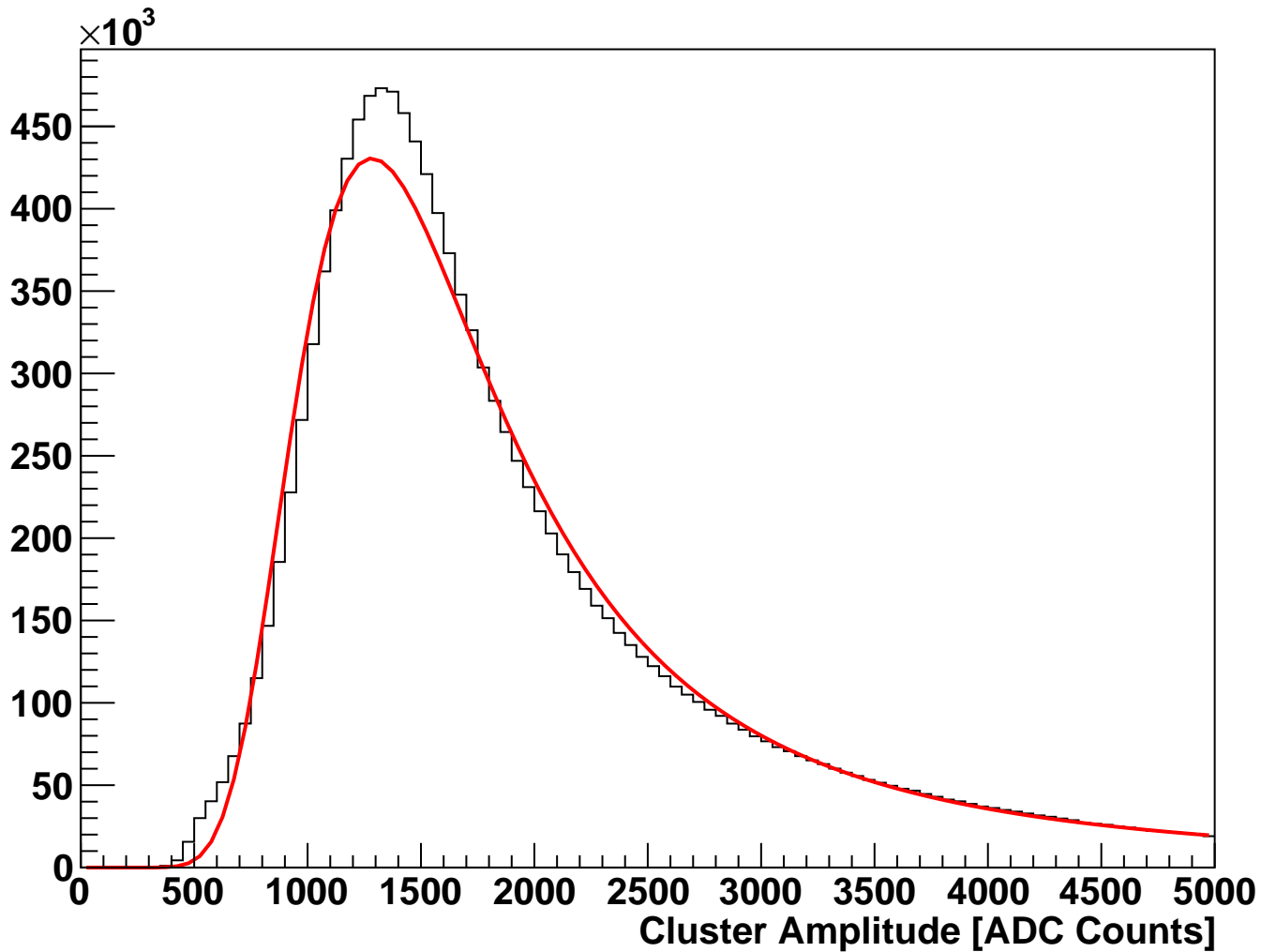
module_L1t_halfmodule_axial_sensor0 Fitted Cluster Amplitude (hits on clean track)
