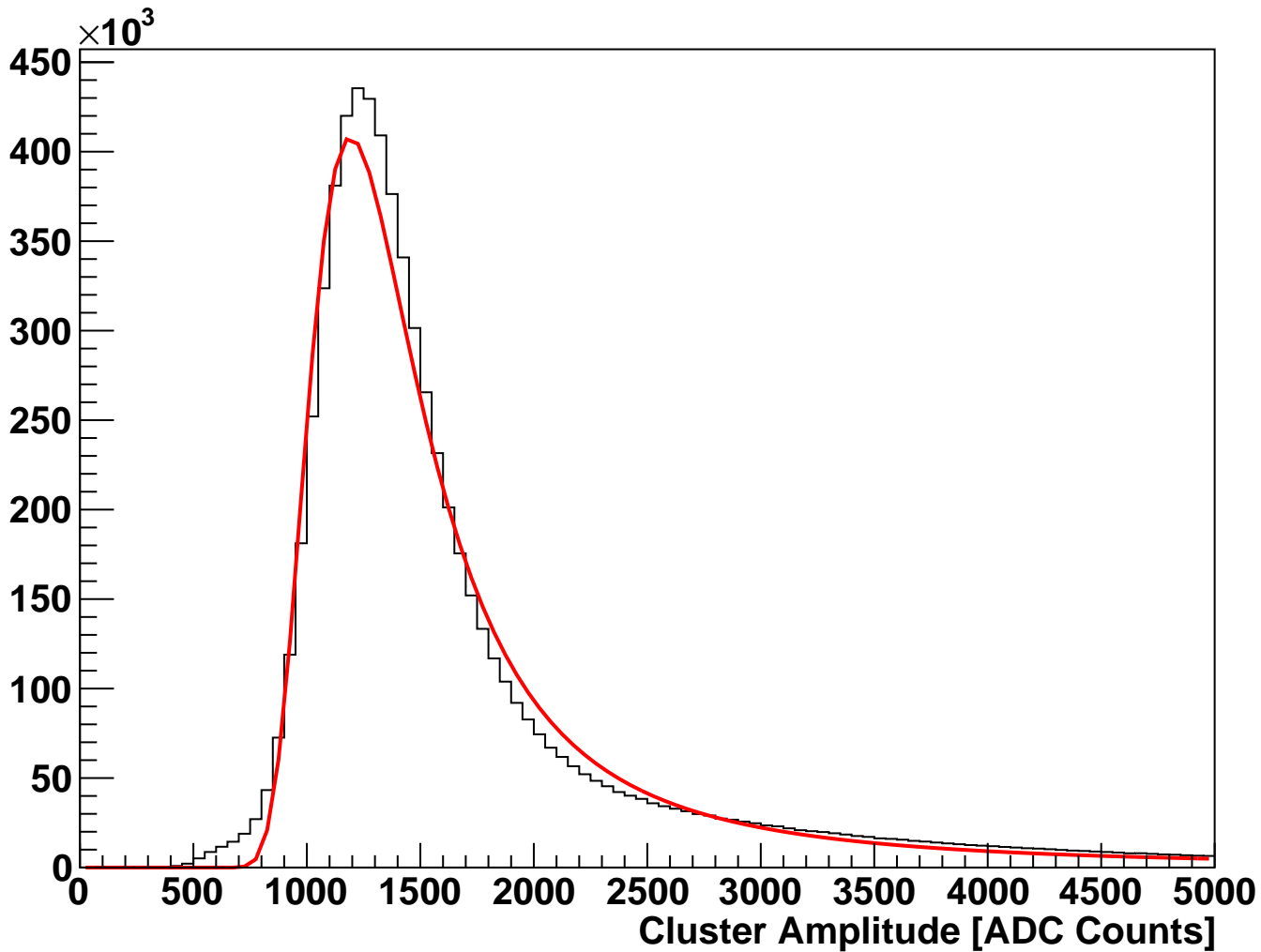
module_L4b_halfmodule_stereo_hole_sensor0 Fitted Cluster Amplitude (hits on clean track)
