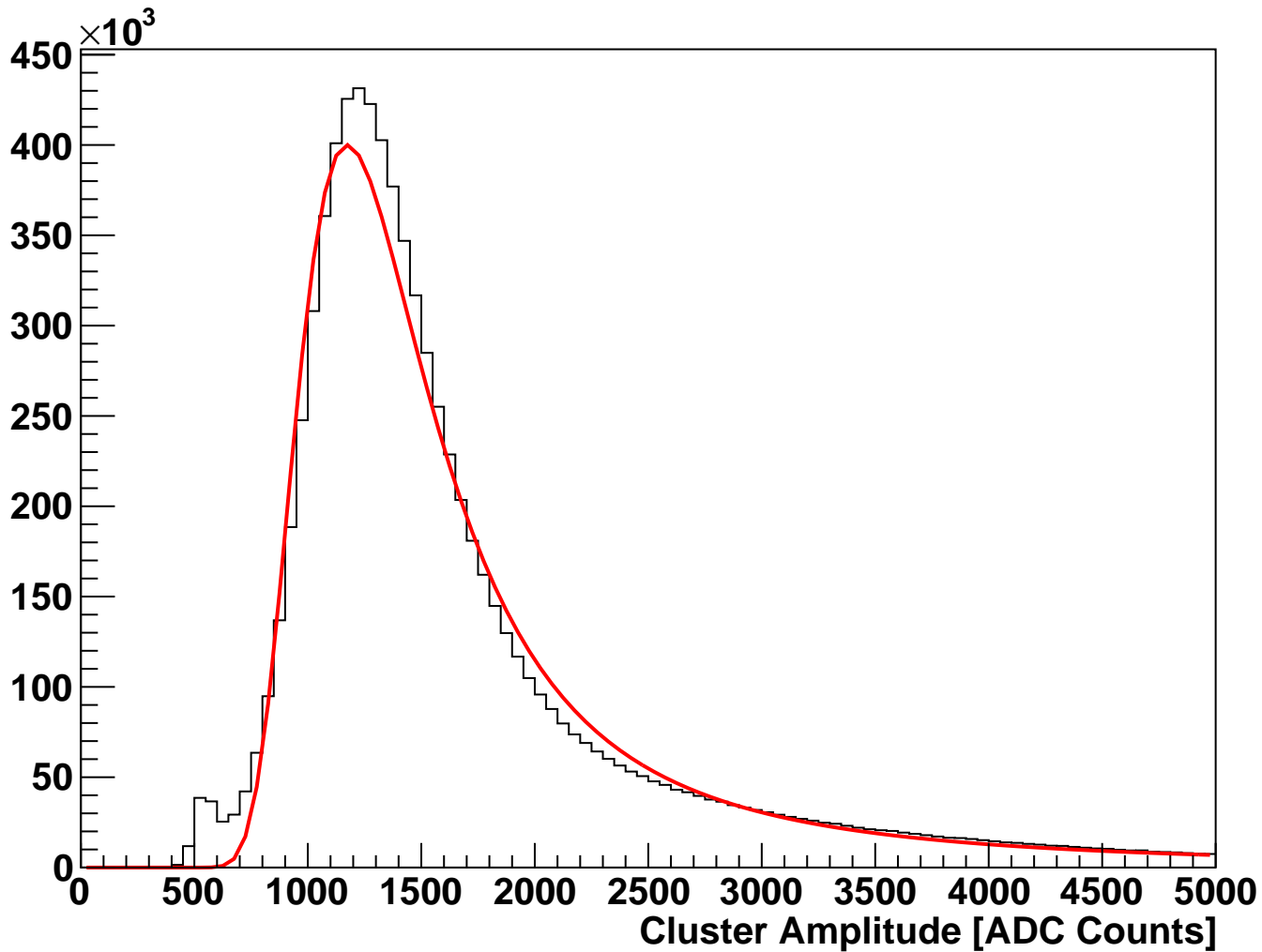
module_L2t_halfmodule_axial_sensor0 Fitted Cluster Amplitude (hits on clean track)
