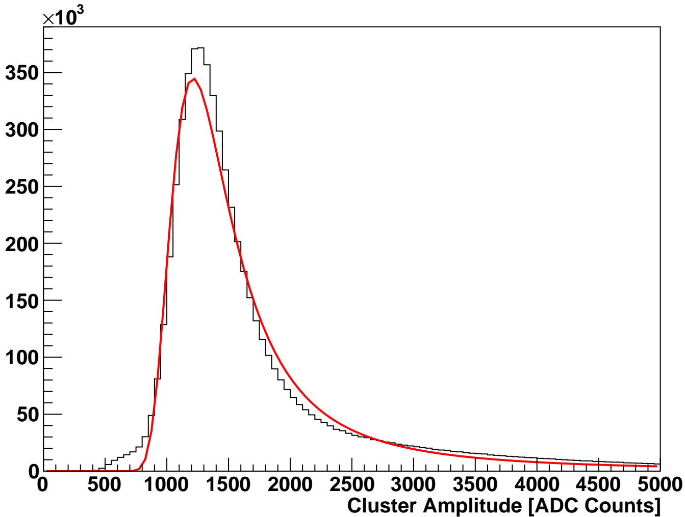
module_L5t_halfmodule_stereo_hole_sensor0 Fitted Cluster Amplitude (hits on clean track)
