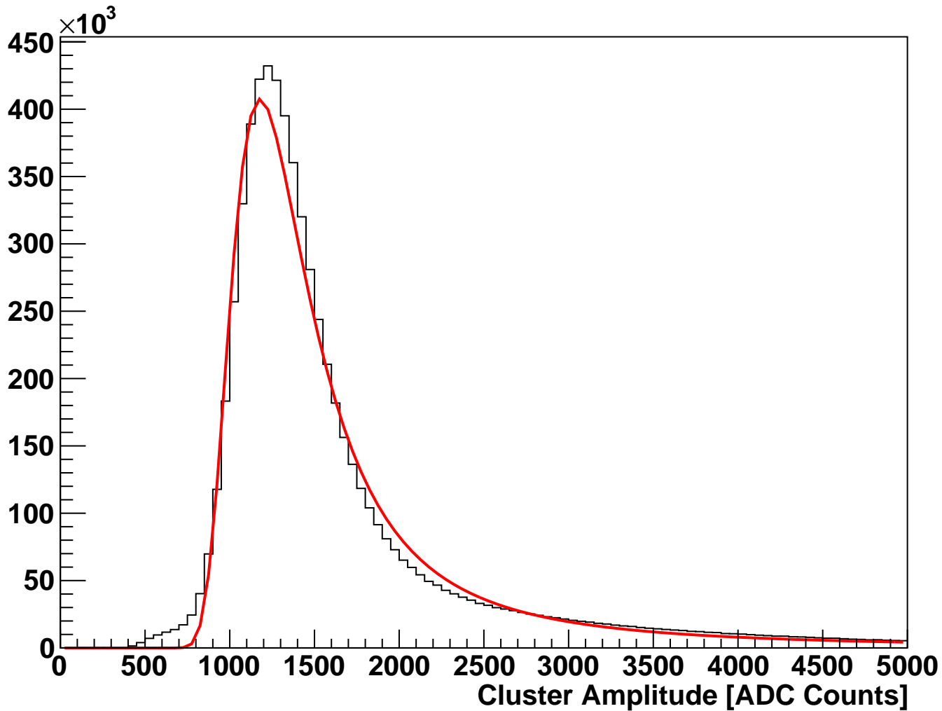
module_L5t_halfmodule_axial_hole_sensor0 Fitted Cluster Amplitude (hits on clean track)
