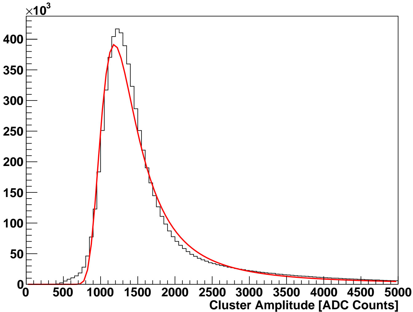
module_L4t_halfmodule_axial_hole_sensor0 Fitted Cluster Amplitude (hits on clean track)
