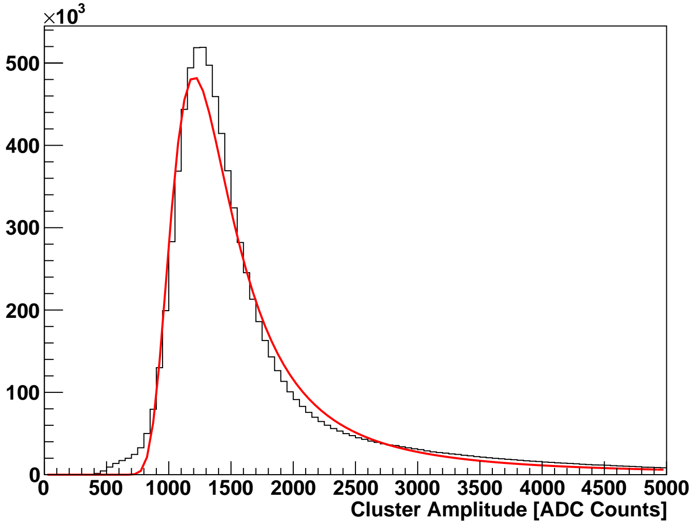
module_L5b_halfmodule_axial_hole_sensor0 Fitted Cluster Amplitude (hits on clean track)
