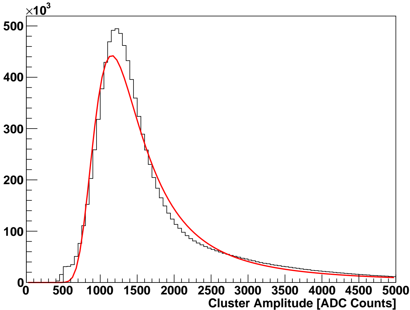
module_L2b_halfmodule_axial_sensor0 Fitted Cluster Amplitude (hits on clean track)
