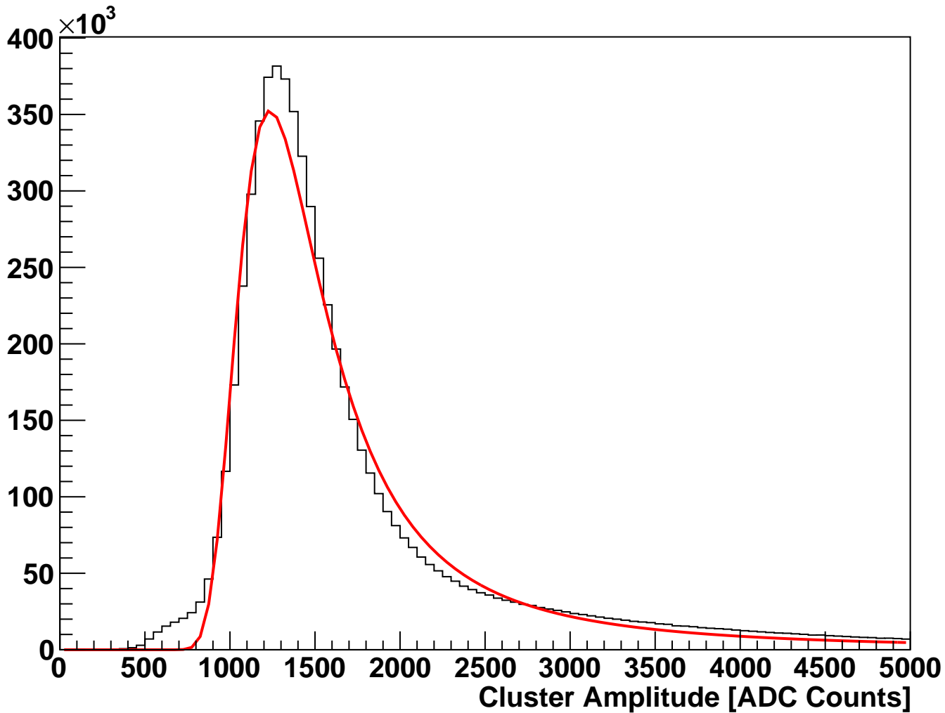
module_L4t_halfmodule_stereo_hole_sensor0 Fitted Cluster Amplitude (hits on clean track)
