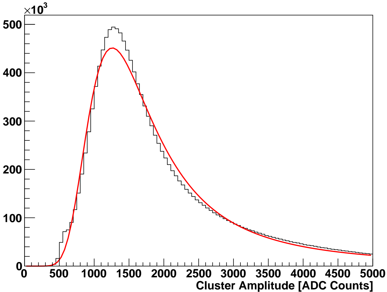
module_L1t_halfmodule_stereo_sensor0 Fitted Cluster Amplitude (hits on clean track)
