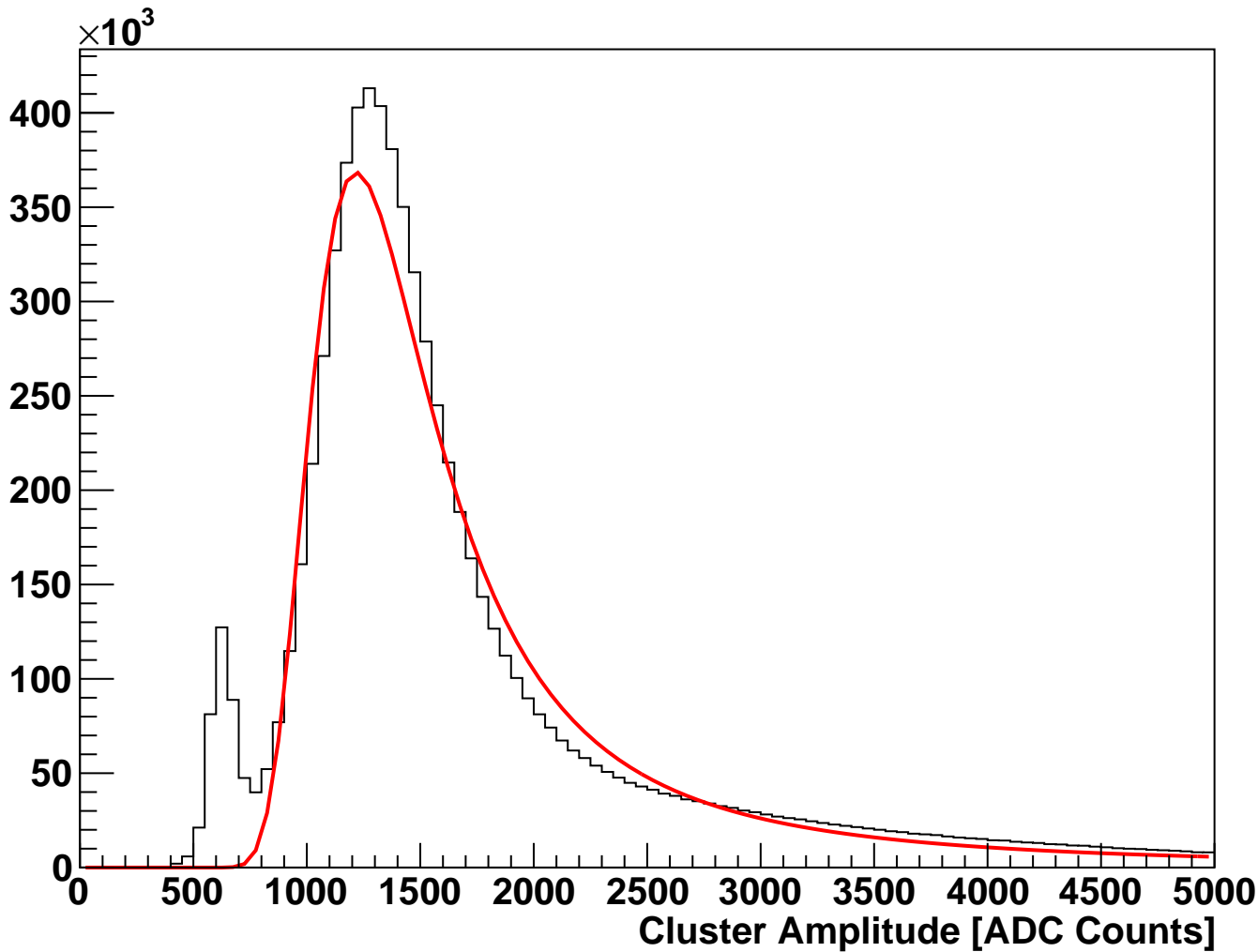
module_L3t_halfmodule_stereo_sensor0 Fitted Cluster Amplitude (hits on clean track)
