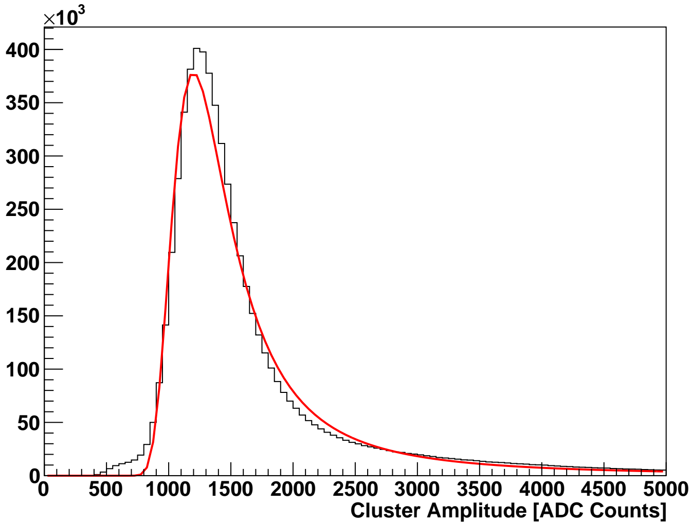
module_L6b_halfmodule_stereo_hole_sensor0 Fitted Cluster Amplitude (hits on clean track)
