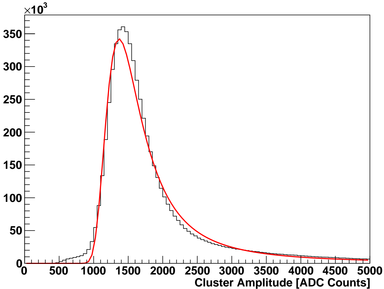
module_L6t_halfmodule_axial_hole_sensor0 Fitted Cluster Amplitude (hits on clean track)
