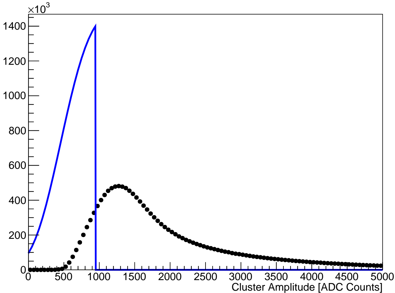
module_L1b_halfmodule_axial_sensor0 Fitted Cluster Amplitude (hits on clean track)
