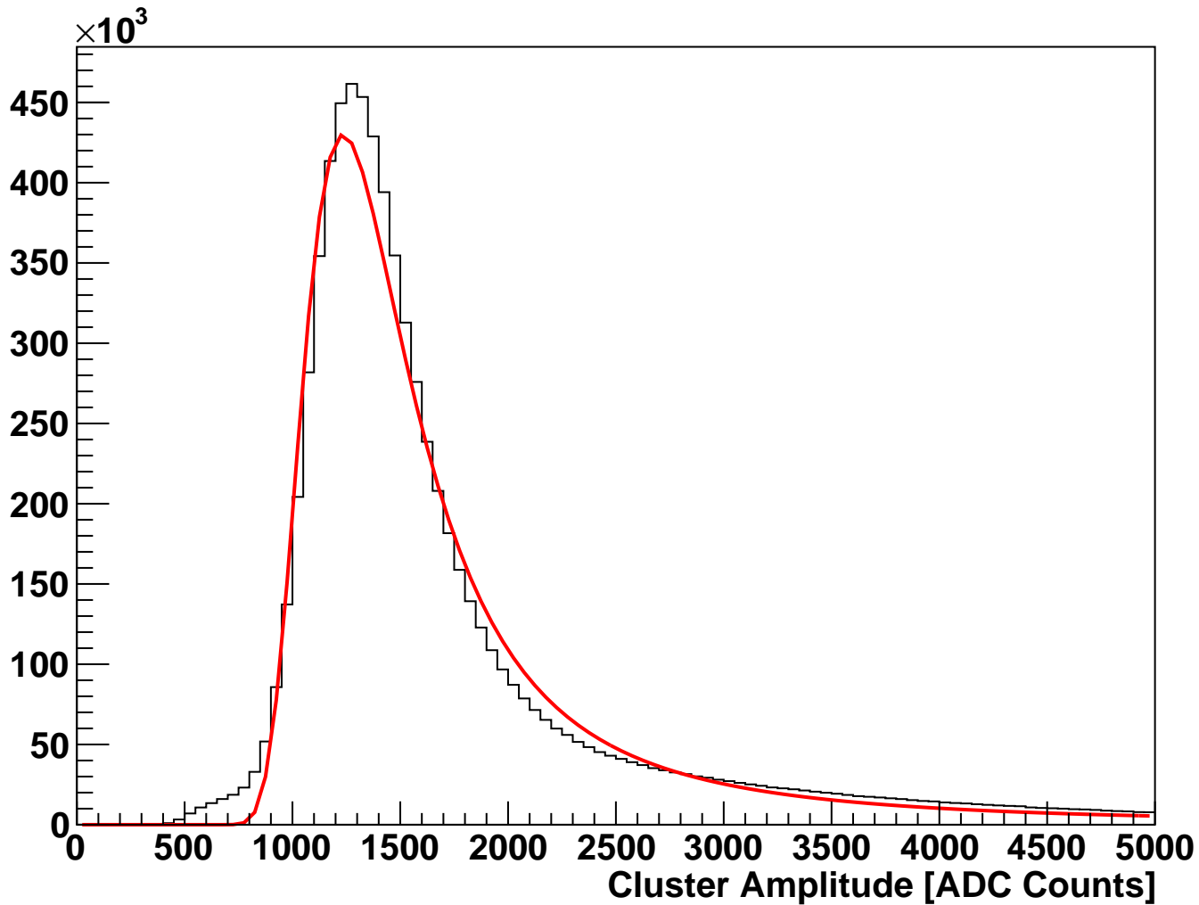
module_L6b_halfmodule_axial_hole_sensor0 Fitted Cluster Amplitude (hits on clean track)
