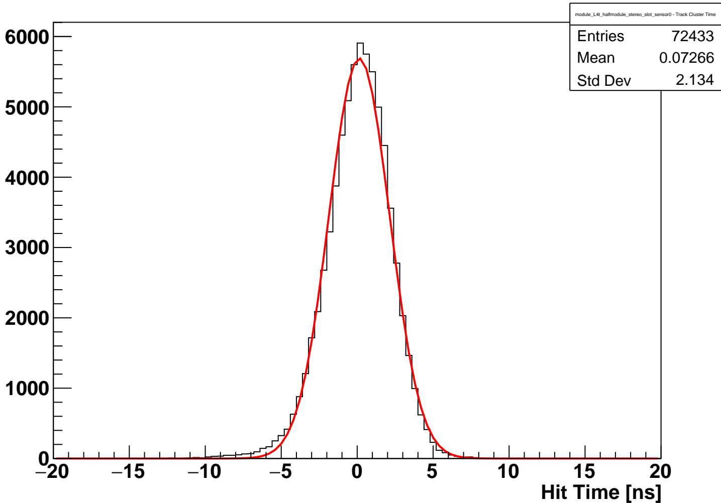
module_L4t_halfmodule_stereo_slot_sensor0 Fitted Hit Time (hits on clean track)
