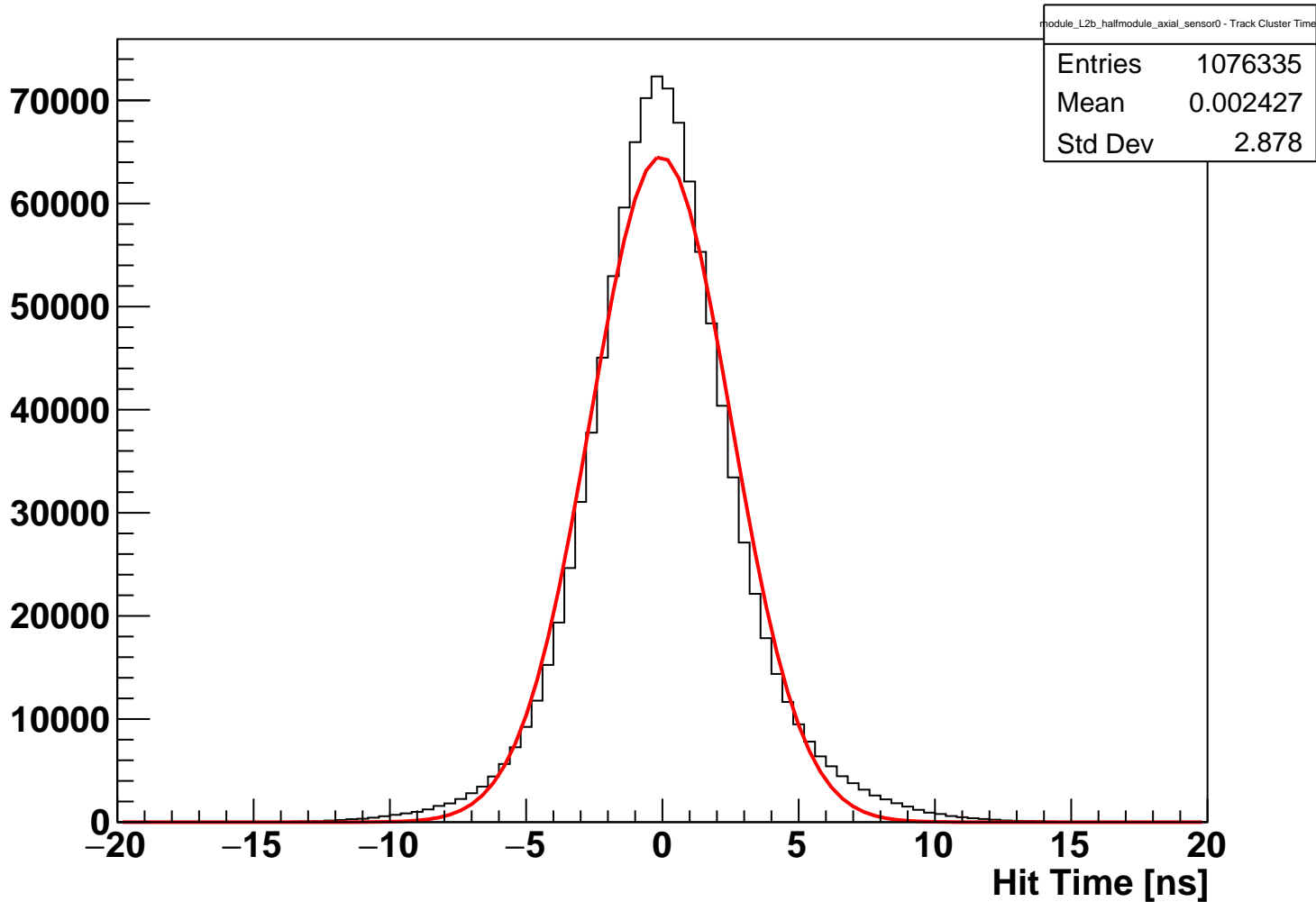
module_L2b_halfmodule_axial_sensor0 Fitted Hit Time (hits on clean track)
