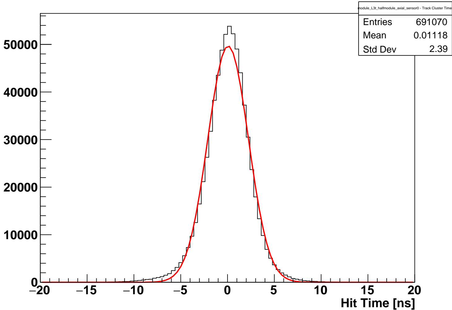
module_L3t_halfmodule_axial_sensor0 Fitted Hit Time (hits on clean track)
