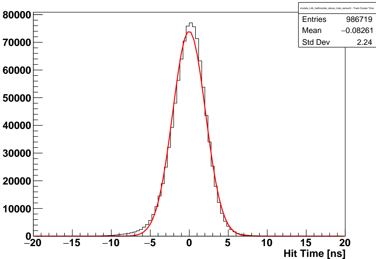
module_L4b_halfmodule_stereo_hole_sensor0 Fitted Hit Time (hits on clean track)
