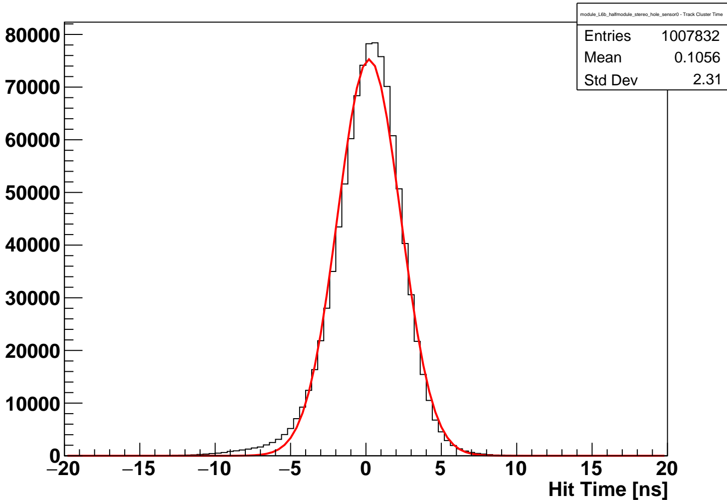
module_L6b_halfmodule_stereo_hole_sensor0 Fitted Hit Time (hits on clean track)
