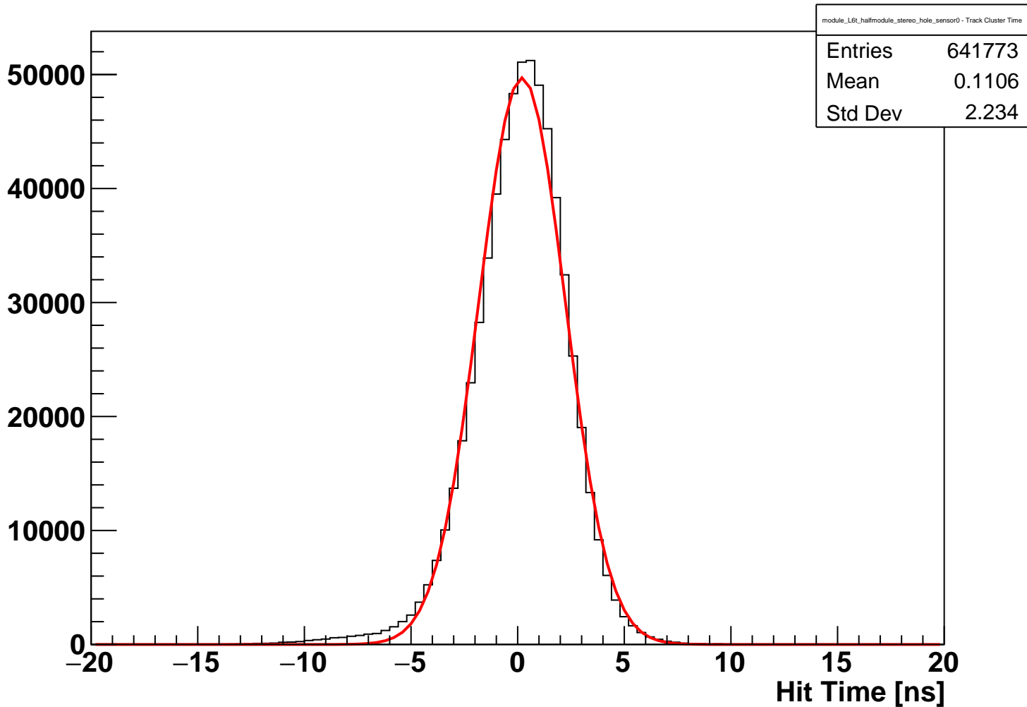
module_L6t_halfmodule_stereo_hole_sensor0 Fitted Hit Time (hits on clean track)
