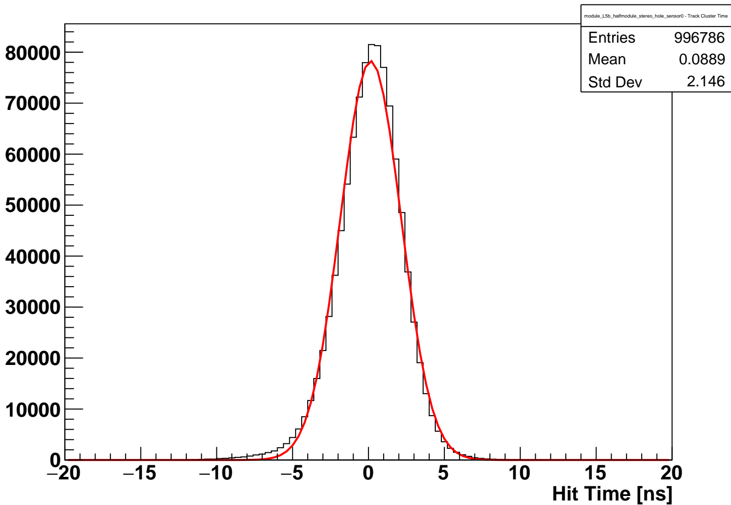
module_L5b_halfmodule_stereo_hole_sensor0 Fitted Hit Time (hits on clean track)
