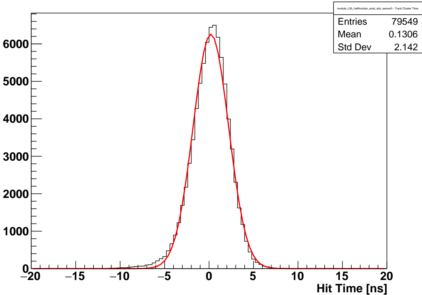
module_L5b_halfmodule_axial_slot_sensor0 Fitted Hit Time (hits on clean track)
