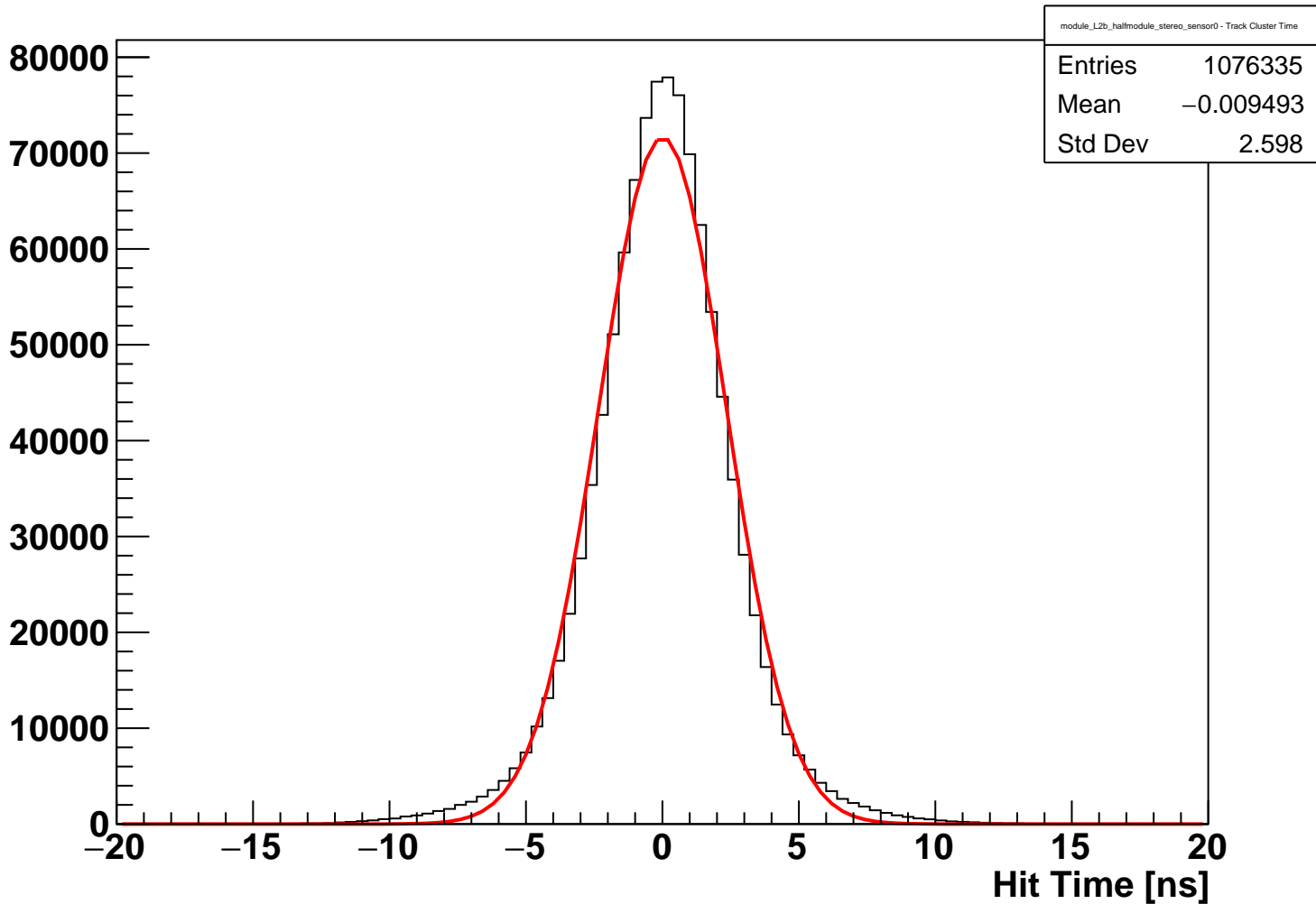
module_L2b_halfmodule_stereo_sensor0 Fitted Hit Time (hits on clean track)
