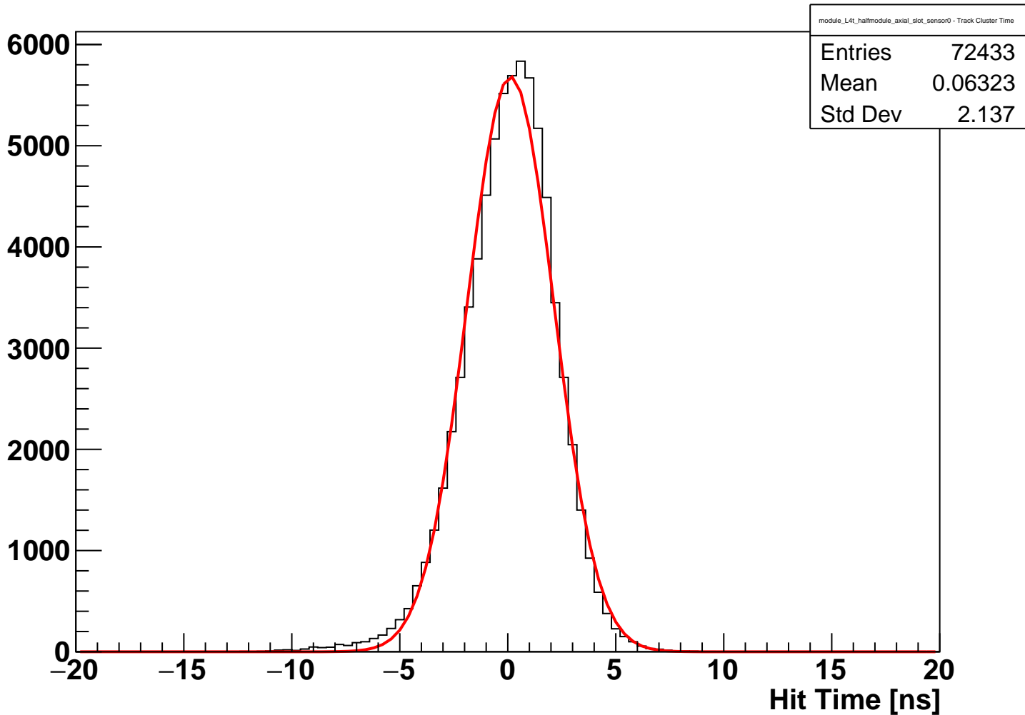
module_L4t_halfmodule_axial_slot_sensor0 Fitted Hit Time (hits on clean track)
