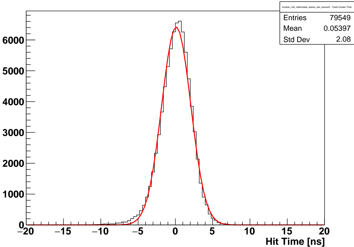
module_L5b_halfmodule_stereo_slot_sensor0 Fitted Hit Time (hits on clean track)
