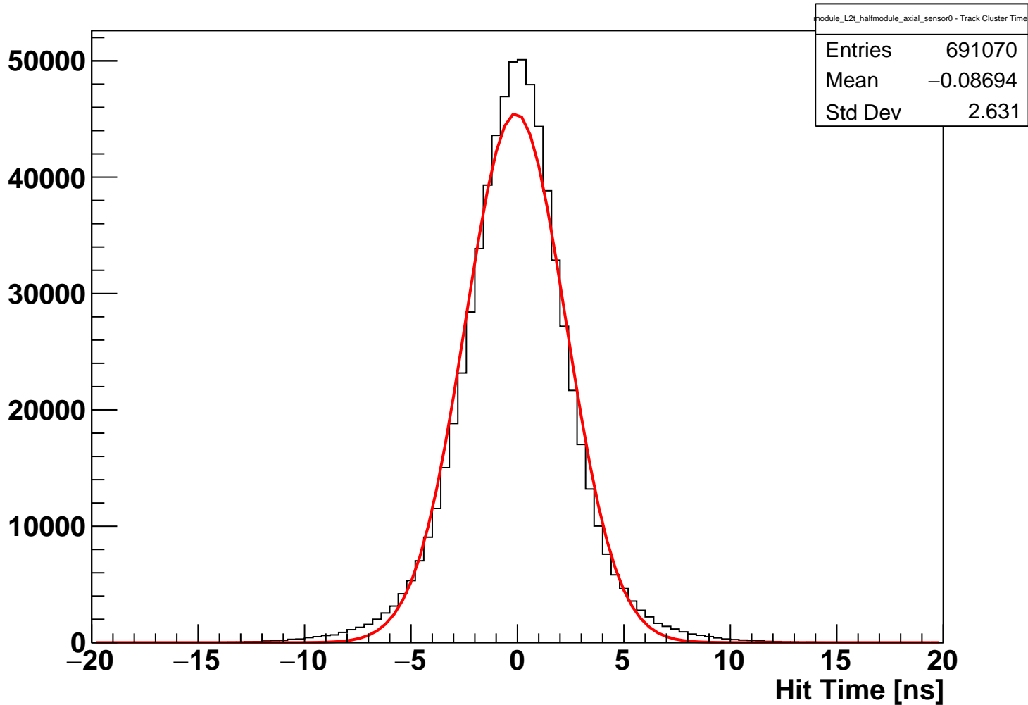
module_L2t_halfmodule_axial_sensor0 Fitted Hit Time (hits on clean track)
