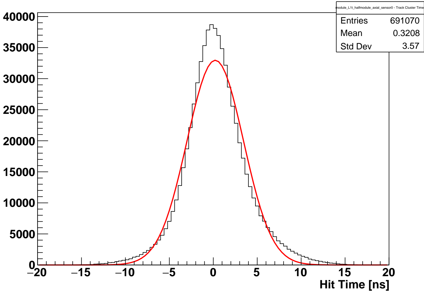
module_L1t_halfmodule_axial_sensor0 Fitted Hit Time (hits on clean track)
