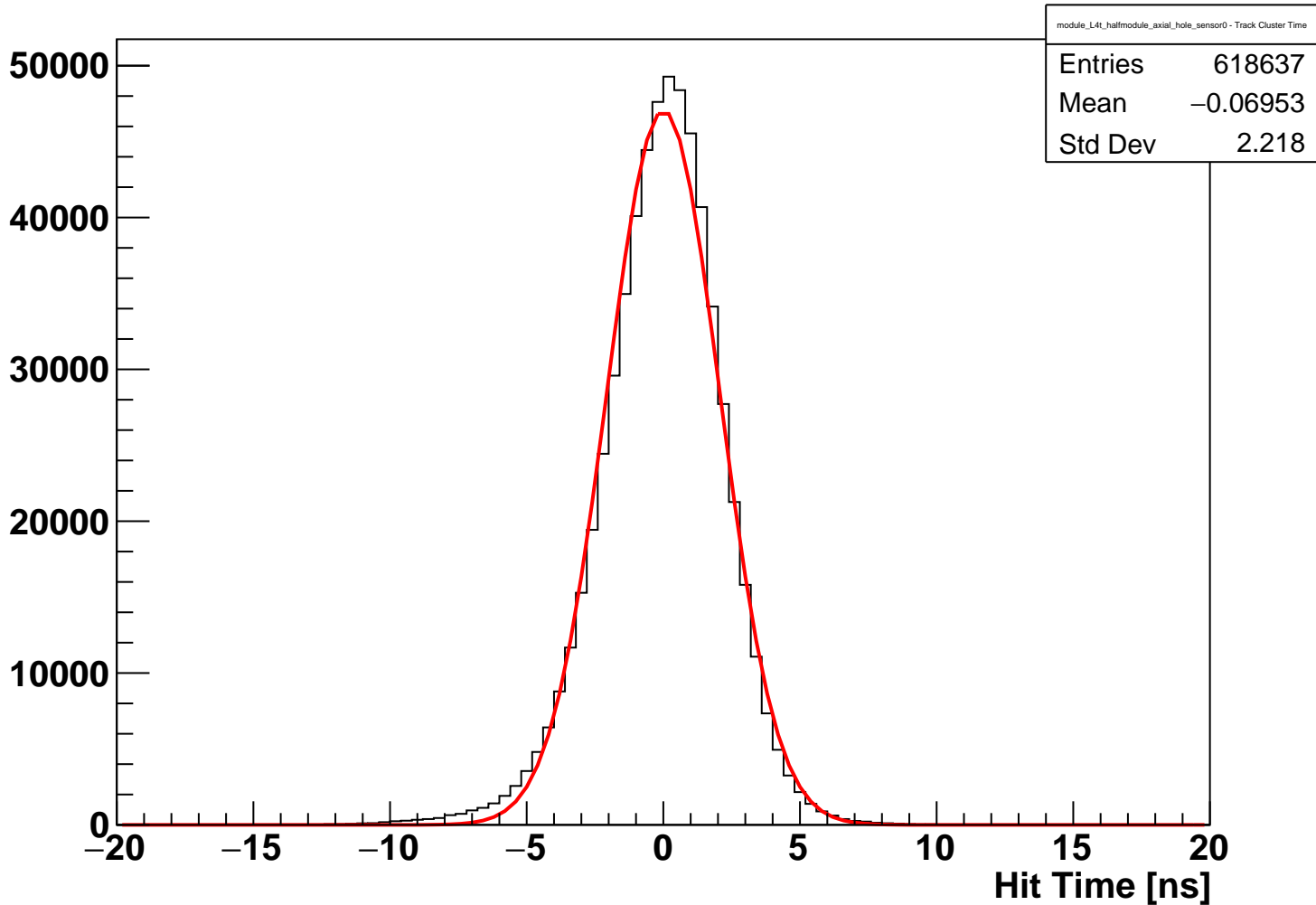
module_L4t_halfmodule_axial_hole_sensor0 Fitted Hit Time (hits on clean track)
