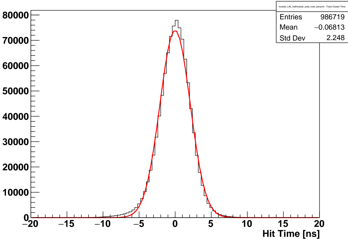
module_L4b_halfmodule_axial_hole_sensor0 Fitted Hit Time (hits on clean track)
