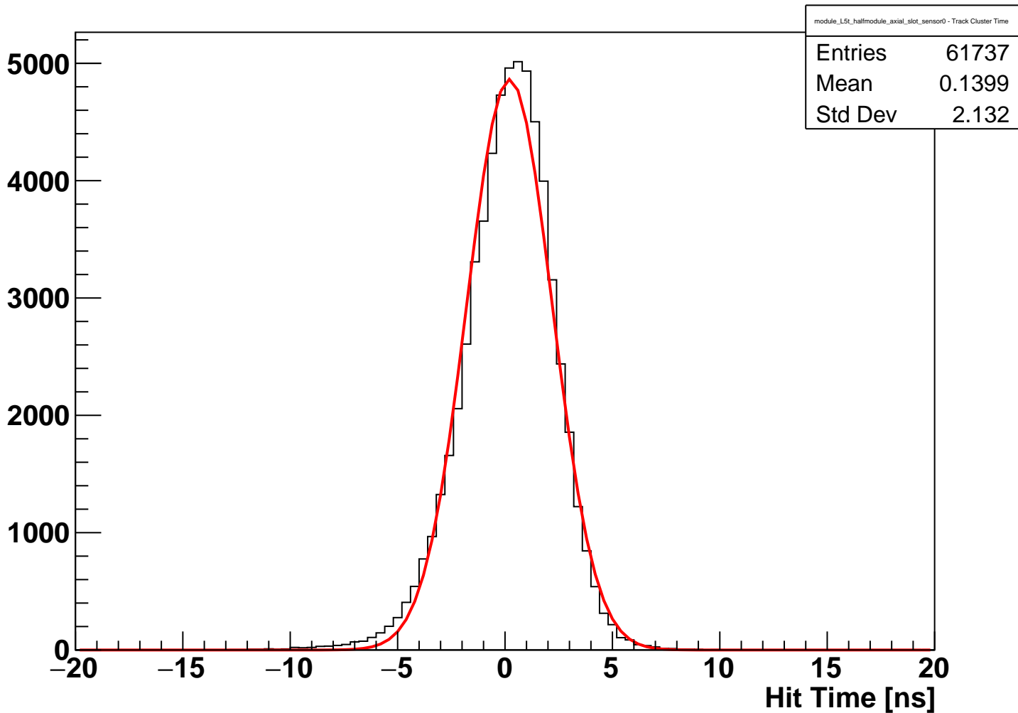
module_L5t_halfmodule_axial_slot_sensor0 Fitted Hit Time (hits on clean track)
