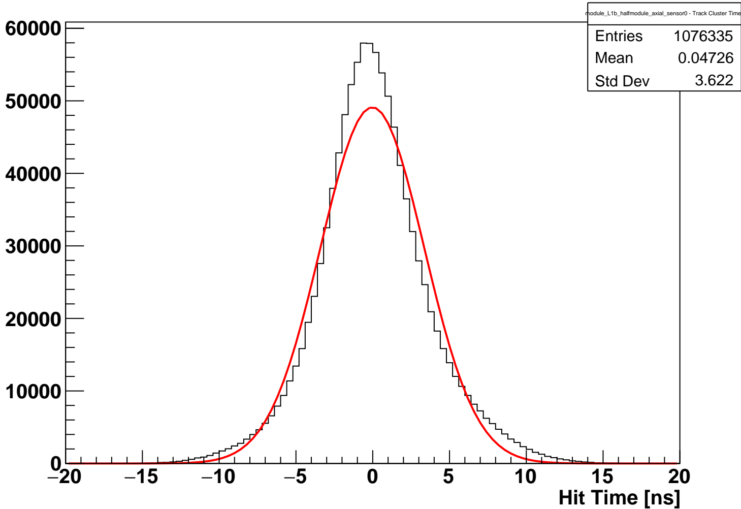
module_L1b_halfmodule_axial_sensor0 Fitted Hit Time (hits on clean track)
