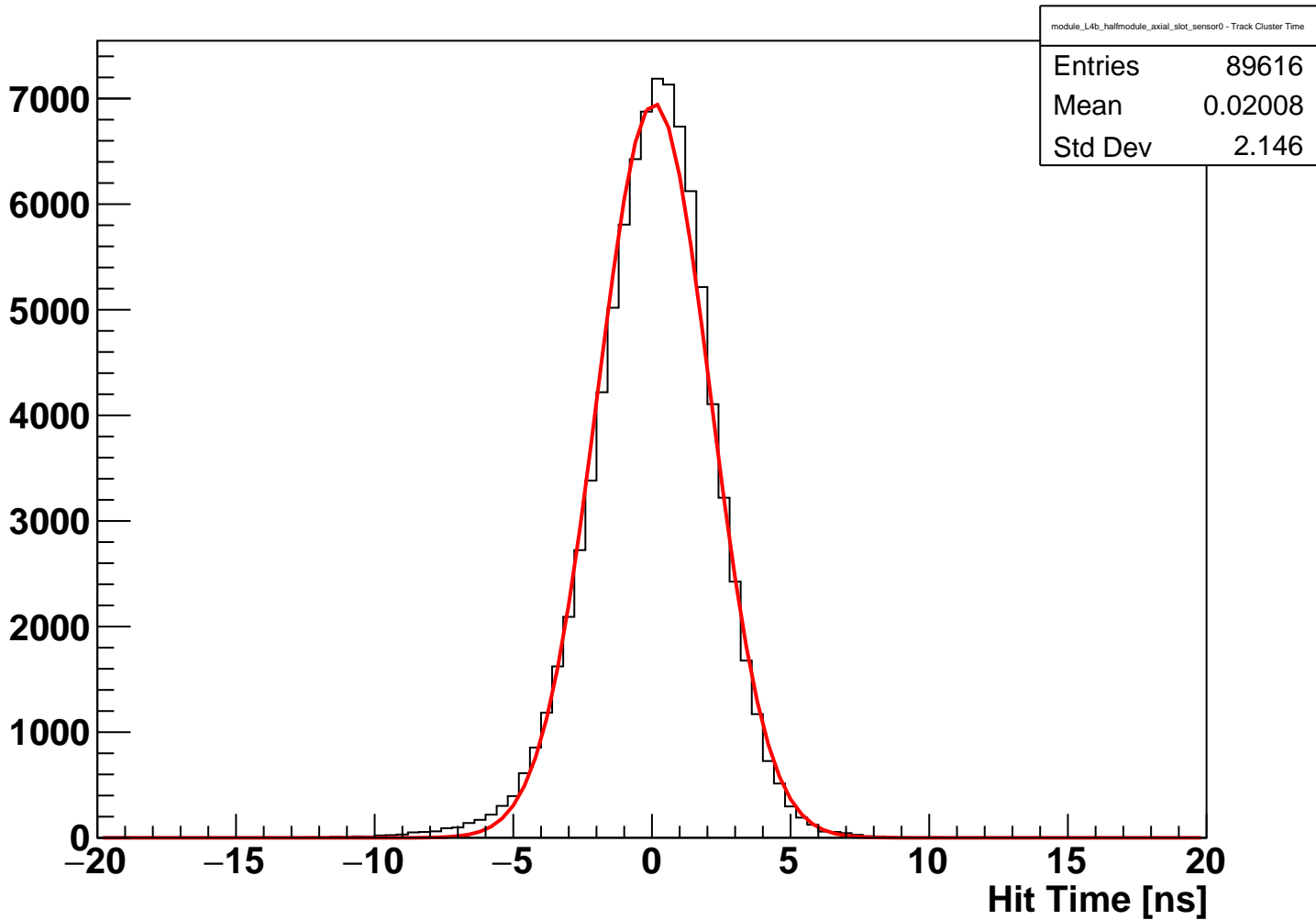
module_L4b_halfmodule_axial_slot_sensor0 Fitted Hit Time (hits on clean track)
