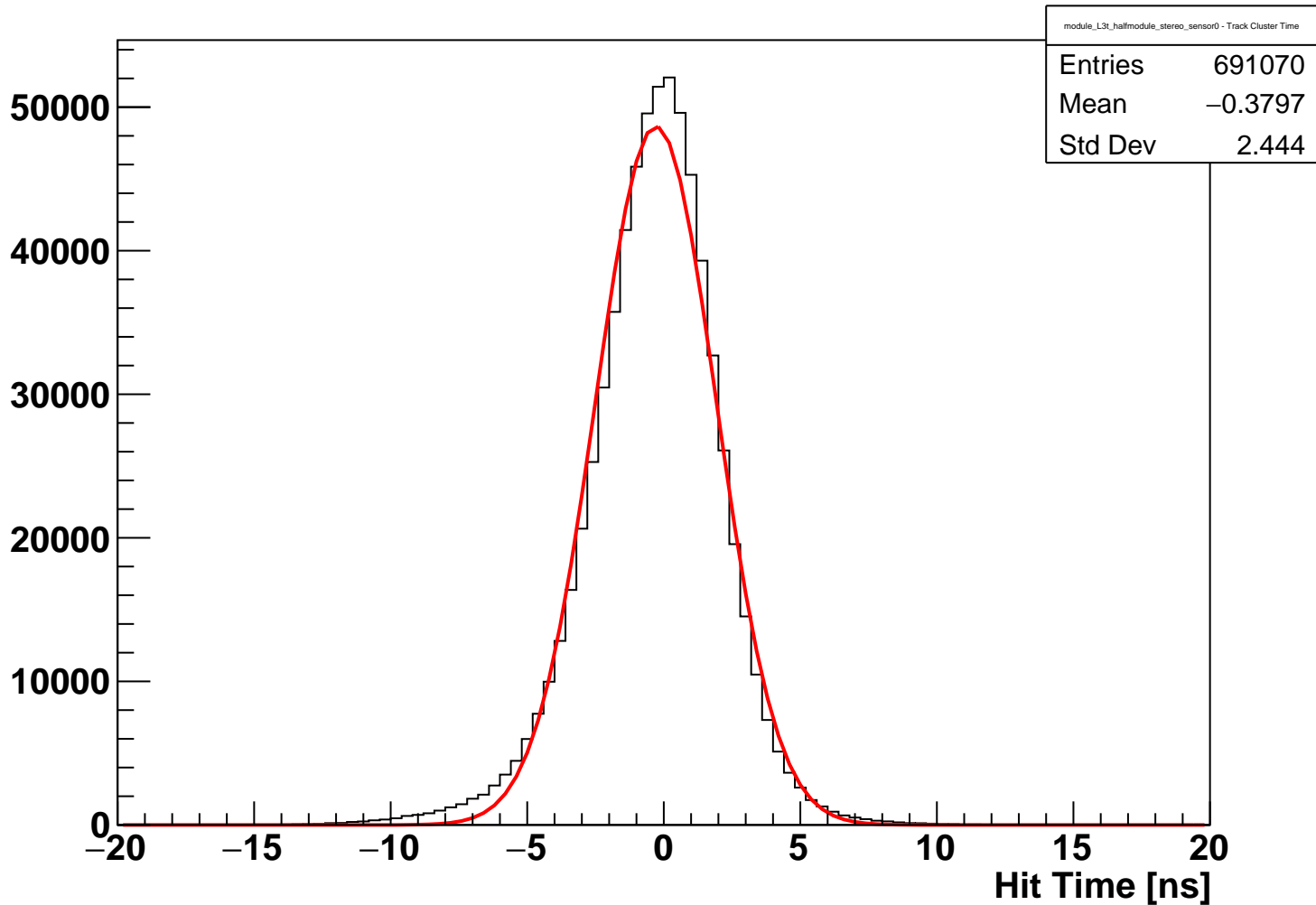
module_L3t_halfmodule_stereo_sensor0 Fitted Hit Time (hits on clean track)
