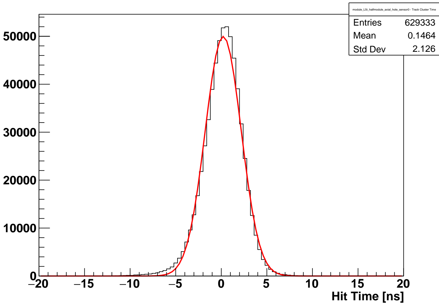
module_L5t_halfmodule_axial_hole_sensor0 Fitted Hit Time (hits on clean track)
