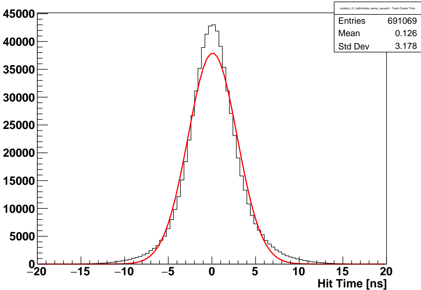
module_L1t_halfmodule_stereo_sensor0 Fitted Hit Time (hits on clean track)
