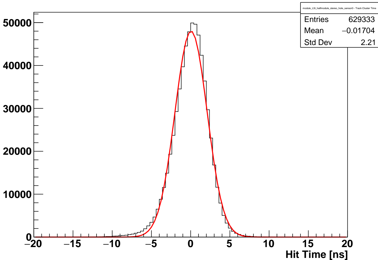
module_L5t_halfmodule_stereo_hole_sensor0 Fitted Hit Time (hits on clean track)
