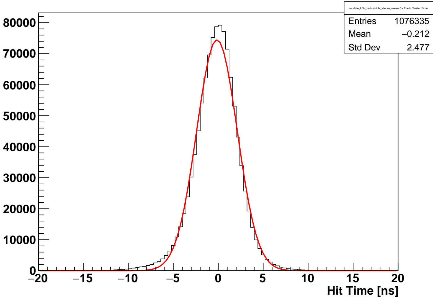
module_L3b_halfmodule_stereo_sensor0 Fitted Hit Time (hits on clean track)
