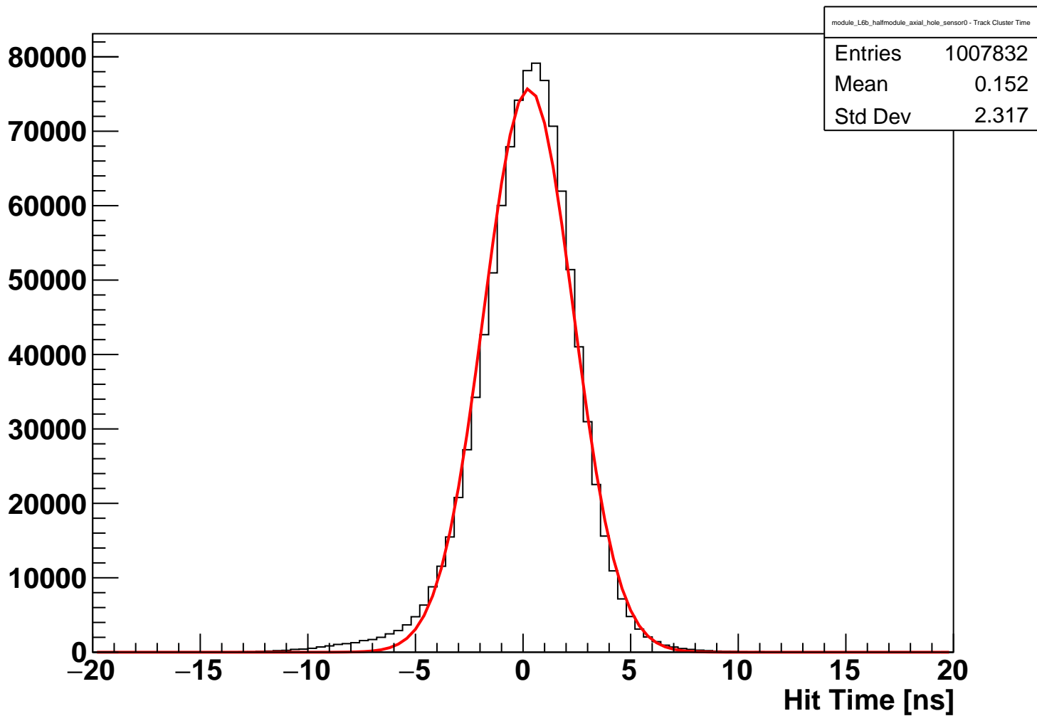
module_L6b_halfmodule_axial_hole_sensor0 Fitted Hit Time (hits on clean track)
