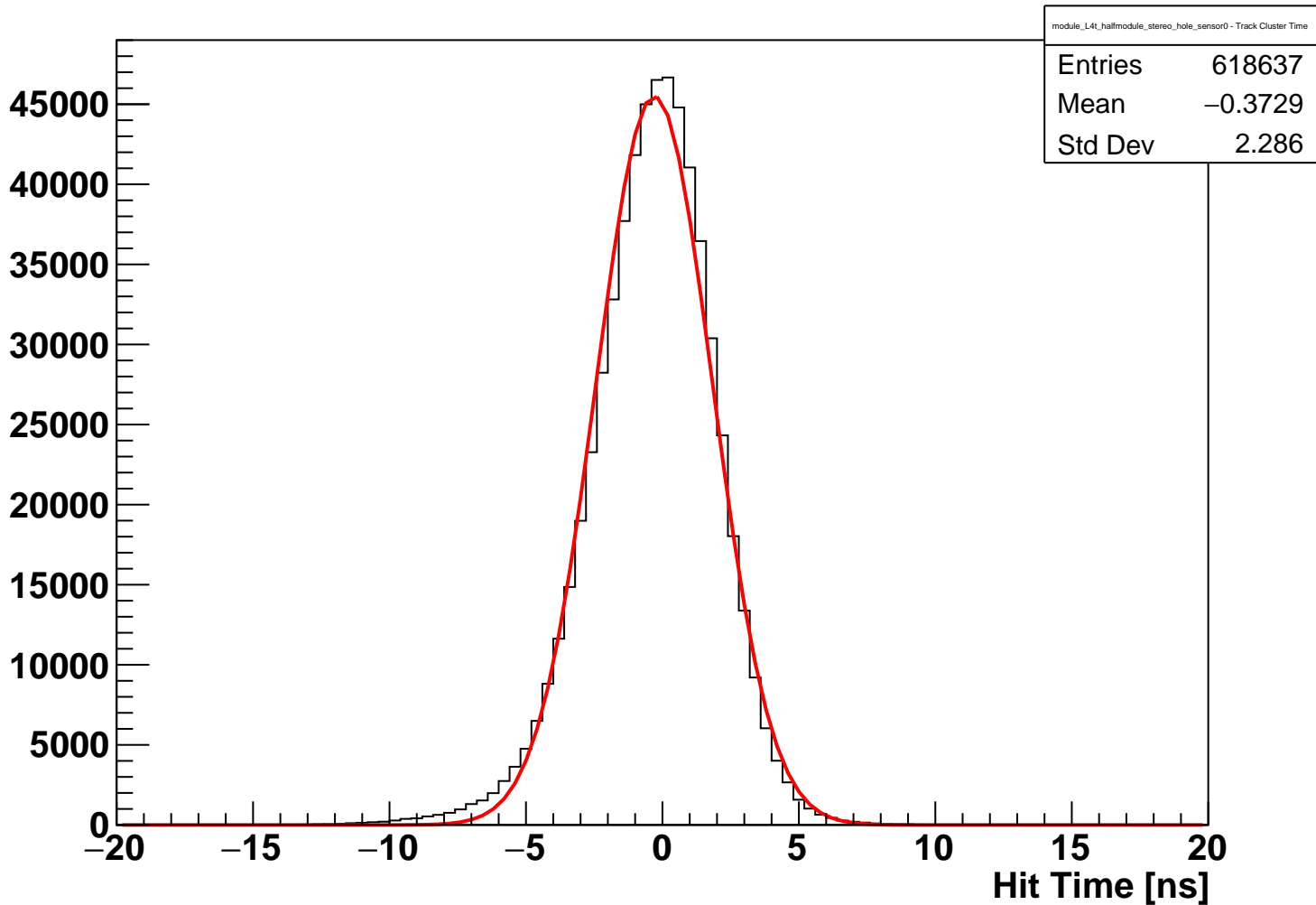
module_L4t_halfmodule_stereo_hole_sensor0 Fitted Hit Time (hits on clean track)
