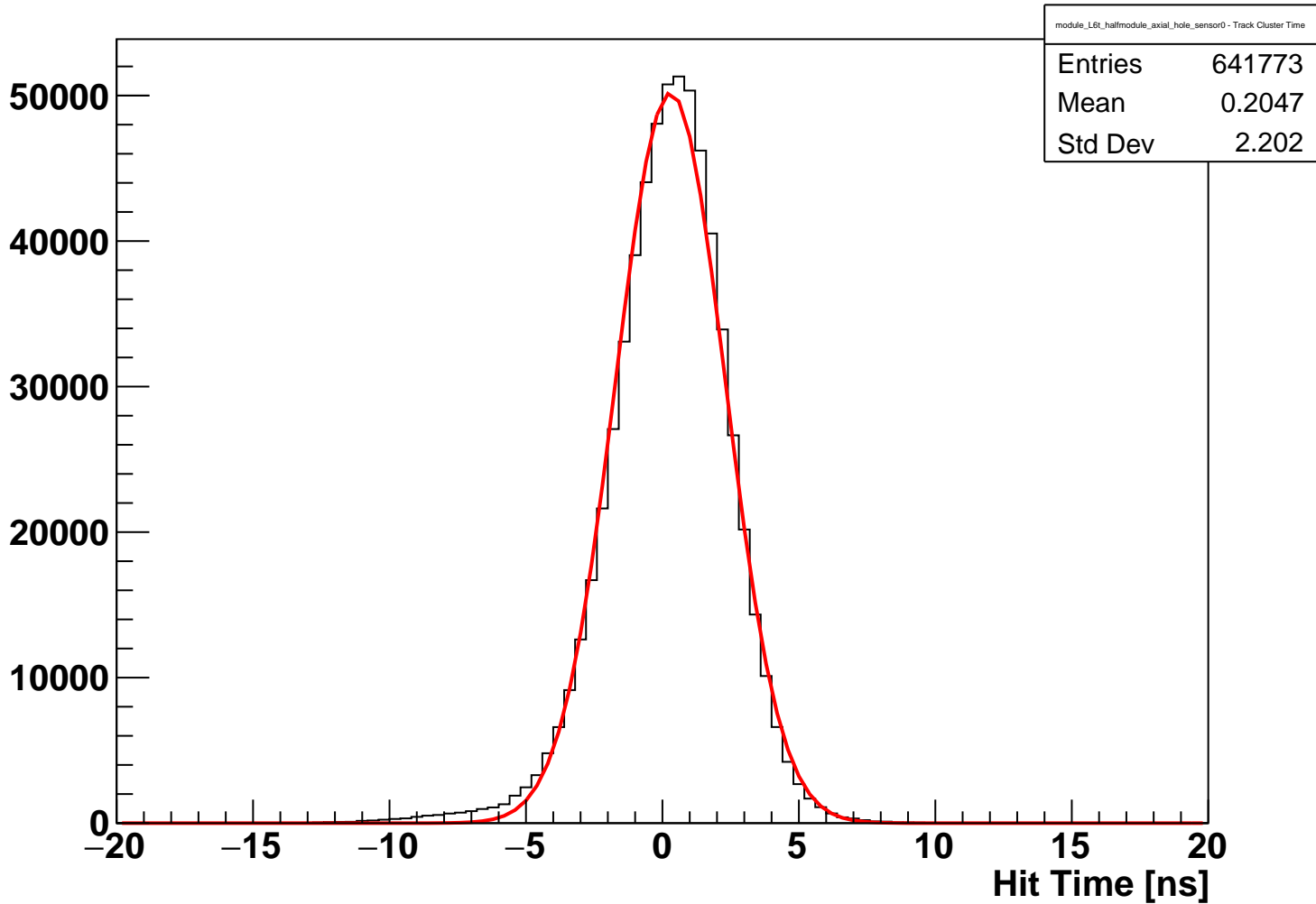
module_L6t_halfmodule_axial_hole_sensor0 Fitted Hit Time (hits on clean track)
