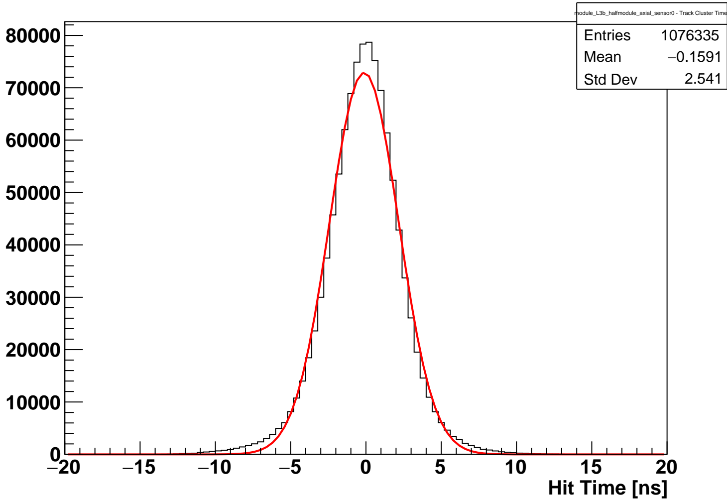
module_L3b_halfmodule_axial_sensor0 Fitted Hit Time (hits on clean track)
