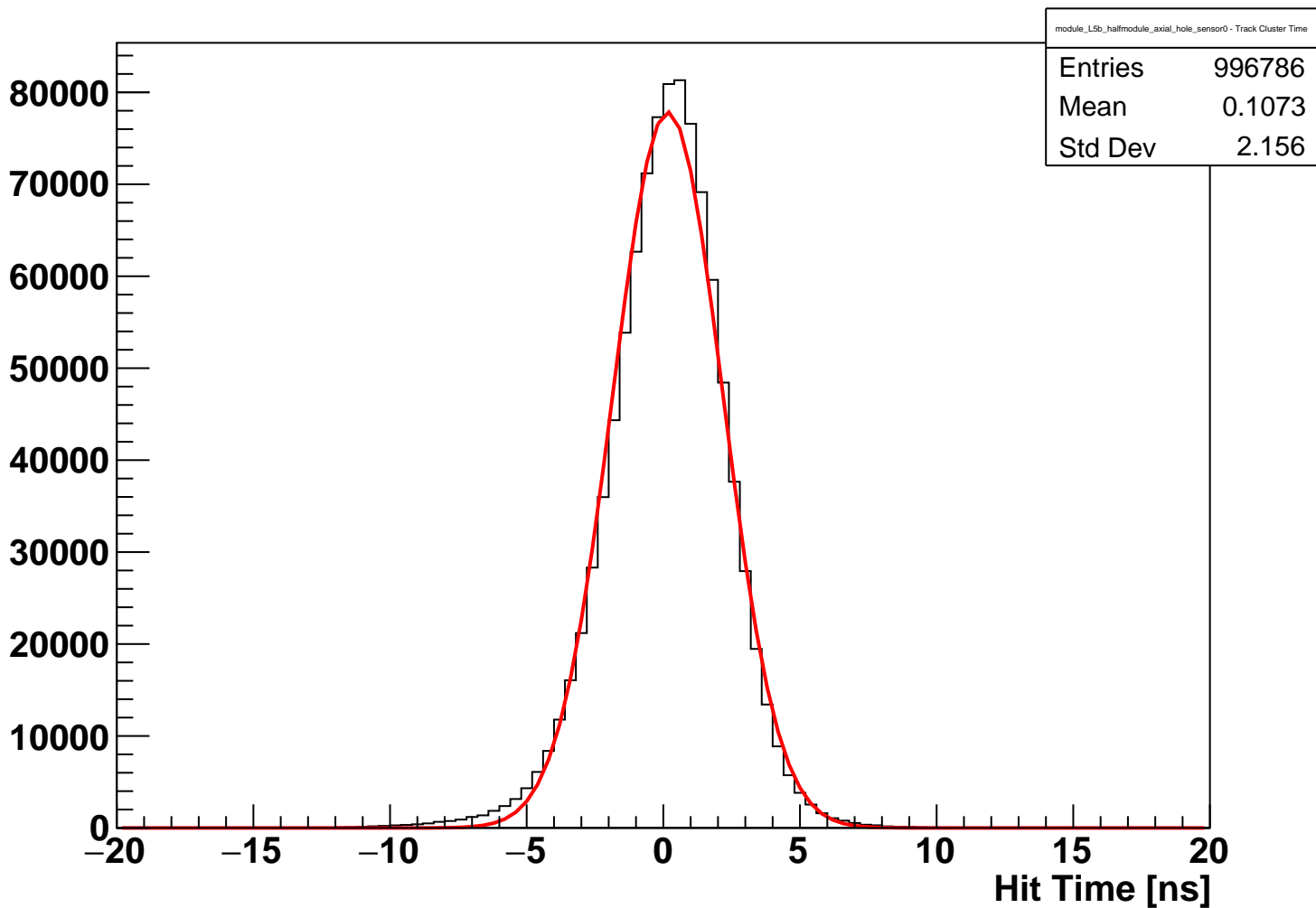
module_L5b_halfmodule_axial_hole_sensor0 Fitted Hit Time (hits on clean track)
