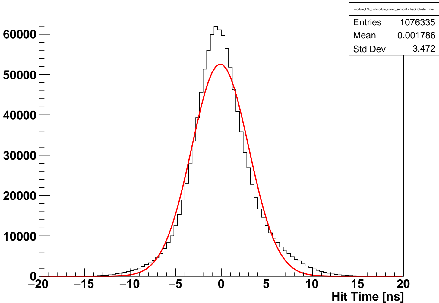
module_L1b_halfmodule_stereo_sensor0 Fitted Hit Time (hits on clean track)
