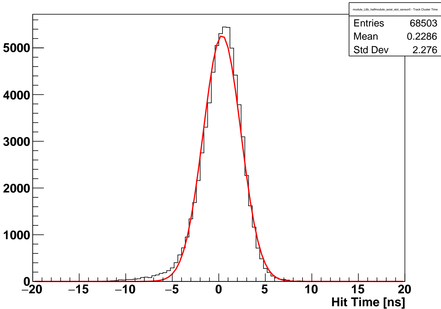
module_L6b_halfmodule_axial_slot_sensor0 Fitted Hit Time (hits on clean track)
