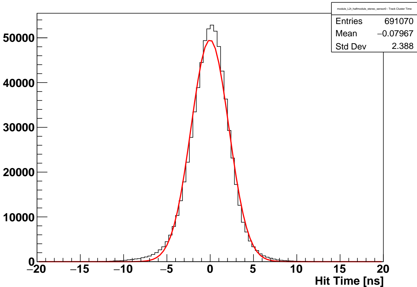
module_L2t_halfmodule_stereo_sensor0 Fitted Hit Time (hits on clean track)
