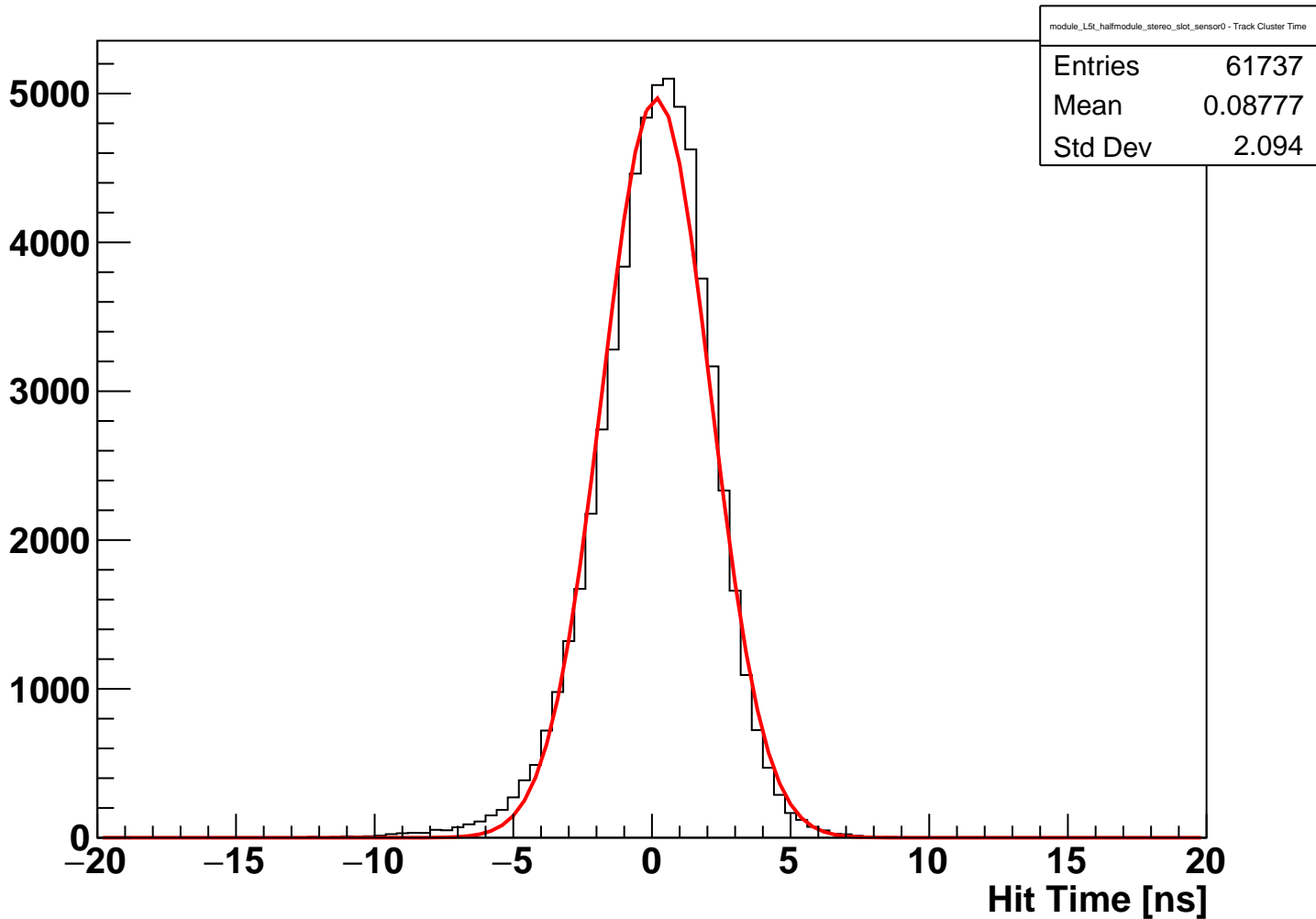
module_L5t_halfmodule_stereo_slot_sensor0 Fitted Hit Time (hits on clean track)
