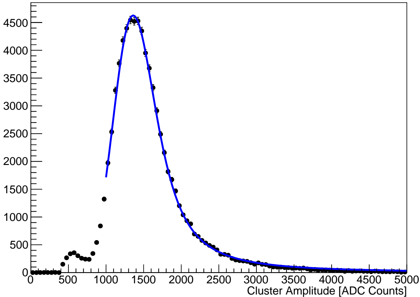
module_L5b_halfmodule_stereo_slot_sensor0 Fitted Cluster Amplitude (hits on clean track)
