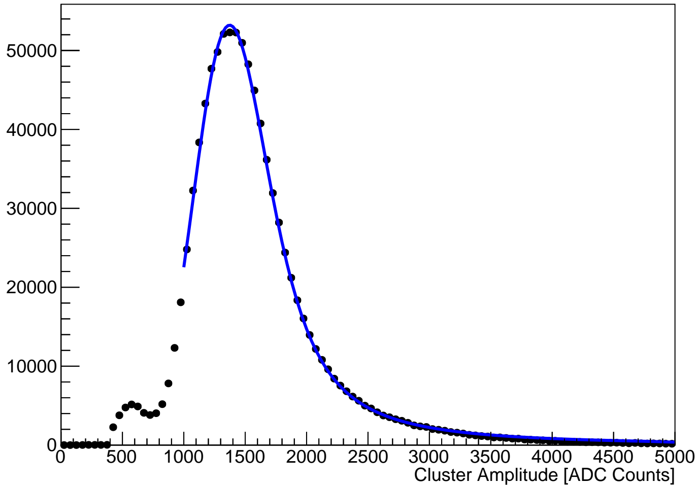
module_L4b_halfmodule_stereo_hole_sensor0 Fitted Cluster Amplitude (hits on clean track)
