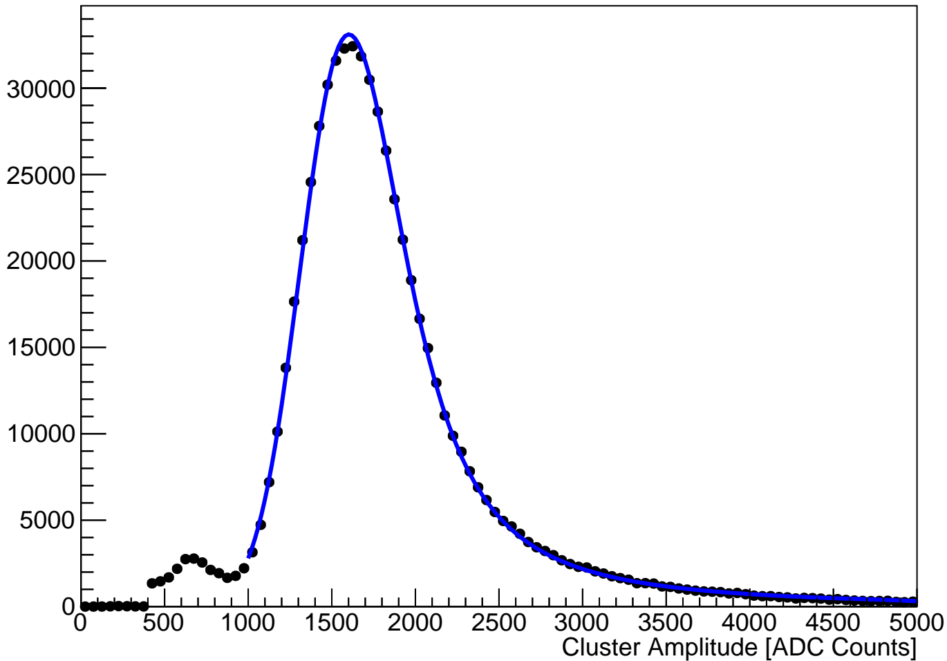
module_L6t_halfmodule_stereo_hole_sensor0 Fitted Cluster Amplitude (hits on clean track)
