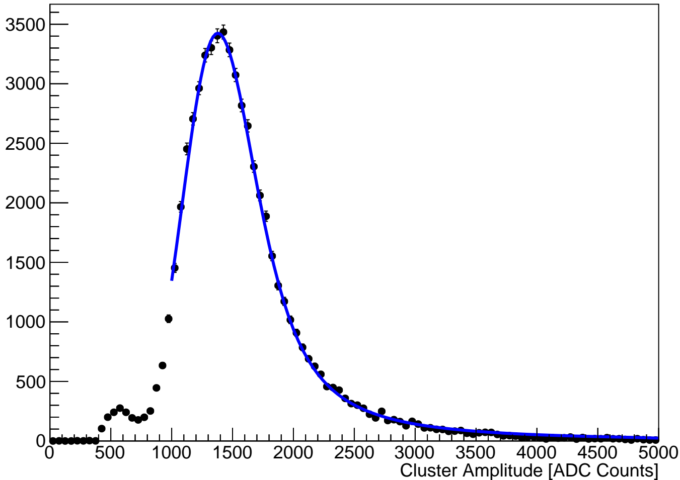
module_L5t_halfmodule_axial_slot_sensor0 Fitted Cluster Amplitude (hits on clean track)
