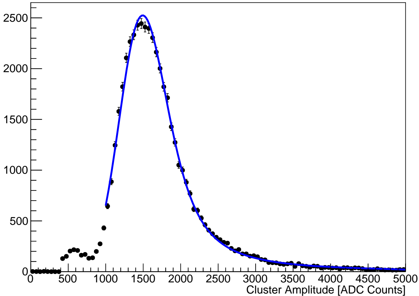
module_L6t_halfmodule_axial_slot_sensor0 Fitted Cluster Amplitude (hits on clean track)
