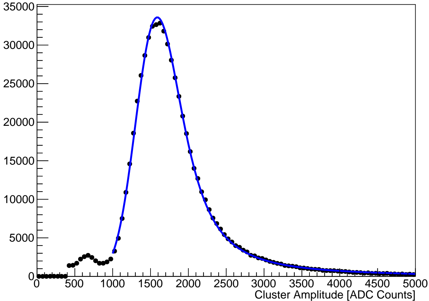
module_L6t_halfmodule_axial_hole_sensor0 Fitted Cluster Amplitude (hits on clean track)
