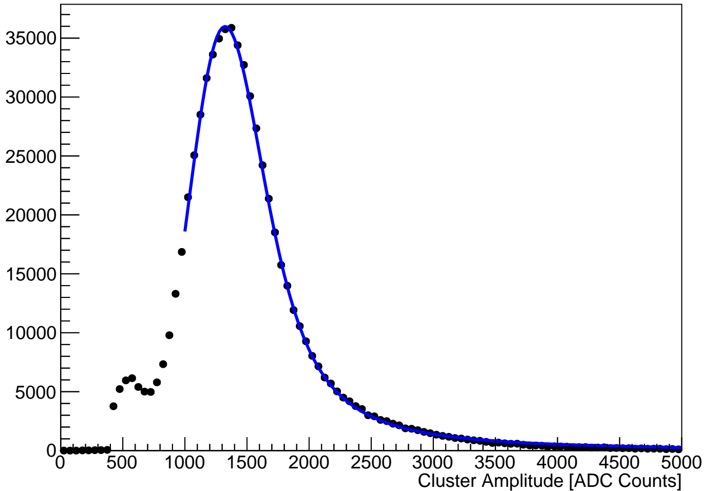
module_L2t_halfmodule_axial_sensor0 Fitted Cluster Amplitude (hits on clean track)
