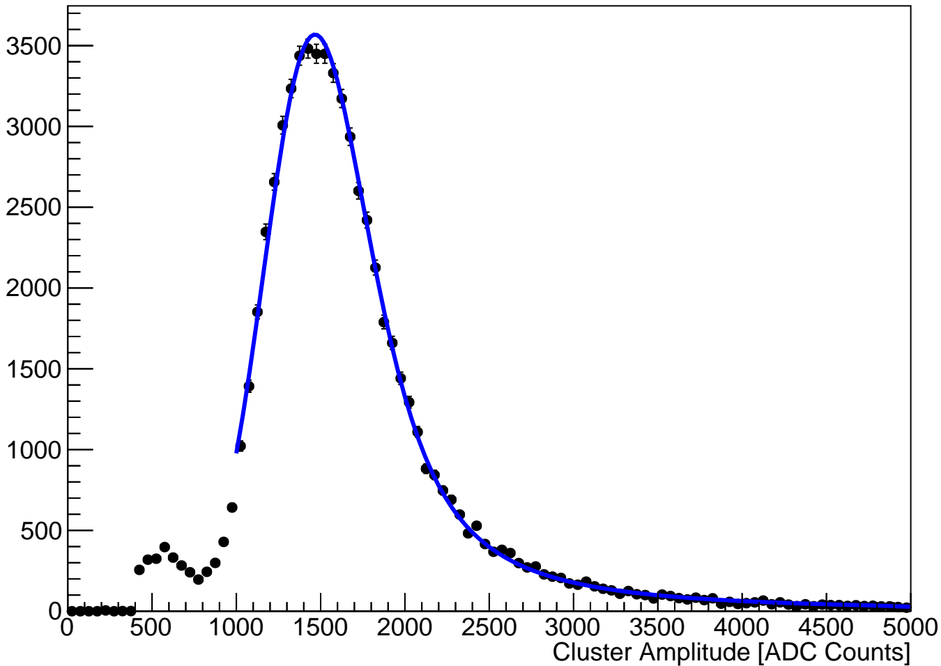
module_L6b_halfmodule_axial_slot_sensor0 Fitted Cluster Amplitude (hits on clean track)
