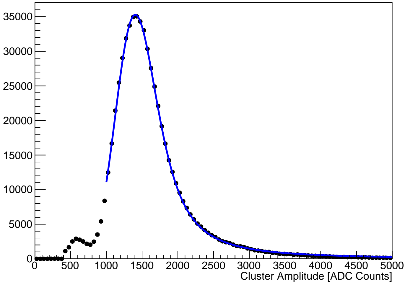
module_L5t_halfmodule_stereo_hole_sensor0 Fitted Cluster Amplitude (hits on clean track)
