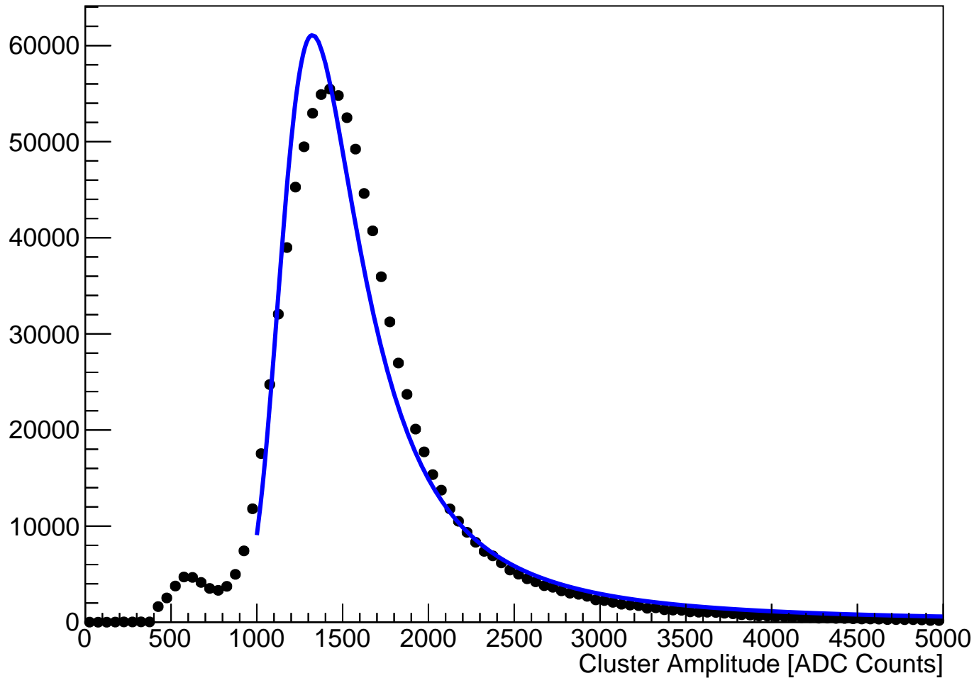
module_L5b_halfmodule_stereo_hole_sensor0 Fitted Cluster Amplitude (hits on clean track)
