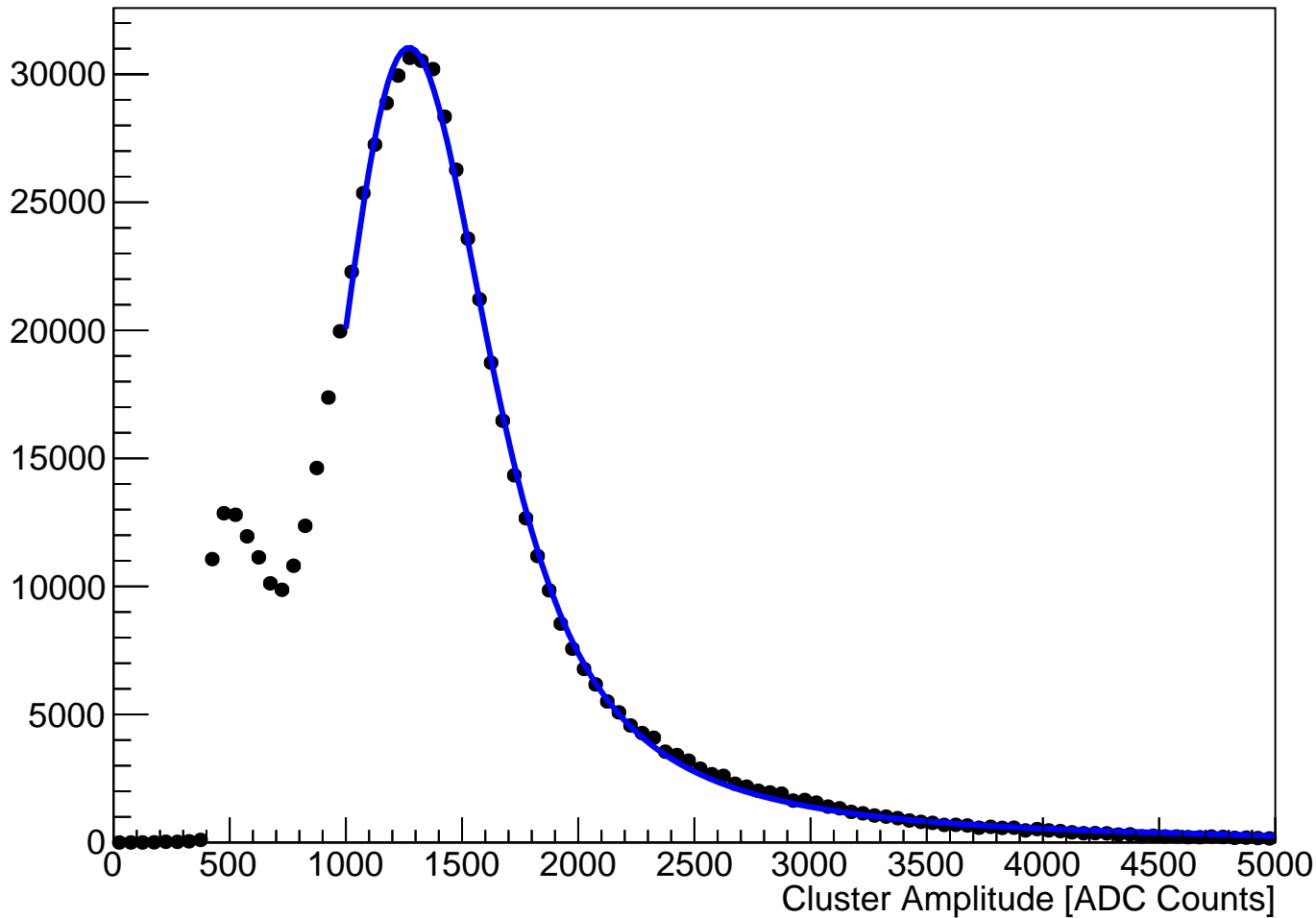
module_L1t_halfmodule_axial_sensor0 Fitted Cluster Amplitude (hits on clean track)
