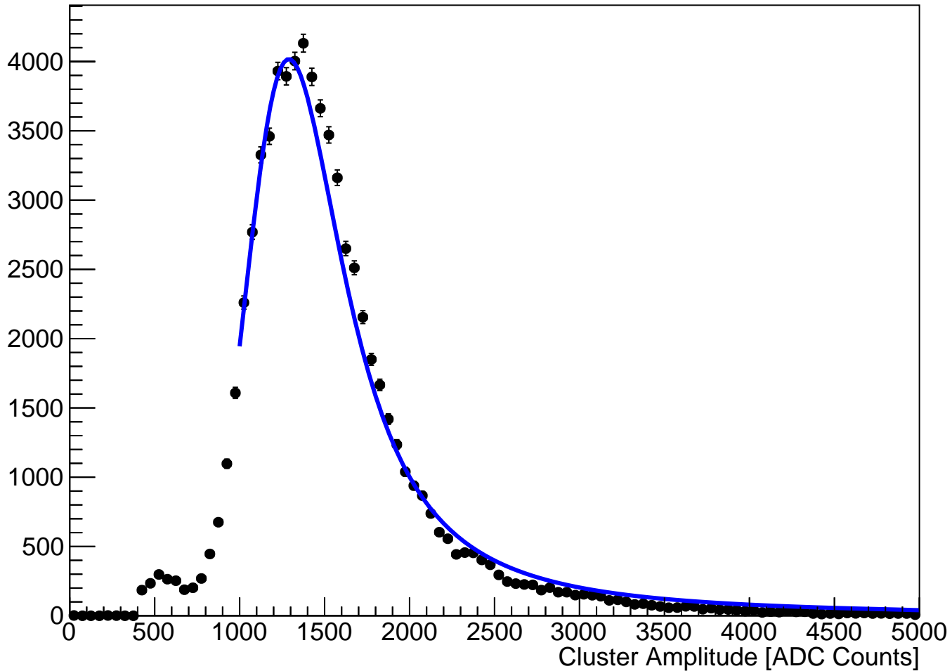
module_L4t_halfmodule_stereo_slot_sensor0 Fitted Cluster Amplitude (hits on clean track)
