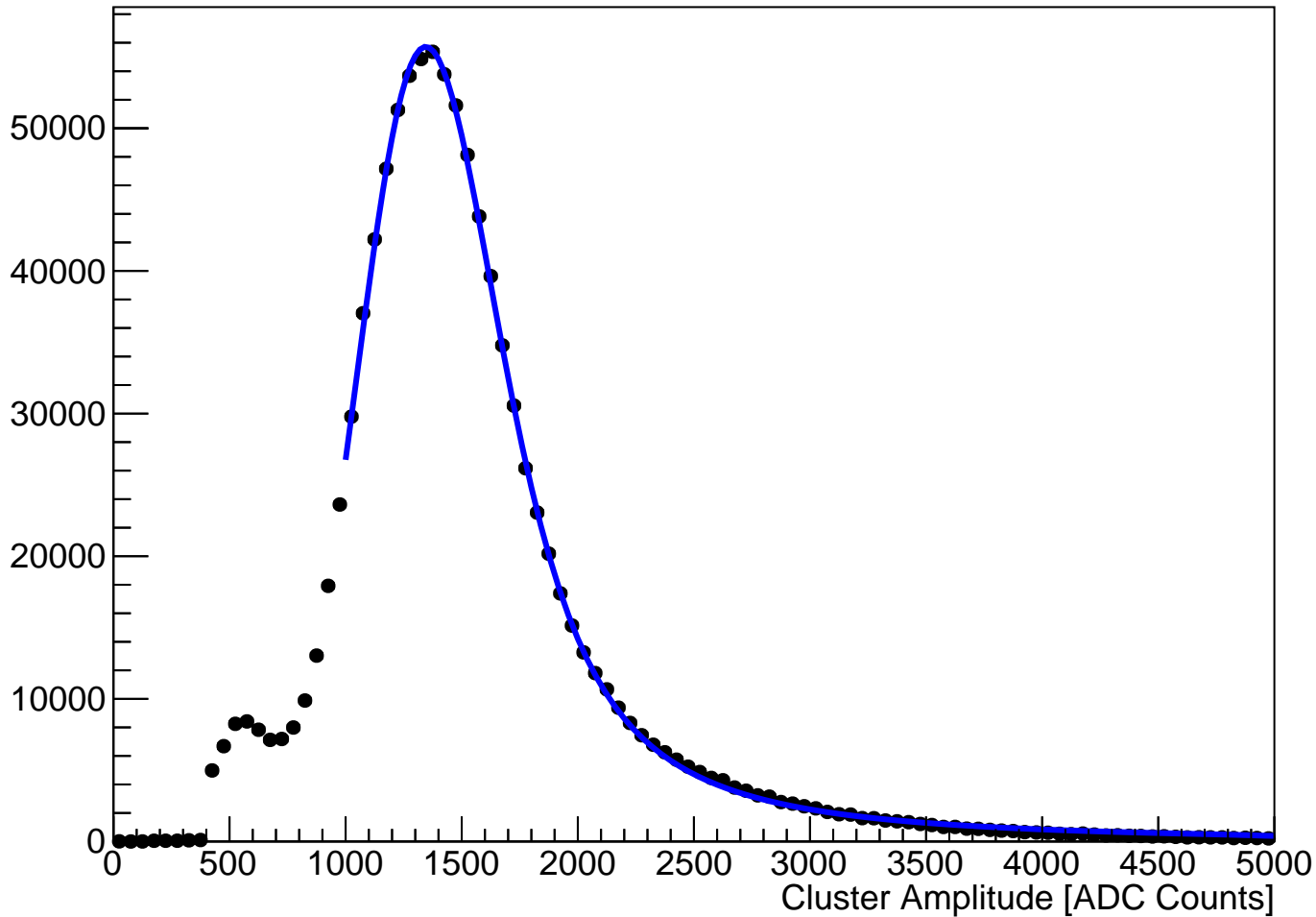
module_L2b_halfmodule_stereo_sensor0 Fitted Cluster Amplitude (hits on clean track)
