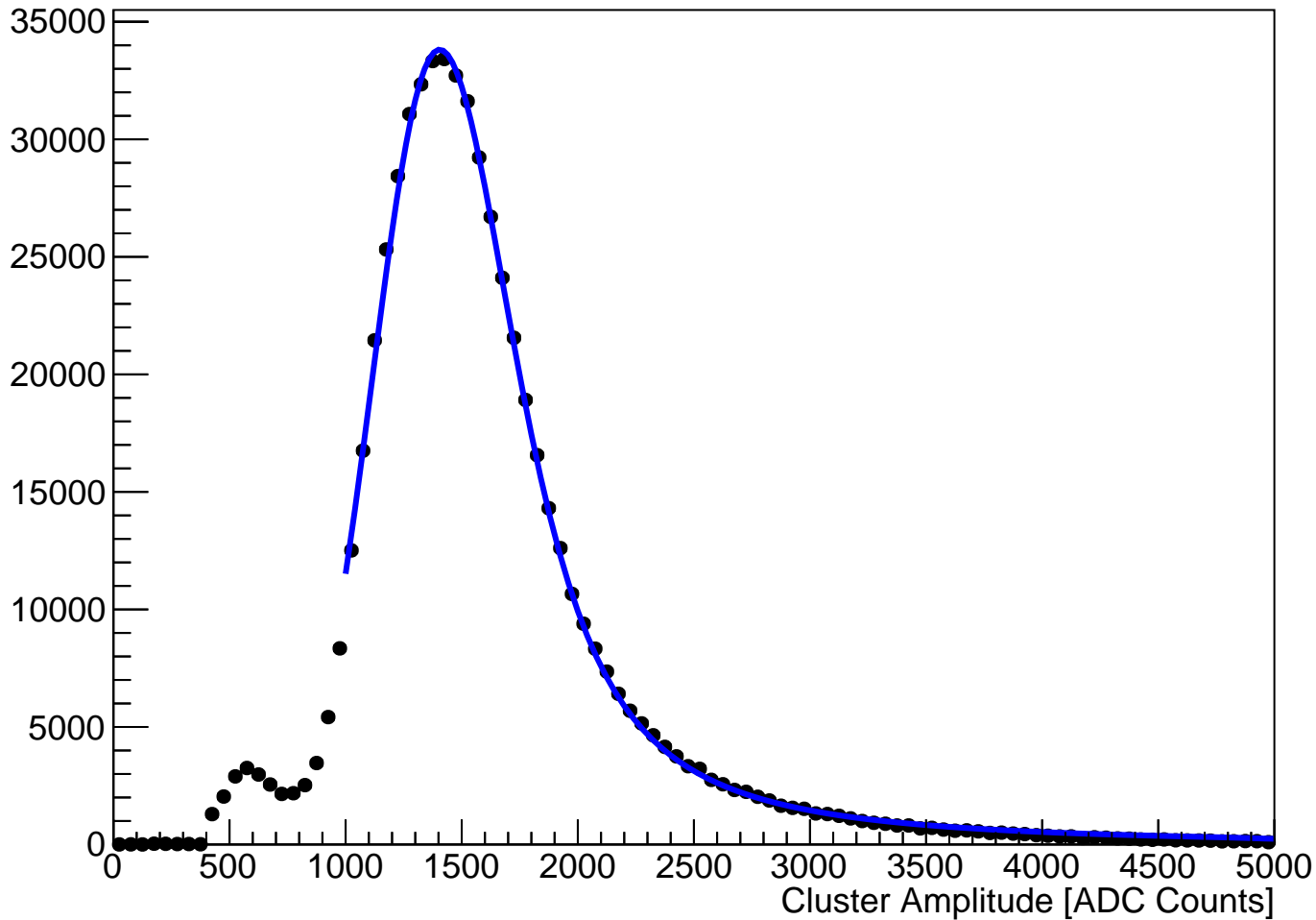
module_L4t_halfmodule_stereo_hole_sensor0 Fitted Cluster Amplitude (hits on clean track)
