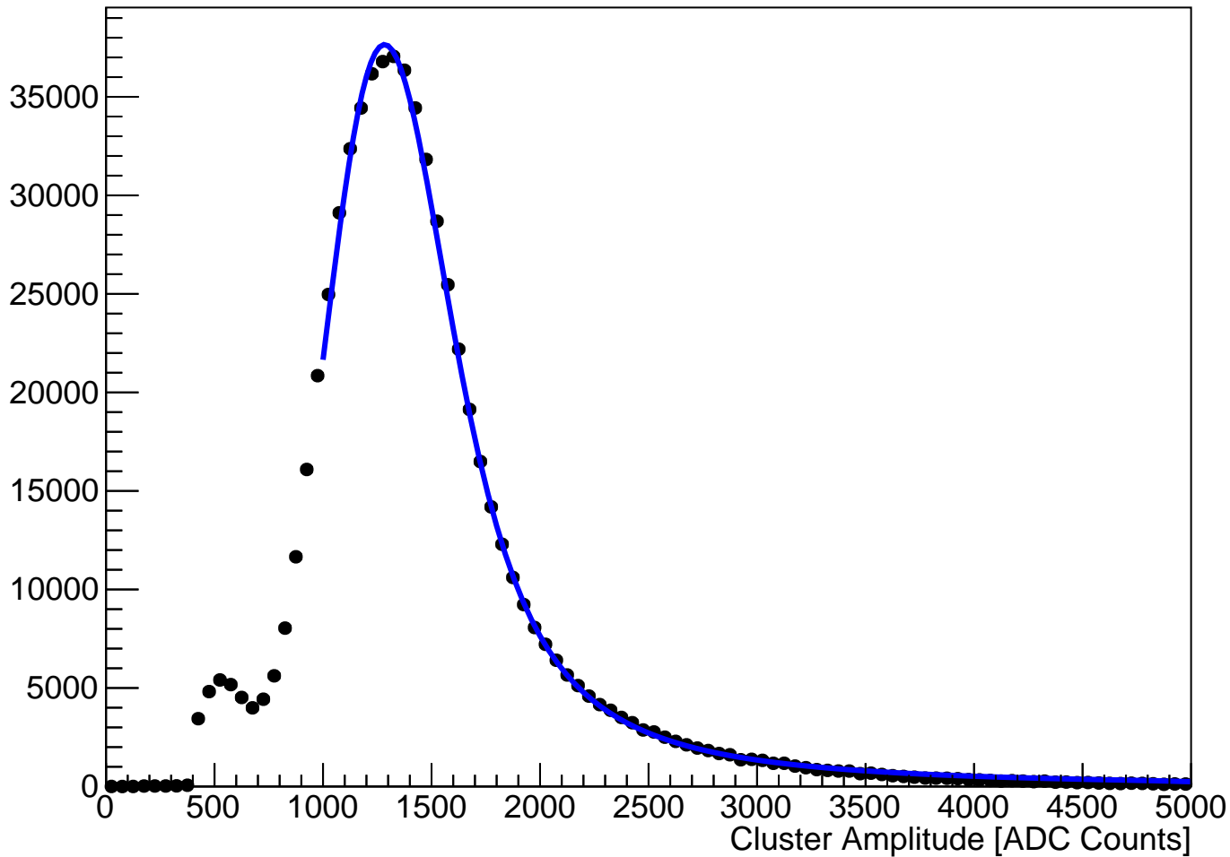
module_L2t_halfmodule_stereo_sensor0 Fitted Cluster Amplitude (hits on clean track)
