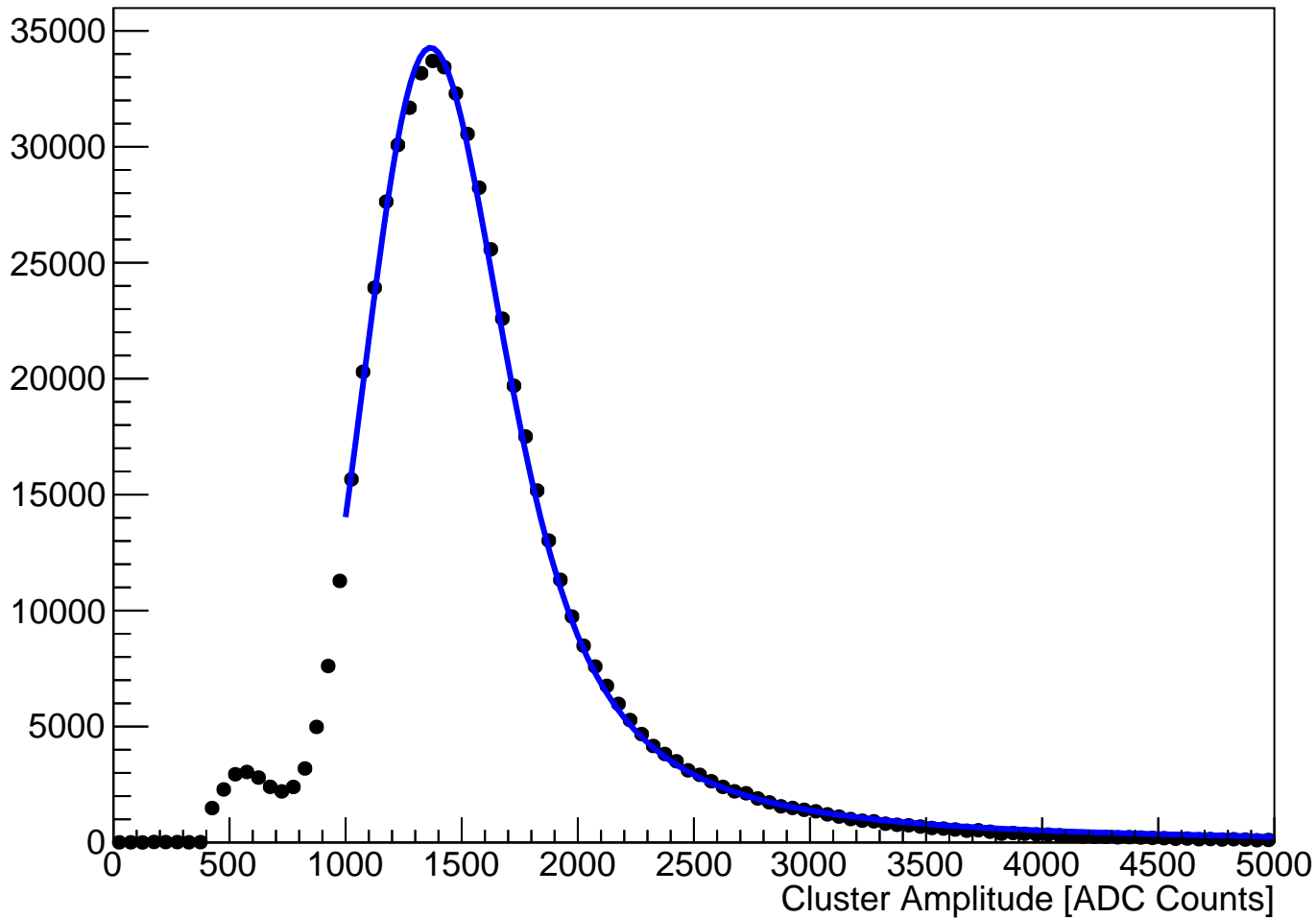
module_L4t_halfmodule_axial_hole_sensor0 Fitted Cluster Amplitude (hits on clean track)
