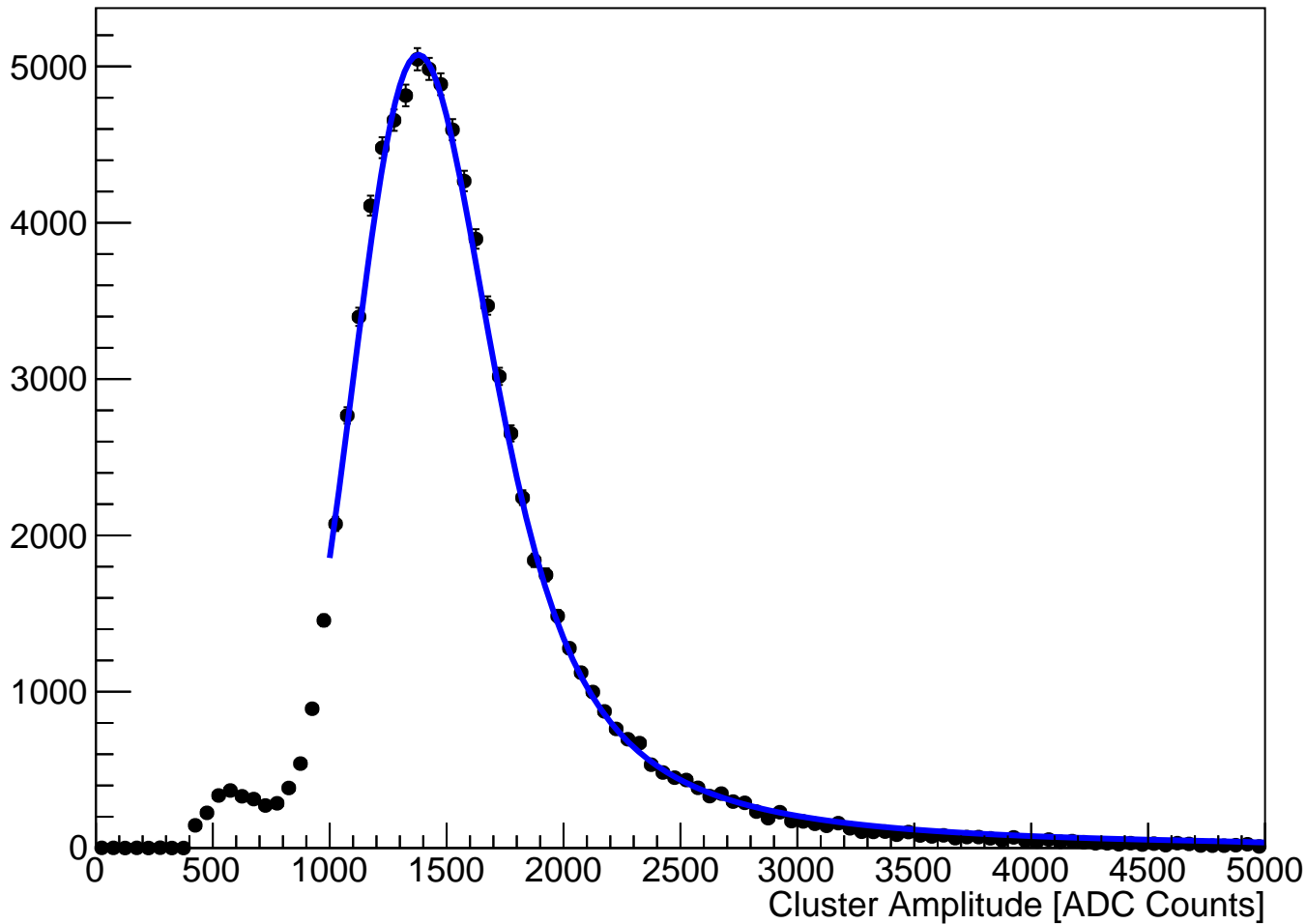
module_L4b_halfmodule_stereo_slot_sensor0 Fitted Cluster Amplitude (hits on clean track)
