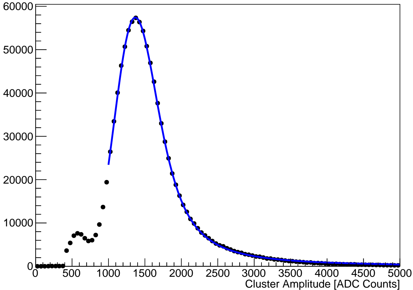
module_L3b_halfmodule_stereo_sensor0 Fitted Cluster Amplitude (hits on clean track)
