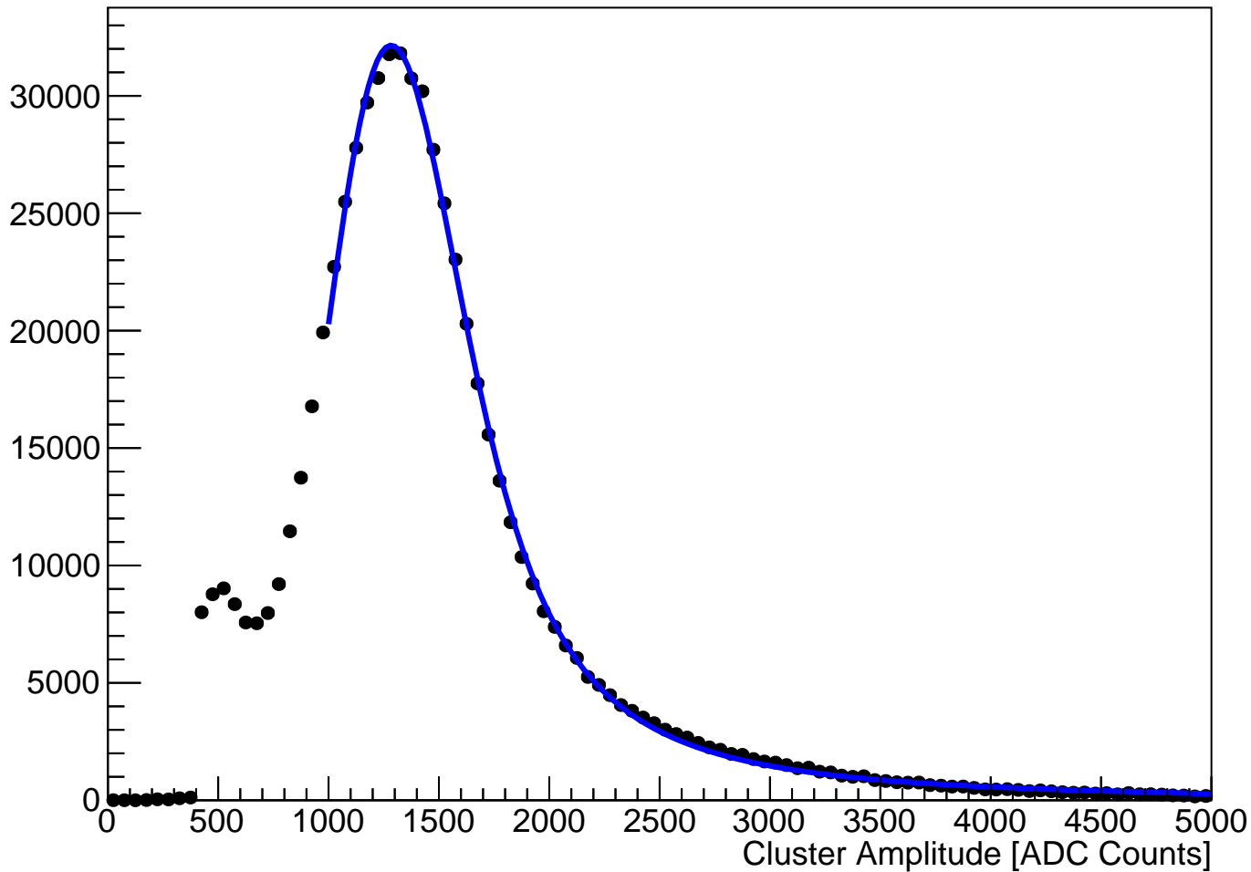
module_L1t_halfmodule_stereo_sensor0 Fitted Cluster Amplitude (hits on clean track)
