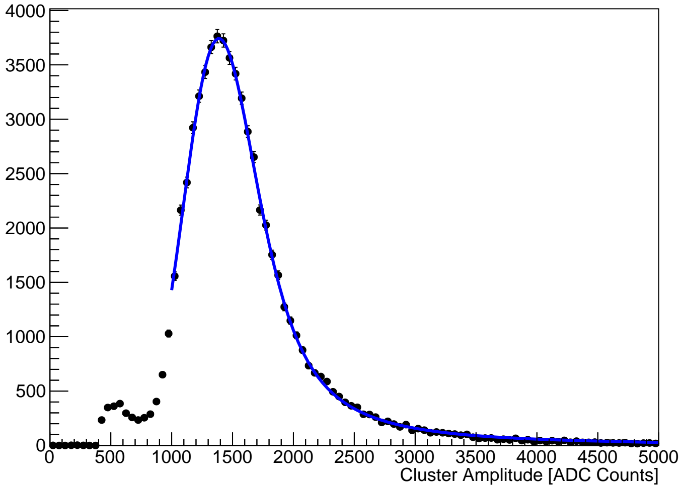
module_L6b_halfmodule_stereo_slot_sensor0 Fitted Cluster Amplitude (hits on clean track)
