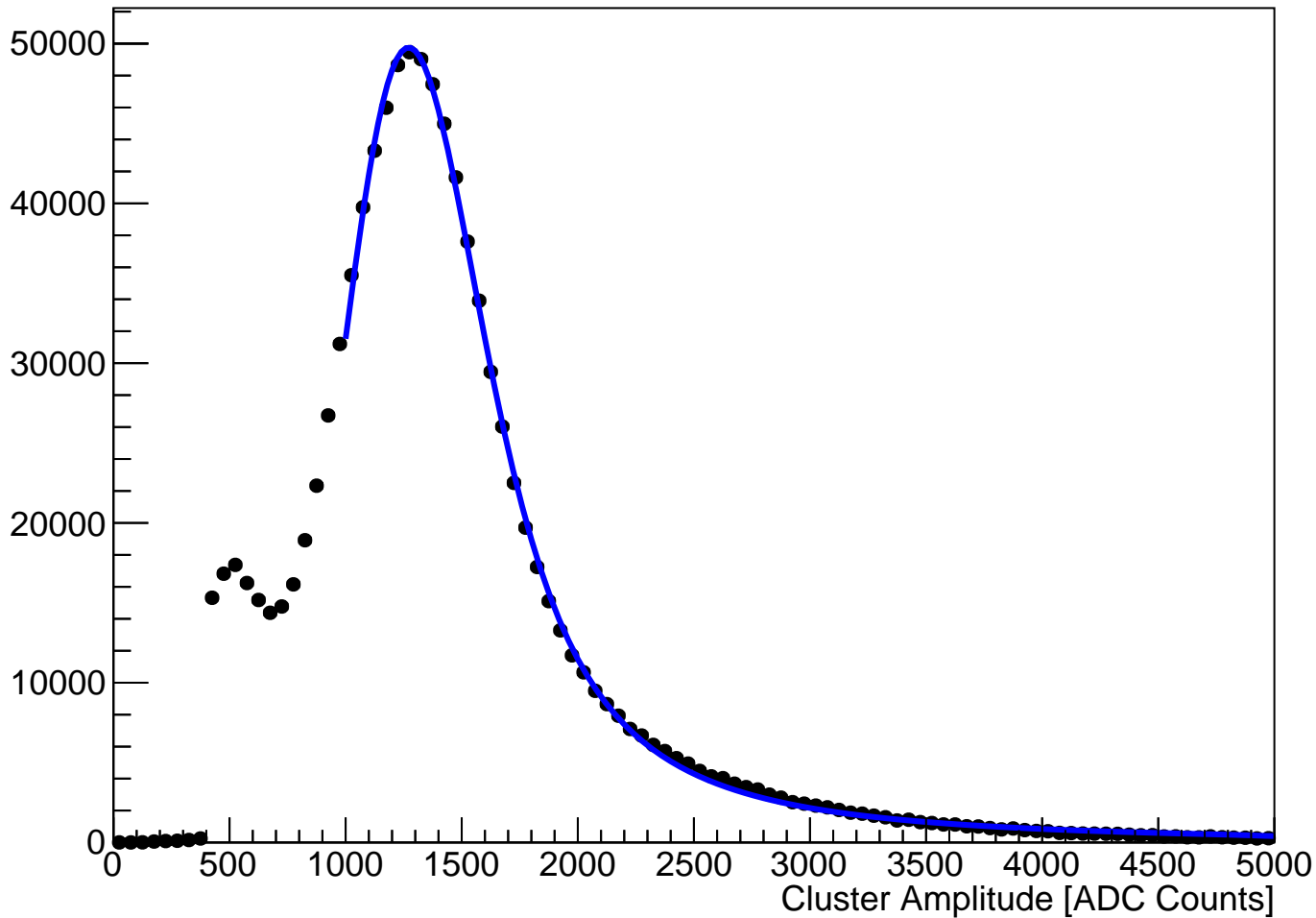
module_L1b_halfmodule_stereo_sensor0 Fitted Cluster Amplitude (hits on clean track)
