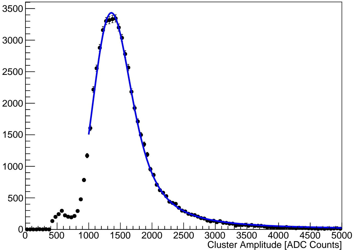
module_L5t_halfmodule_stereo_slot_sensor0 Fitted Cluster Amplitude (hits on clean track)
