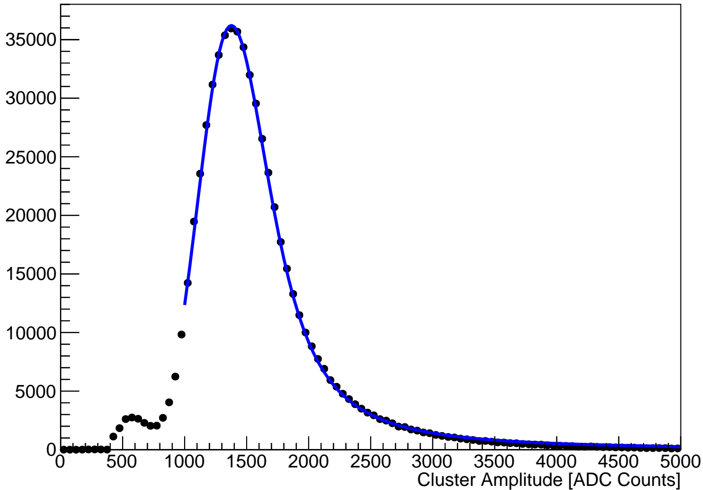
module_L5t_halfmodule_axial_hole_sensor0 Fitted Cluster Amplitude (hits on clean track)
