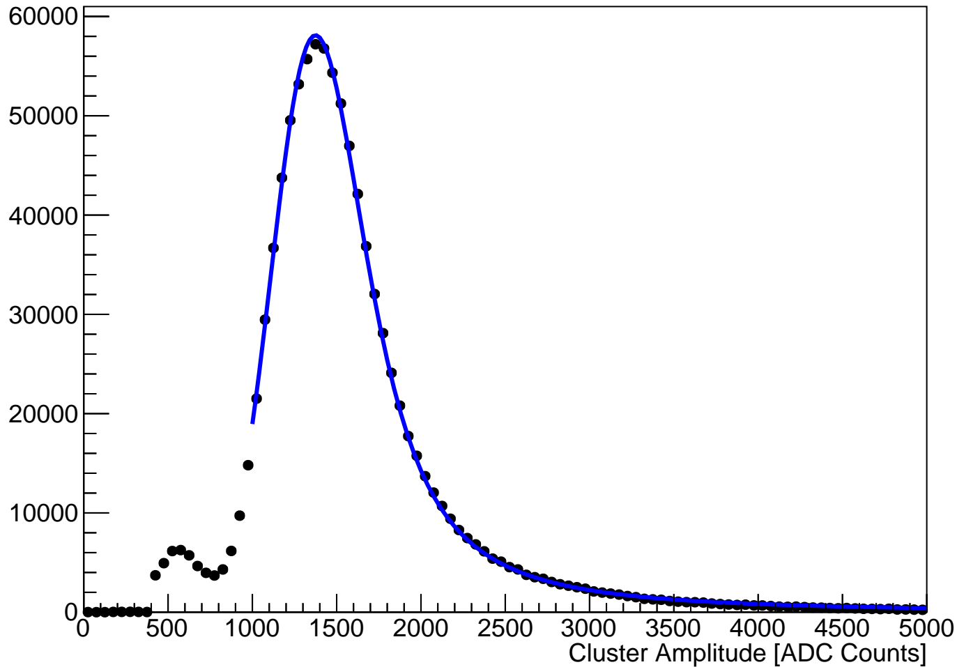
module_L6b_halfmodule_stereo_hole_sensor0 Fitted Cluster Amplitude (hits on clean track)
