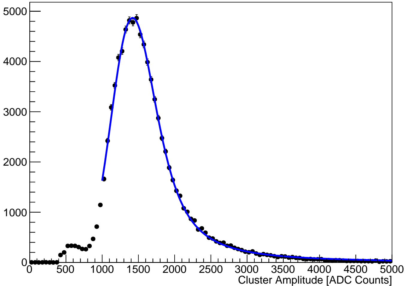
module_L4b_halfmodule_axial_slot_sensor0 Fitted Cluster Amplitude (hits on clean track)
