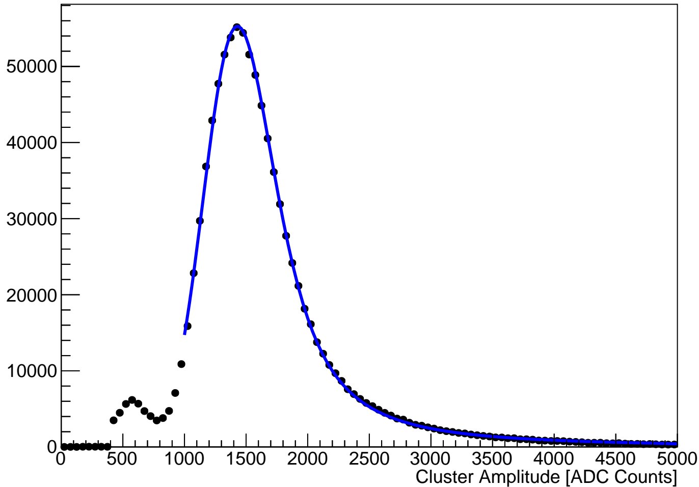
module_L6b_halfmodule_axial_hole_sensor0 Fitted Cluster Amplitude (hits on clean track)
