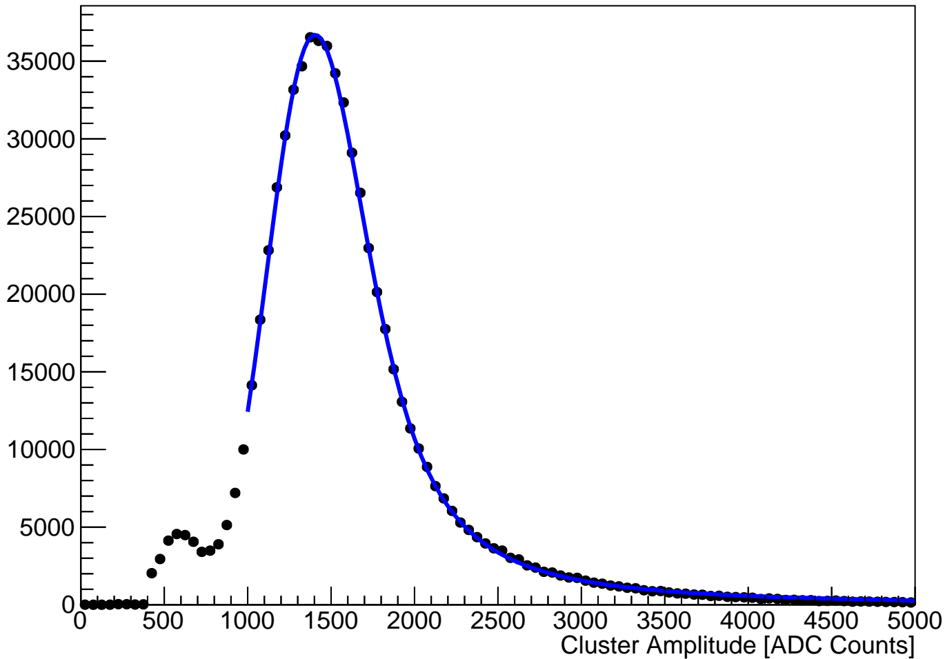
module_L3t_halfmodule_stereo_sensor0 Fitted Cluster Amplitude (hits on clean track)
