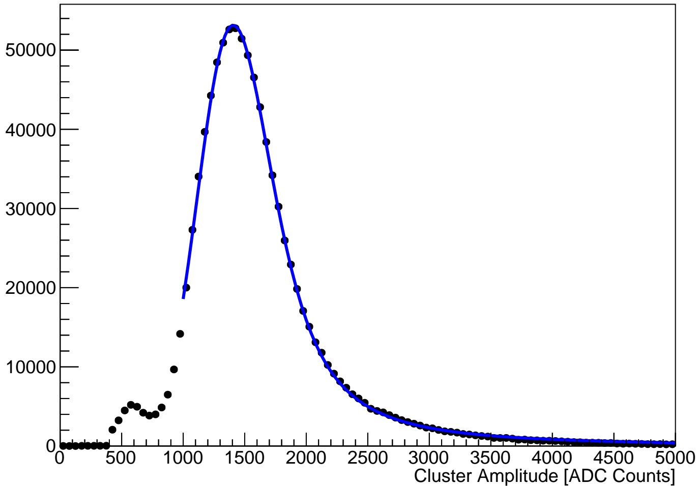
module_L4b_halfmodule_axial_hole_sensor0 Fitted Cluster Amplitude (hits on clean track)
