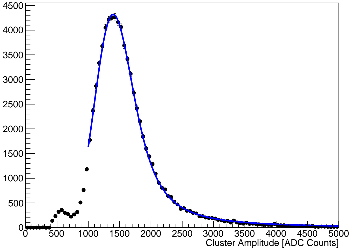
module_L5b_halfmodule_axial_slot_sensor0 Fitted Cluster Amplitude (hits on clean track)
