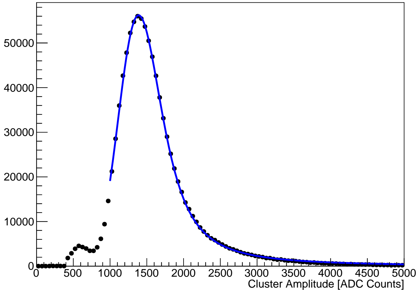
module_L5b_halfmodule_axial_hole_sensor0 Fitted Cluster Amplitude (hits on clean track)
