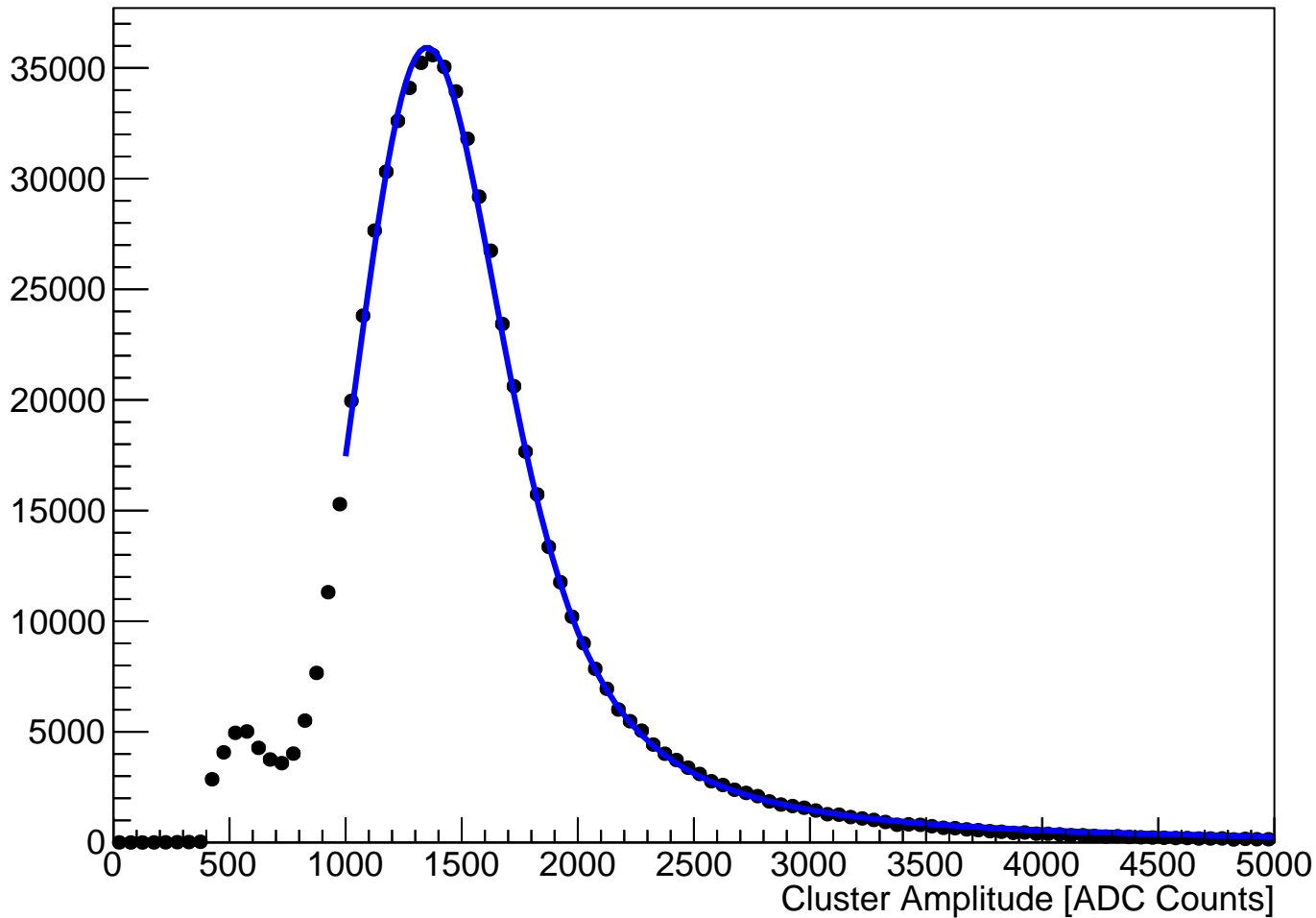
module_L3t_halfmodule_axial_sensor0 Fitted Cluster Amplitude (hits on clean track)
