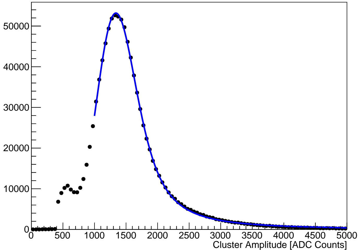
module_L2b_halfmodule_axial_sensor0 Fitted Cluster Amplitude (hits on clean track)
