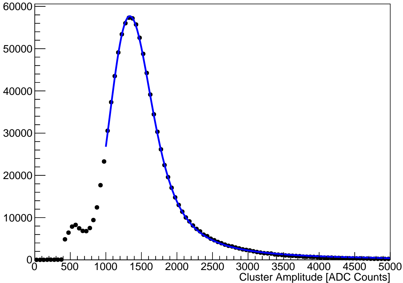
module_L3b_halfmodule_axial_sensor0 Fitted Cluster Amplitude (hits on clean track)
