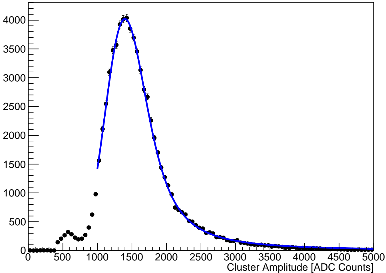
module_L4t_halfmodule_axial_slot_sensor0 Fitted Cluster Amplitude (hits on clean track)
