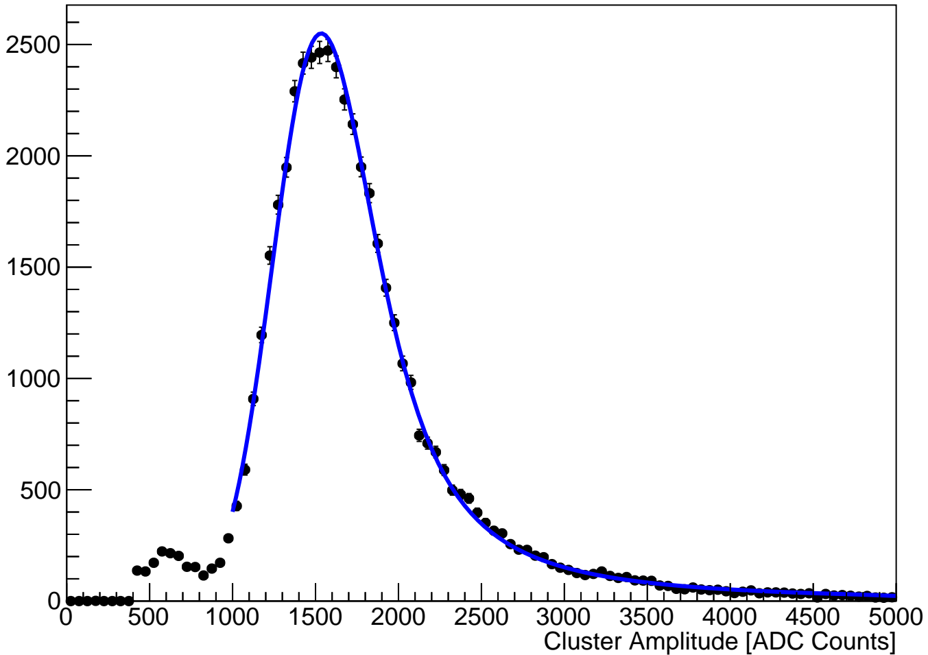
module_L6t_halfmodule_stereo_slot_sensor0 Fitted Cluster Amplitude (hits on clean track)
