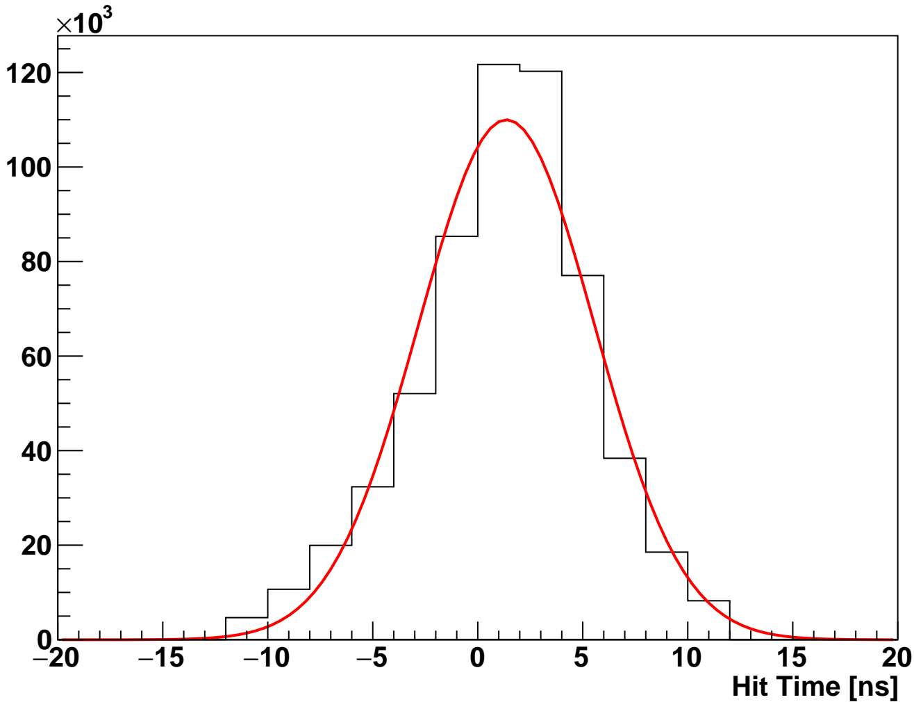
module_L2b_halfmodule_stereo_sensor0 Fitted Hit Time (hits on clean track)
