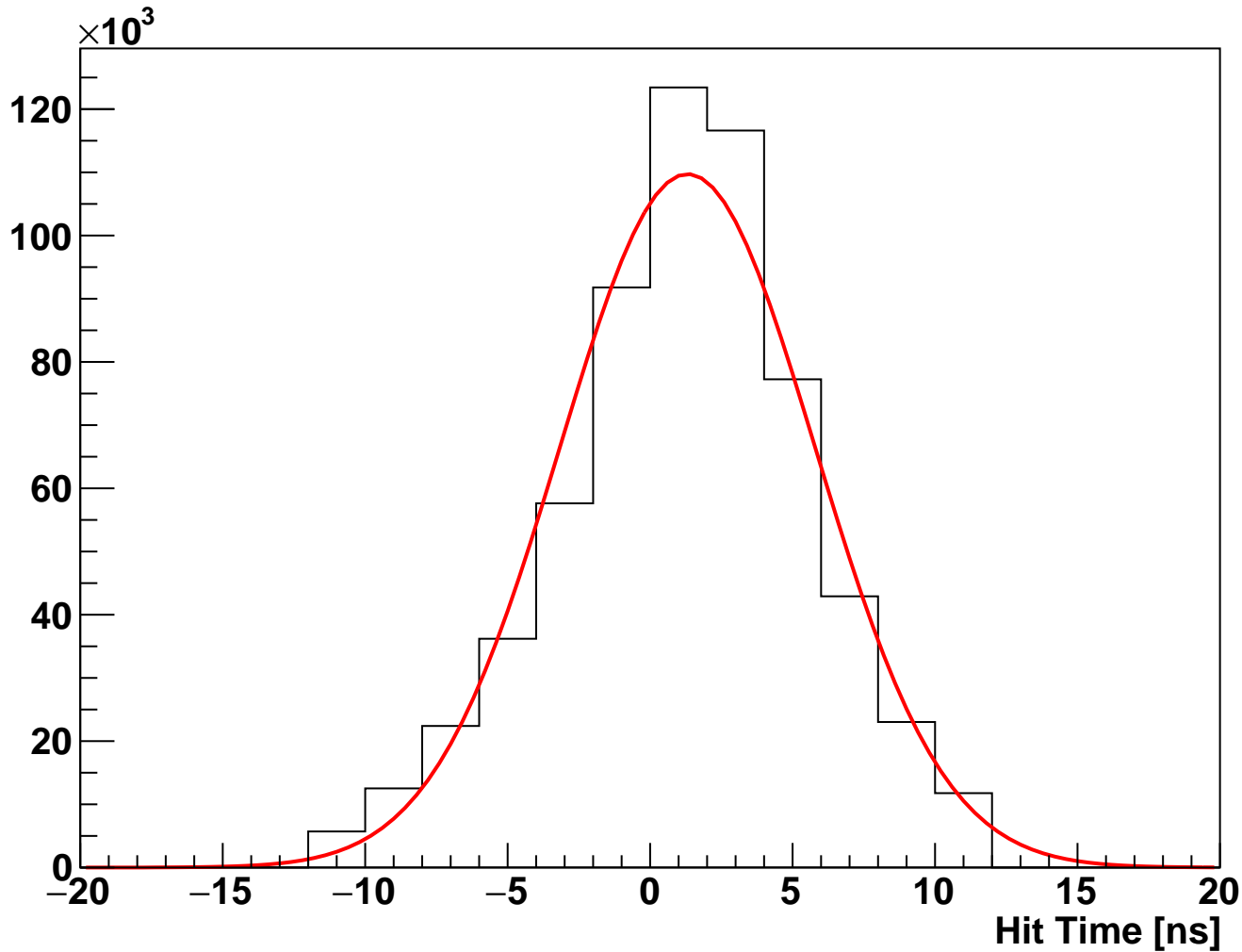
module_L2b_halfmodule_axial_sensor0 Fitted Hit Time (hits on clean track)
