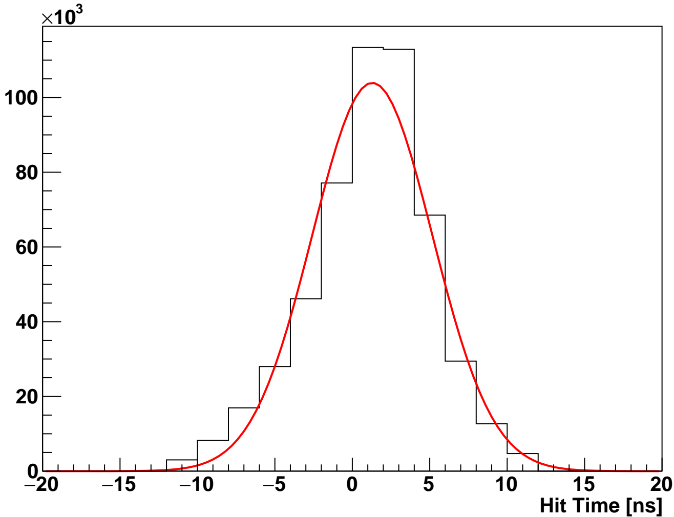
module_L4b_halfmodule_stereo_hole_sensor0 Fitted Hit Time (hits on clean track)
