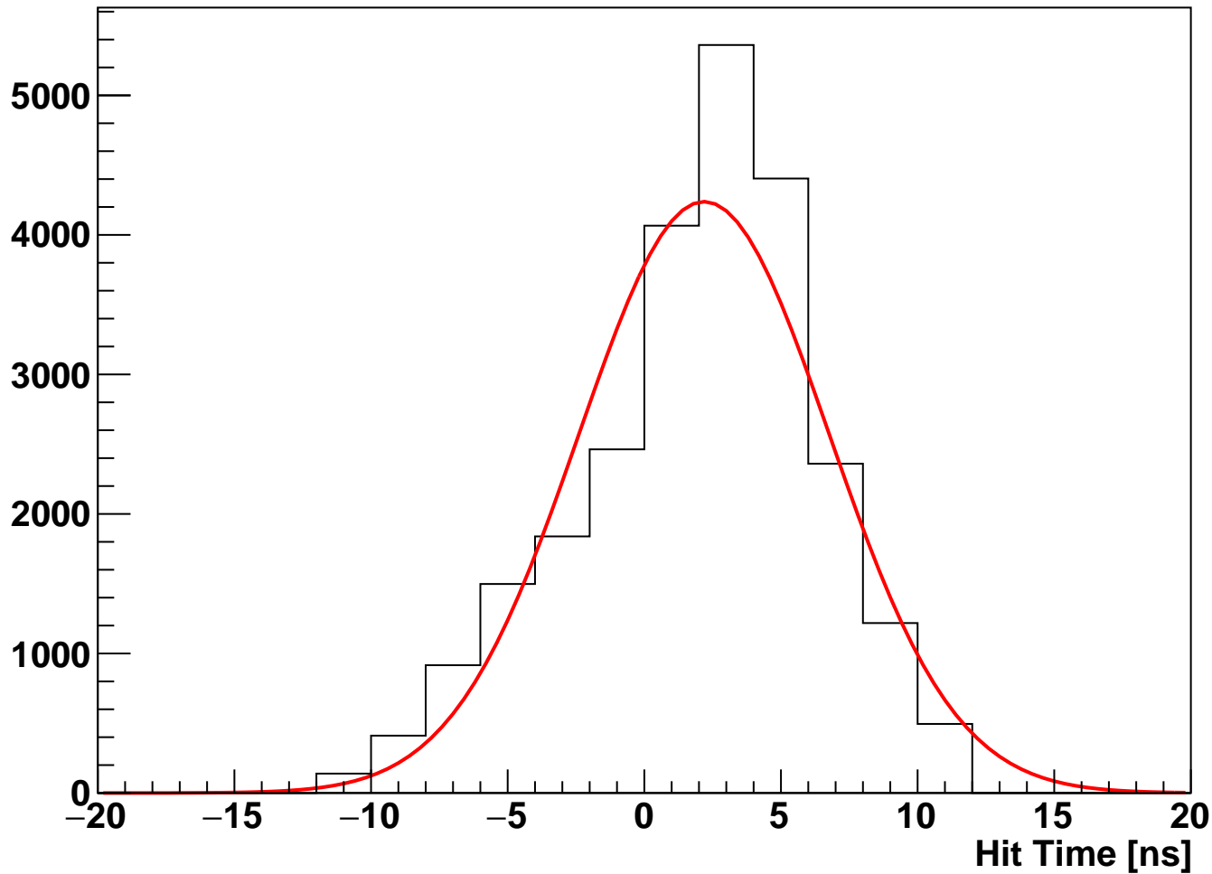
module_L6t_halfmodule_axial_slot_sensor0 Fitted Hit Time (hits on clean track)
