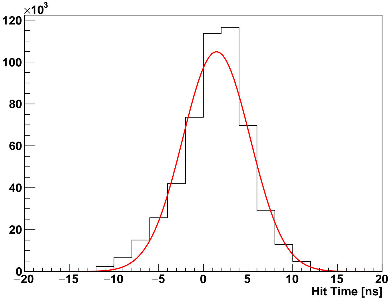
module_L5b_halfmodule_stereo_hole_sensor0 Fitted Hit Time (hits on clean track)
