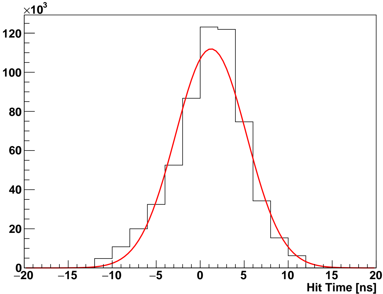
module_L3b_halfmodule_stereo_sensor0 Fitted Hit Time (hits on clean track)
