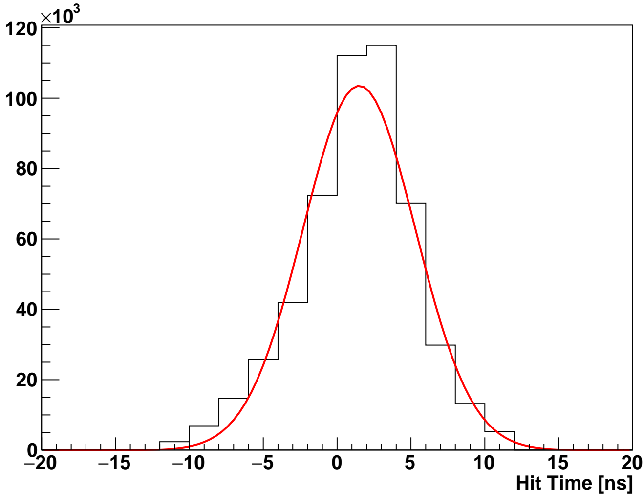
module_L5b_halfmodule_axial_hole_sensor0 Fitted Hit Time (hits on clean track)
