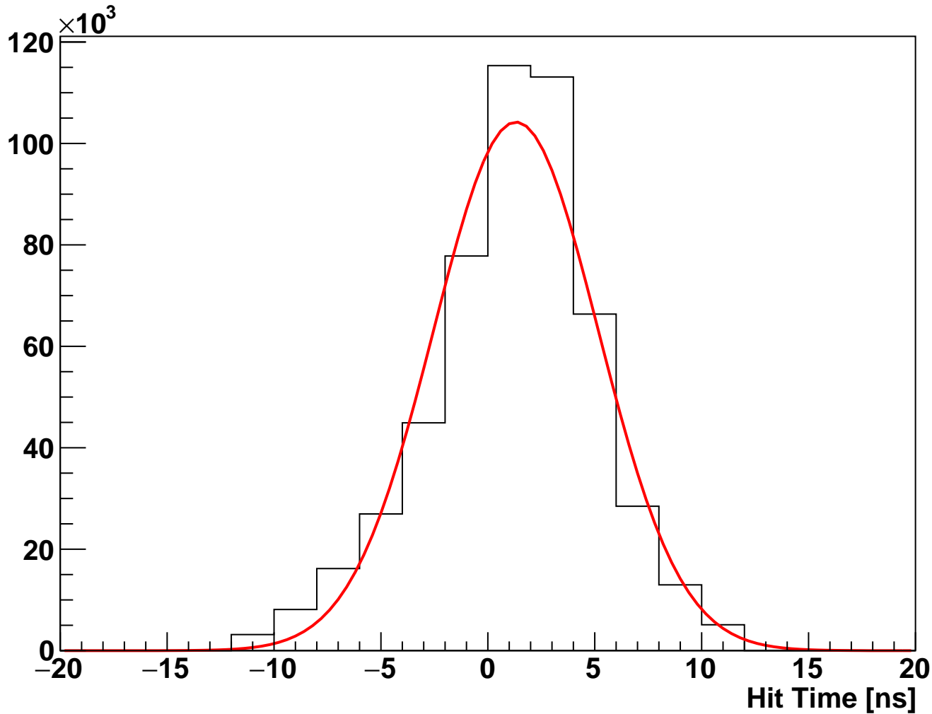
module_L4b_halfmodule_axial_hole_sensor0 Fitted Hit Time (hits on clean track)
