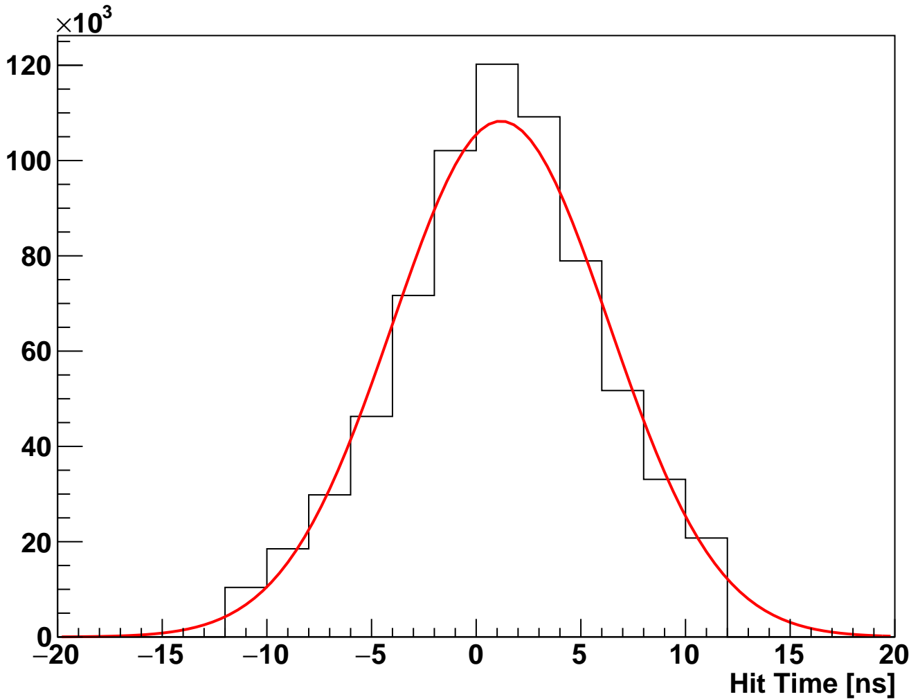
module_L1b_halfmodule_axial_sensor0 Fitted Hit Time (hits on clean track)
