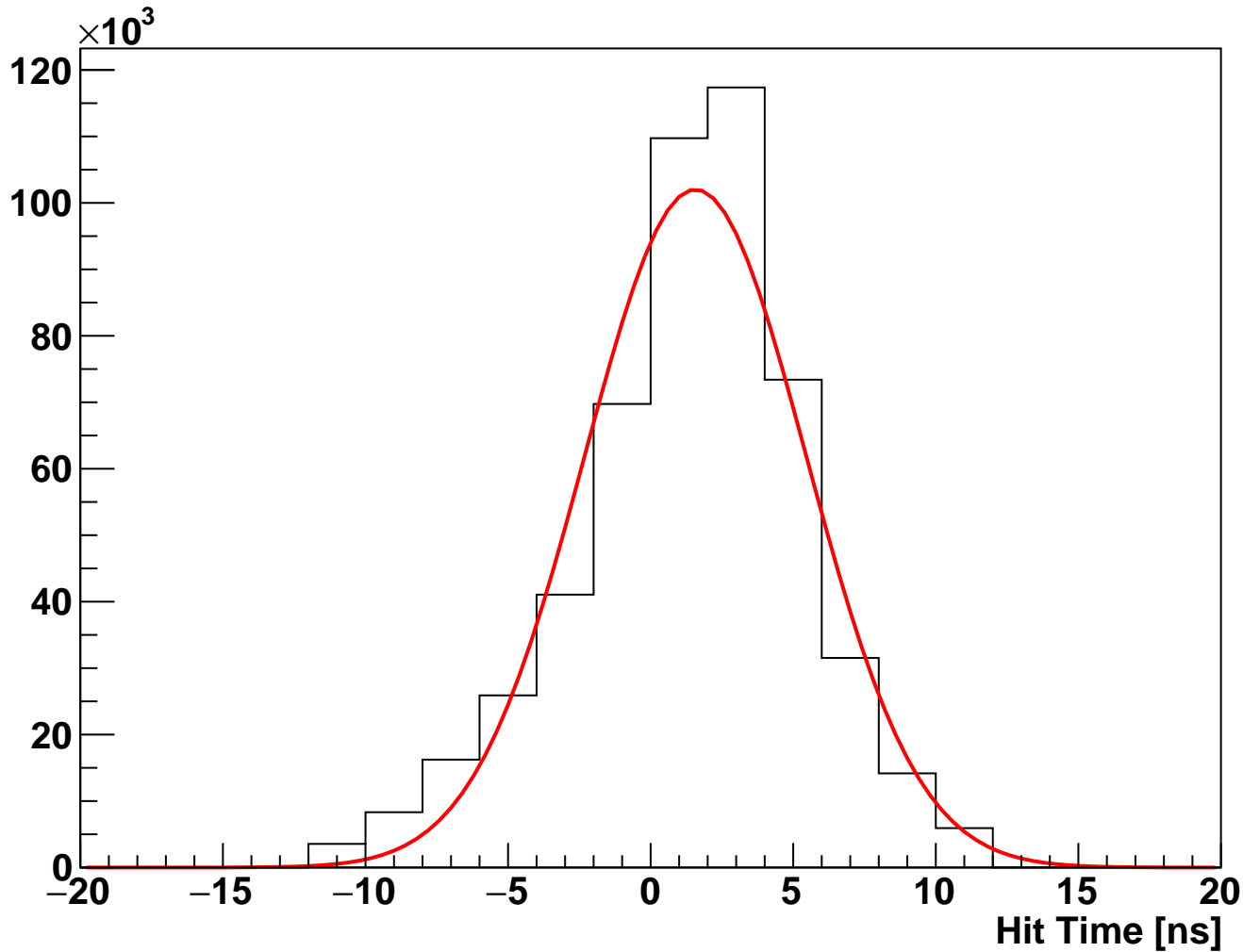
module_L6b_halfmodule_axial_hole_sensor0 Fitted Hit Time (hits on clean track)
