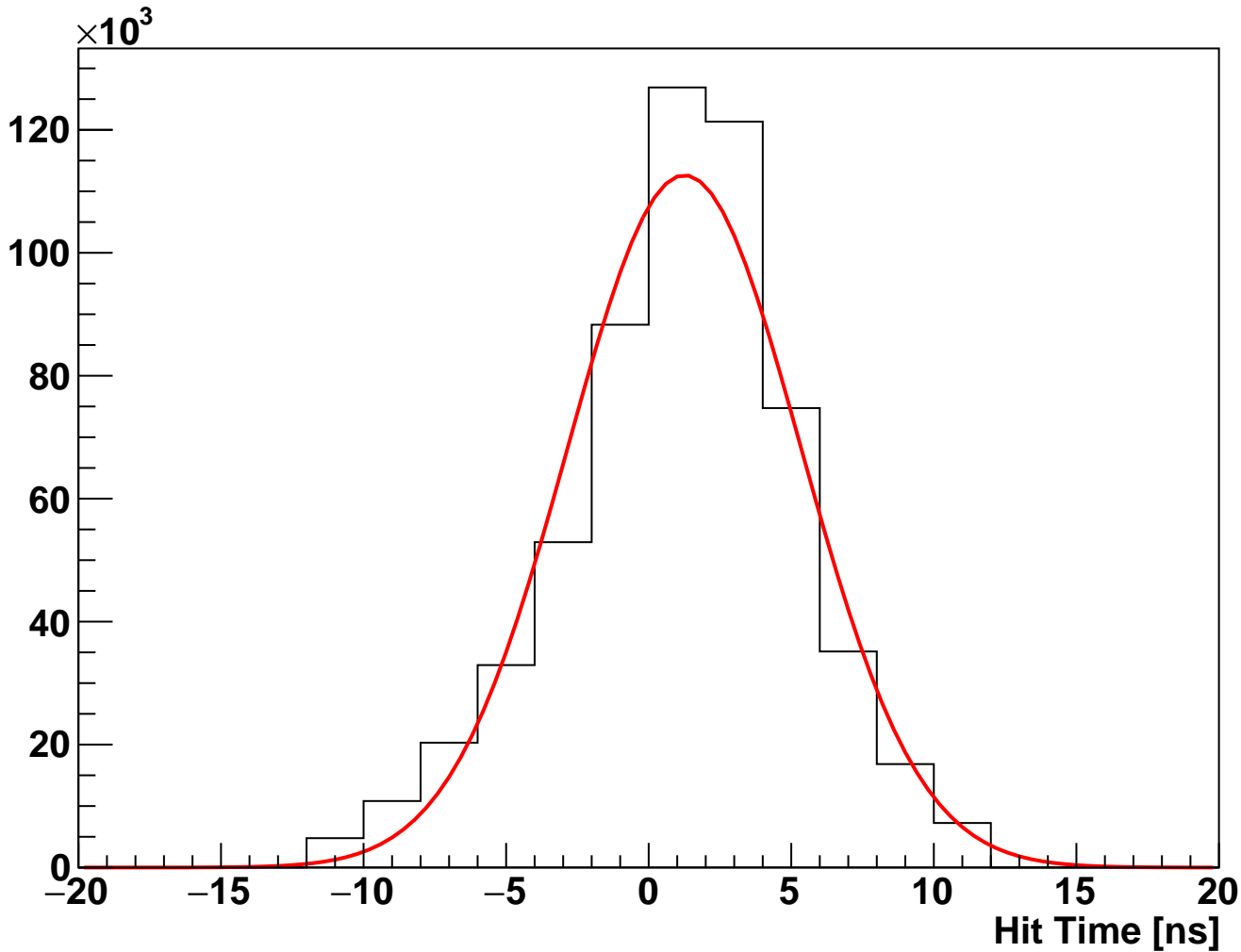
module_L3b_halfmodule_axial_sensor0 Fitted Hit Time (hits on clean track)
