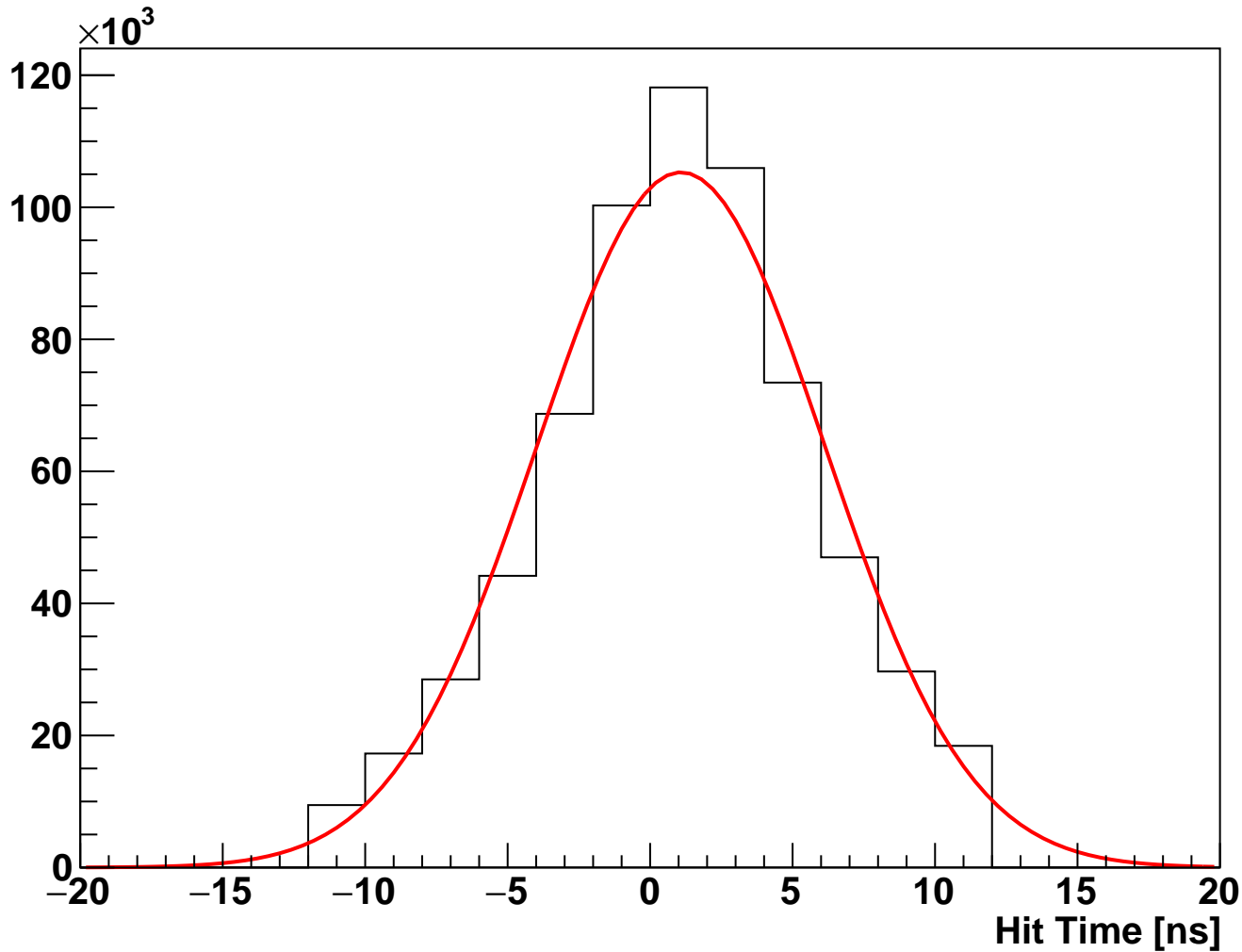
module_L1b_halfmodule_stereo_sensor0 Fitted Hit Time (hits on clean track)
