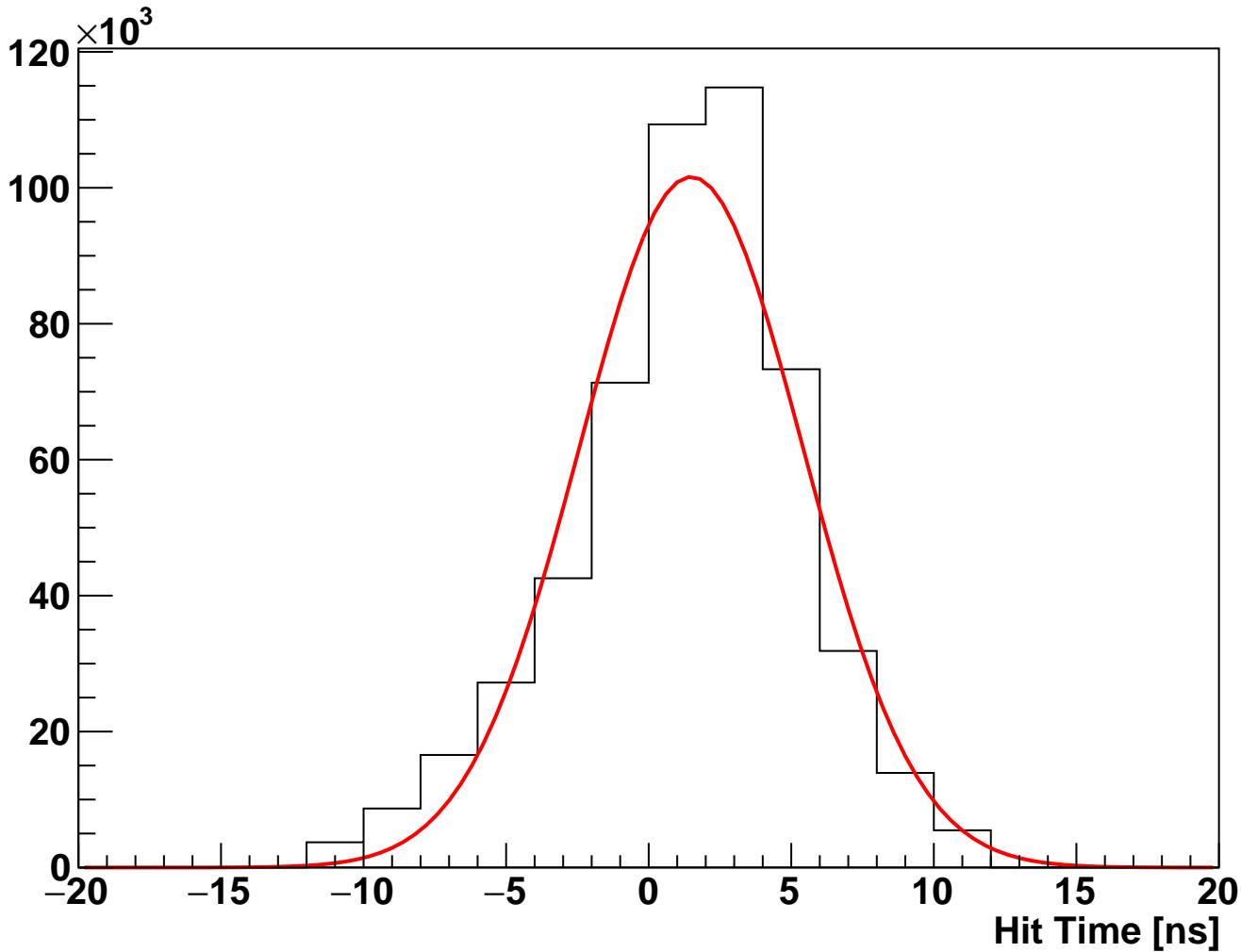
module_L6b_halfmodule_stereo_hole_sensor0 Fitted Hit Time (hits on clean track)
