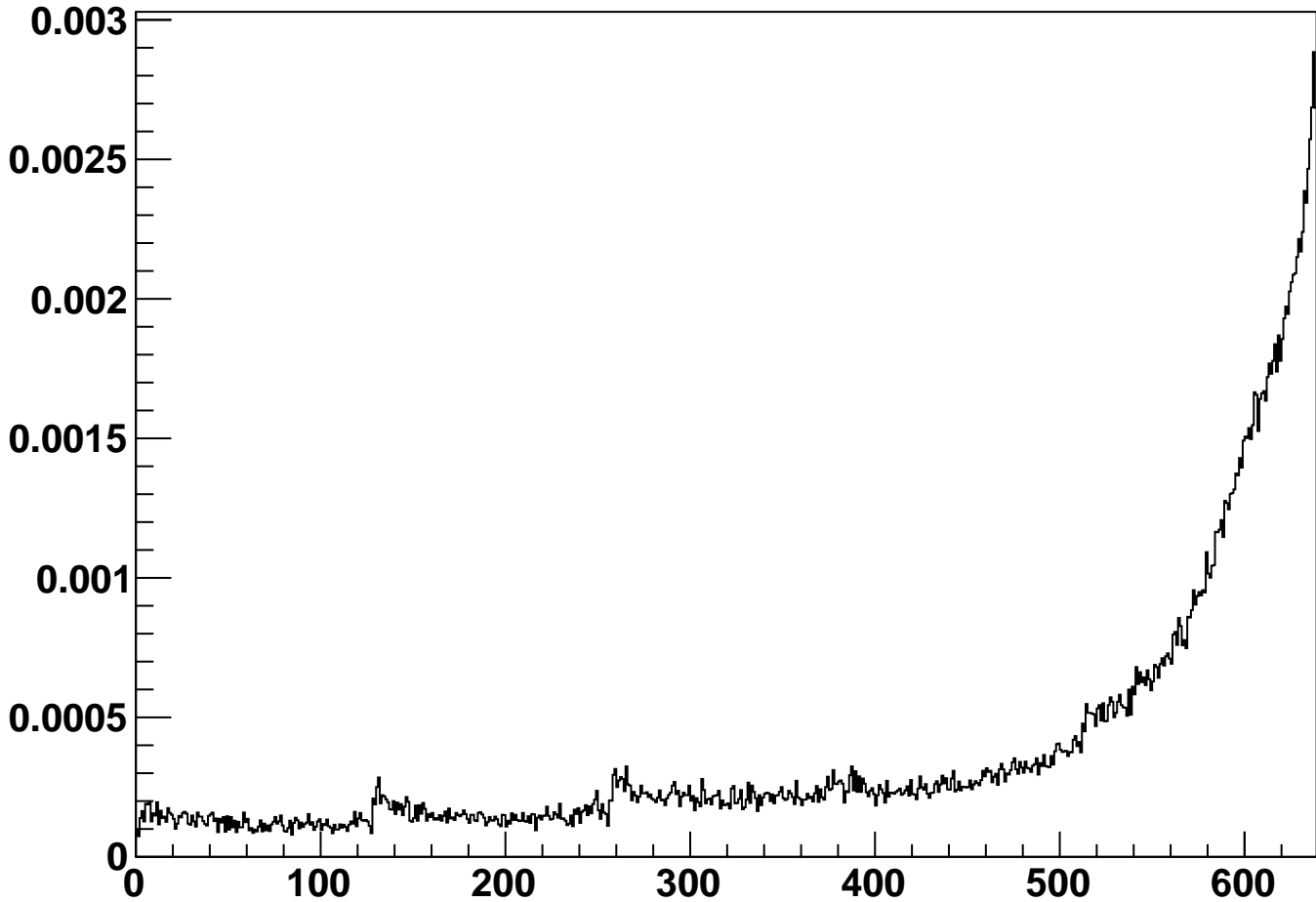
module_L3t_halfmodule_stereo_sensor0 - Occupancy
