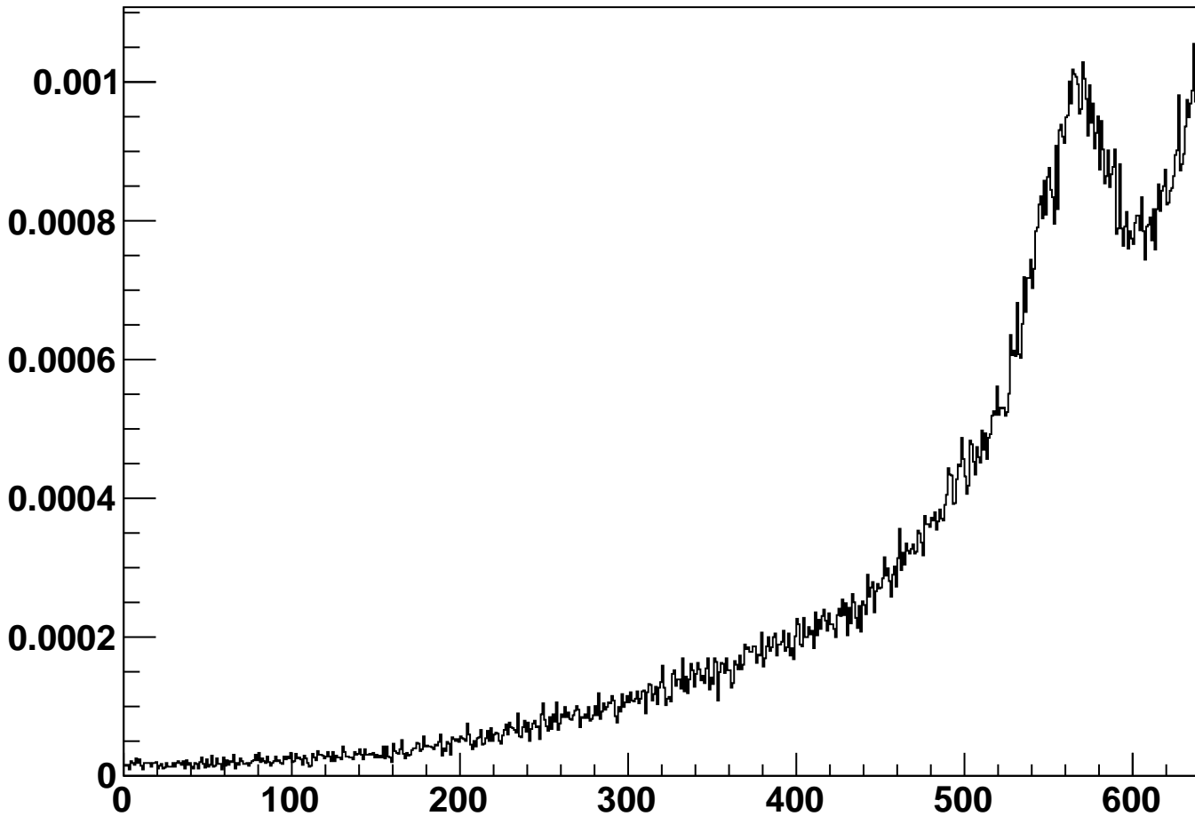
module_L4b_halfmodule_stereo_hole_sensor0 - Cluster Occupancy
