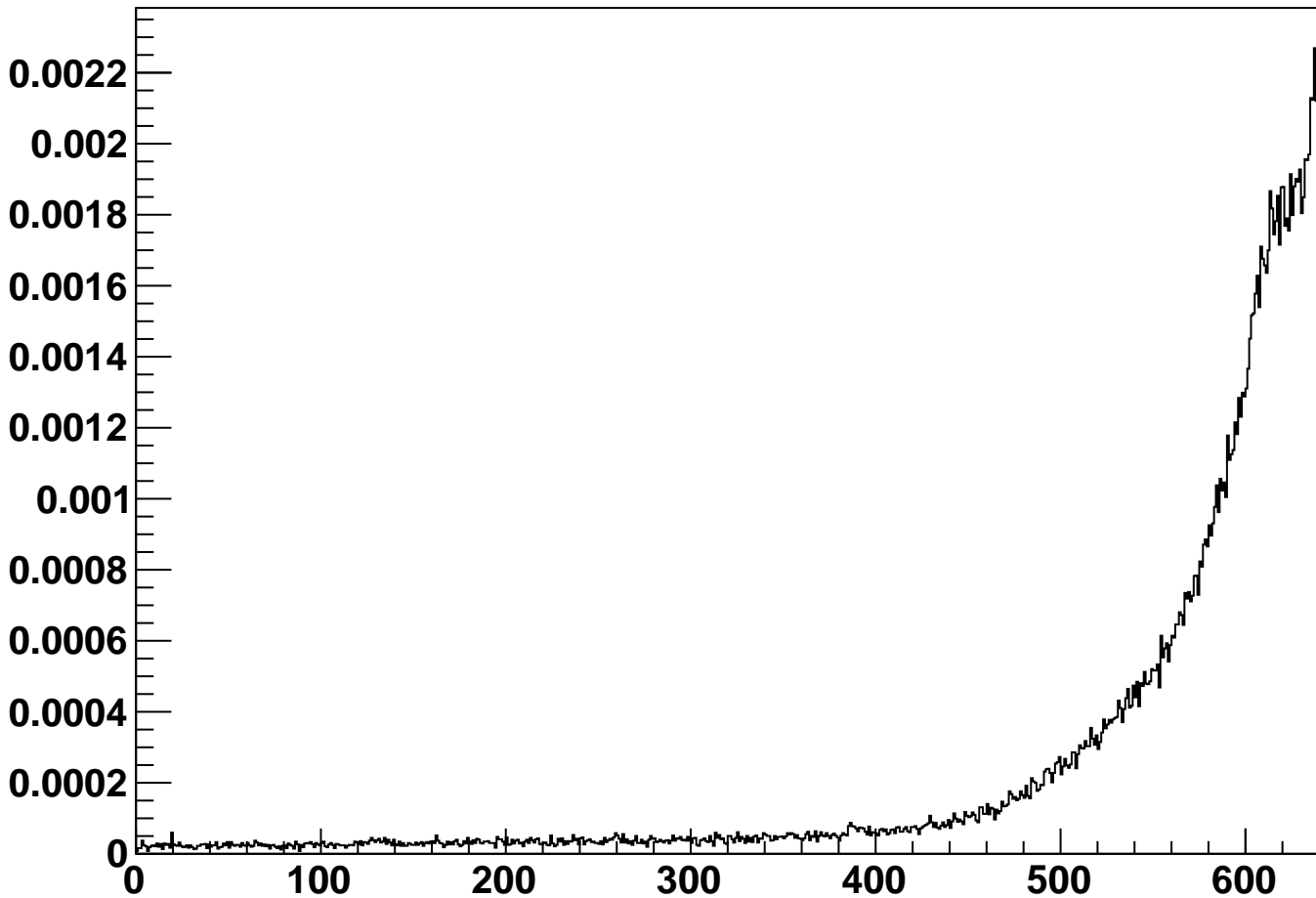
module_L2t_halfmodule_stereo_sensor0 - Cluster Occupancy
