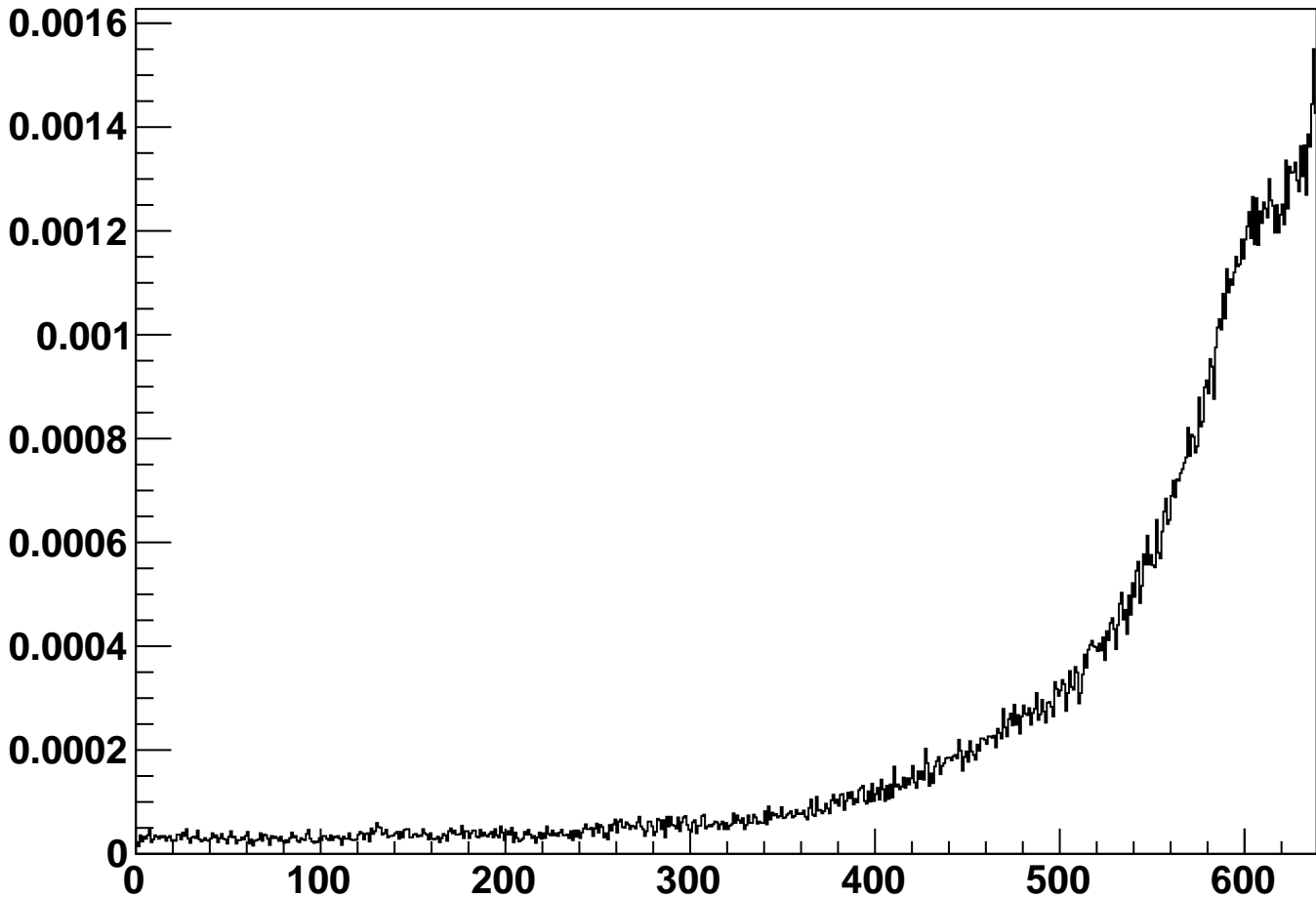
module_L3t_halfmodule_stereo_sensor0 - Cluster Occupancy
