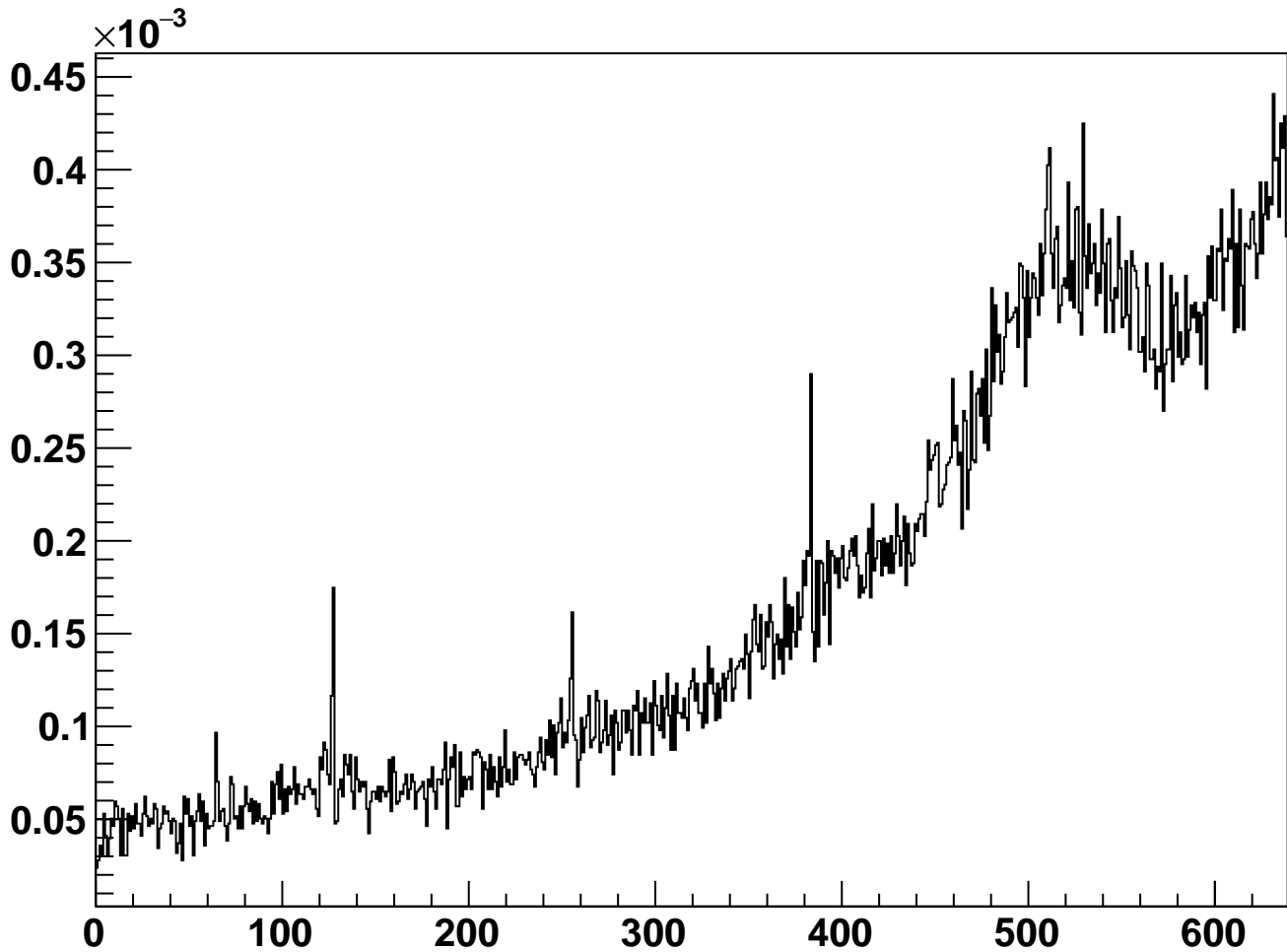
module_L6t_halfmodule_stereo_hole_sensor0 - Cluster Occupancy
