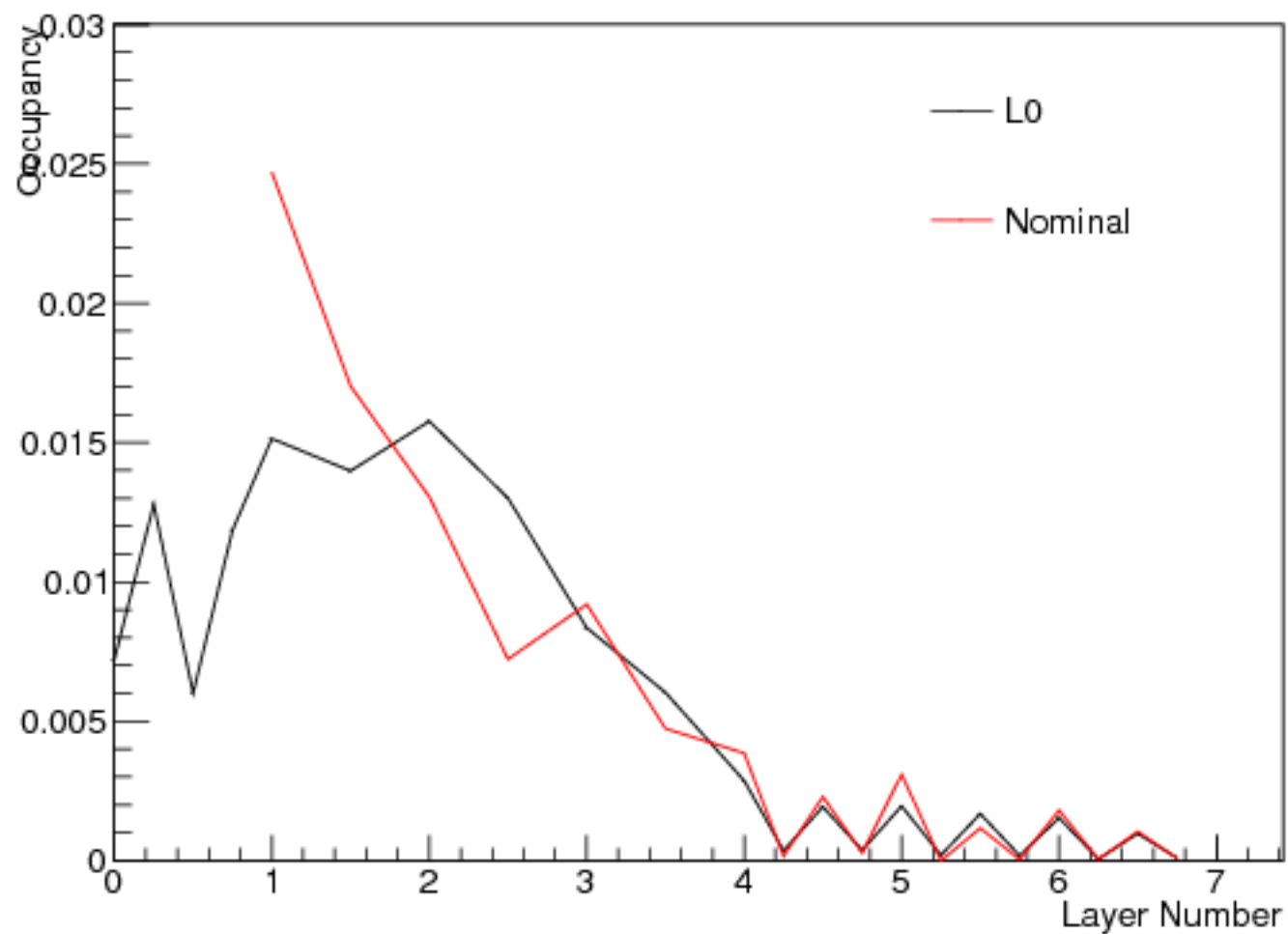
SVT Sensor Edge Strip Occupancies Bottom
