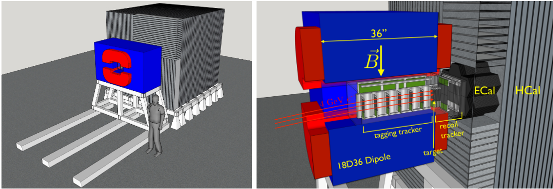
Figure 1: (From [2]) Left: An overview of the LDMX detector showing the full detector apparatus with a person for scale. Right: A cutaway overview of the LDMX detector showing, from left to right, the trackers and target inside the spectrometer dipole, the forward ECal, and the HCal.
