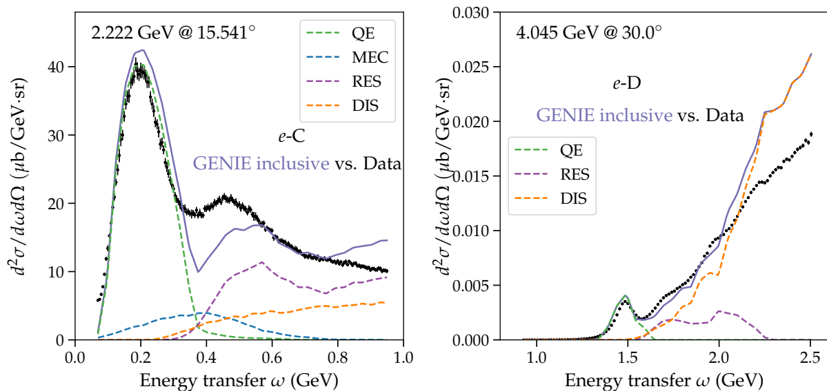
FIG. 1: Left : Comparison of the inclusive GENIE prediction (solid line) to data for electron scattering off carbon at beam energy 2.2 GeV and 15.5^\circ [5], an example of kinematics relevant to DUNE. The individual components contributing to the GENIE cross section are also shown (dashed lines). Large discrepancies beyond the quasielastic peak are apparent. Right : Comparison of GENIE inclusive predictions (solid line) to data for a 4.045 GeV electron scattering off deuterium at 30^\circ [6], where pion-producing processes dominate.
