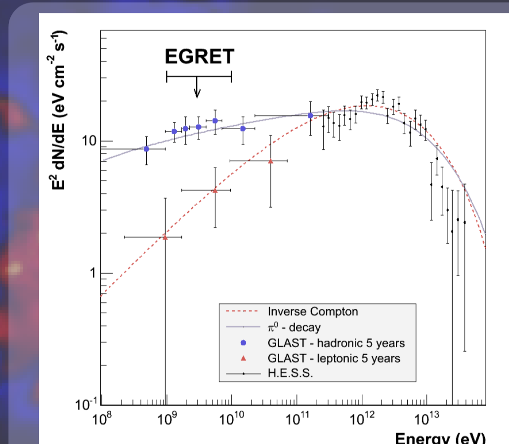
Spectral energy distribution of the shell-type SNR RX J1713.7-3946 above 100 MeV. The black data points denote measurements with H.E.S.S., the blue and red data points correspond to simulated GLAST data assuming different mechanisms for the gamma-ray emission as described in the text.
