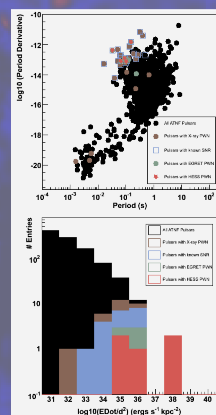
Top: P-Pdot diagram of all ATNF pulsars (black), showing the pulsars with detected X-ray PWN (brown), pulsars for which the corresponding SNR is known (blue), those who can be associated to an EGRET PWN (green) and those associated to a H.E.S.S. VHE PWN (red). Bottom: Energy output distribution for the selections used in the top panel.
