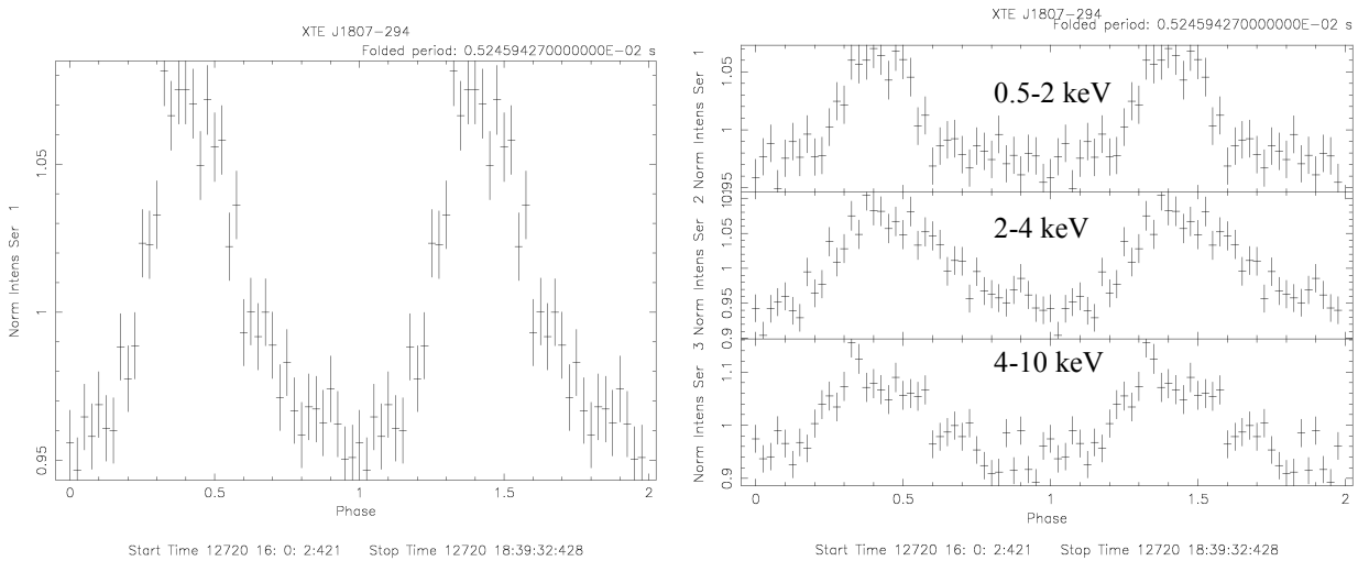
Figure 6: Left: 0.5 to 10 keV pulse profile of single and double events of XTE J1807-294 from EPIC pn Timing mode. Right: Pulse profiles of XTE J1807-294 in three energy bands. Two phase cycles are shown for clarity.
