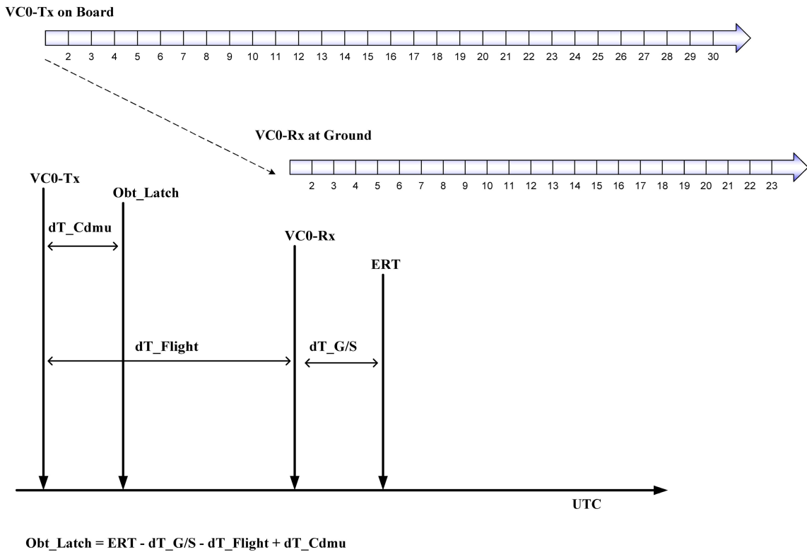
Figure 1: The Timing Information Flow Diagram shows the OBT-UTC time correlation. The formula to correlate OBT and ERT (UTC) is OBT = ERT - dt_{GS} - dt_{FLIGHT} + dt_{CDMU} . The drawing in the lower part shows the correct time model for OBT propagation delay and ERT, where
