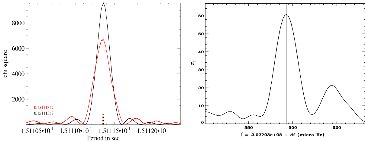
Figure 4: Left: Influence of a time jump of 31 s on the \chi^2 -distribution of epoch folding period search (pulsar period 150 ms).
