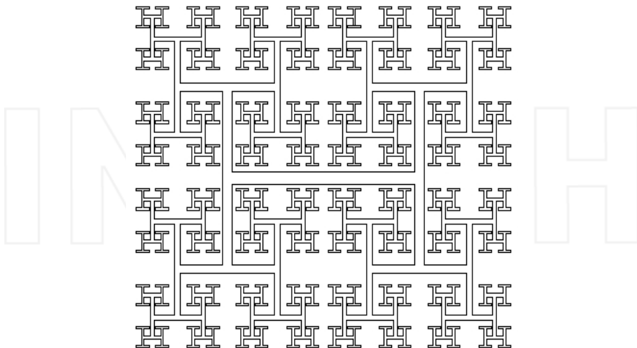
Fig. 3.9. Schematic of the geometric structure of fractal-like microchannel networks with 180° branch angle.
