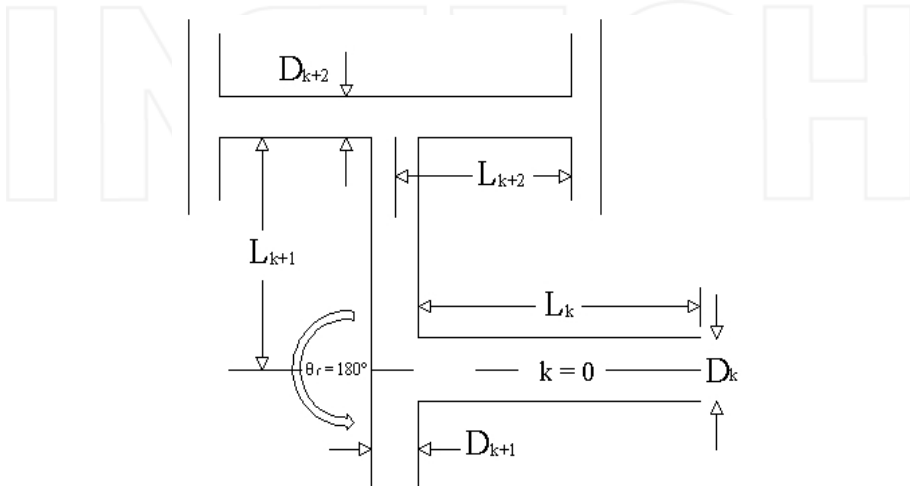
Fig. 3.8. Generation of a fractal-like microchannel networks.
