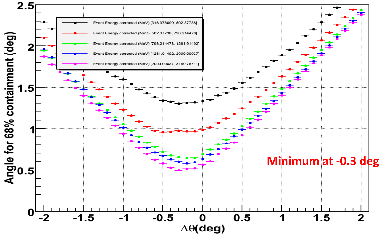
Tower 3 - MC Data - Angular Resolution Vs. Reconstructed Energy at Normal Incidence
