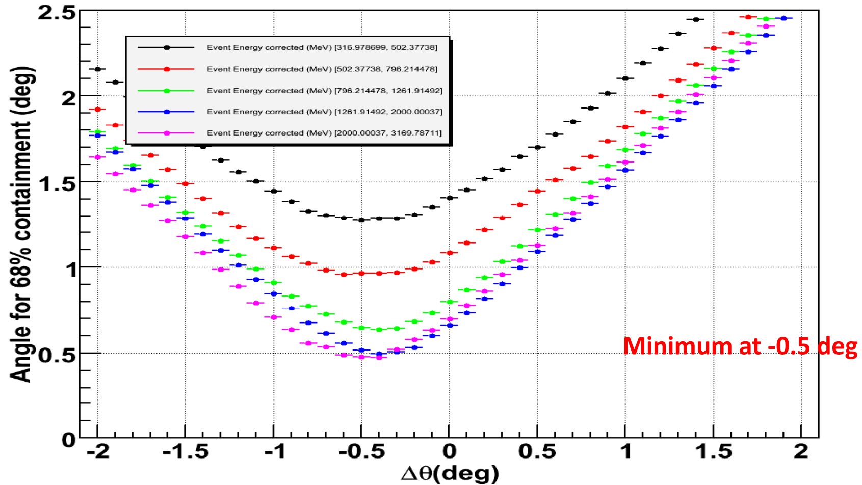
Tower 3 - MC Data - Angular Resolution Vs. Reconstructed Energy at Normal Incidence
