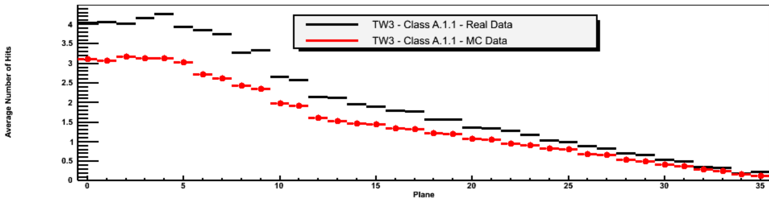
Class A.1.1 - Cluster Size Profile Tower 3
