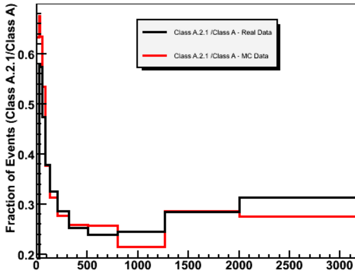
Class A.2.1 Event Energy corrected distribution
