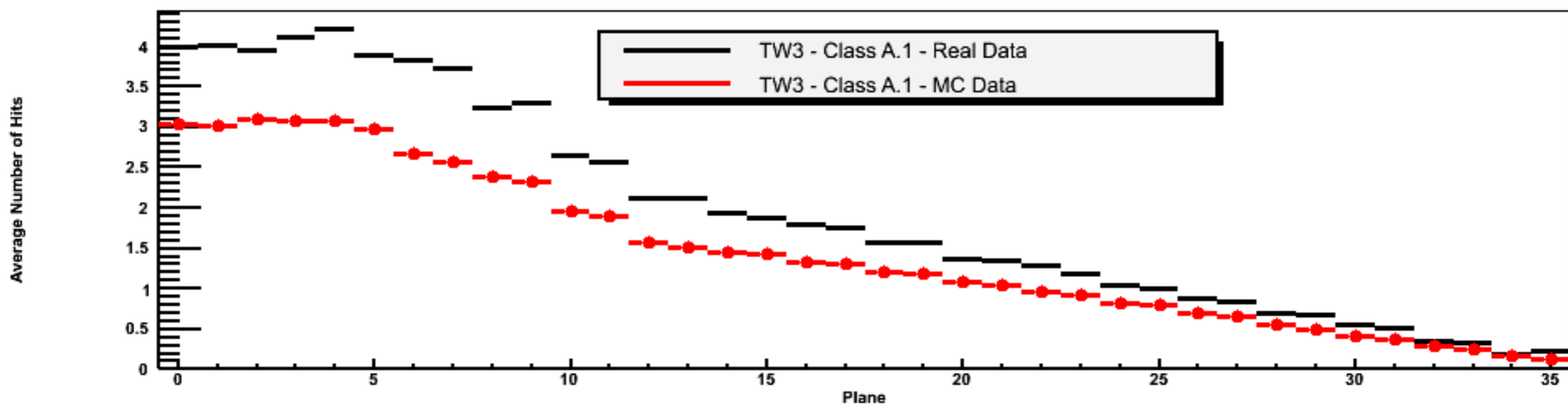
Class A.1 - Cluster Size Profile Tower 3
