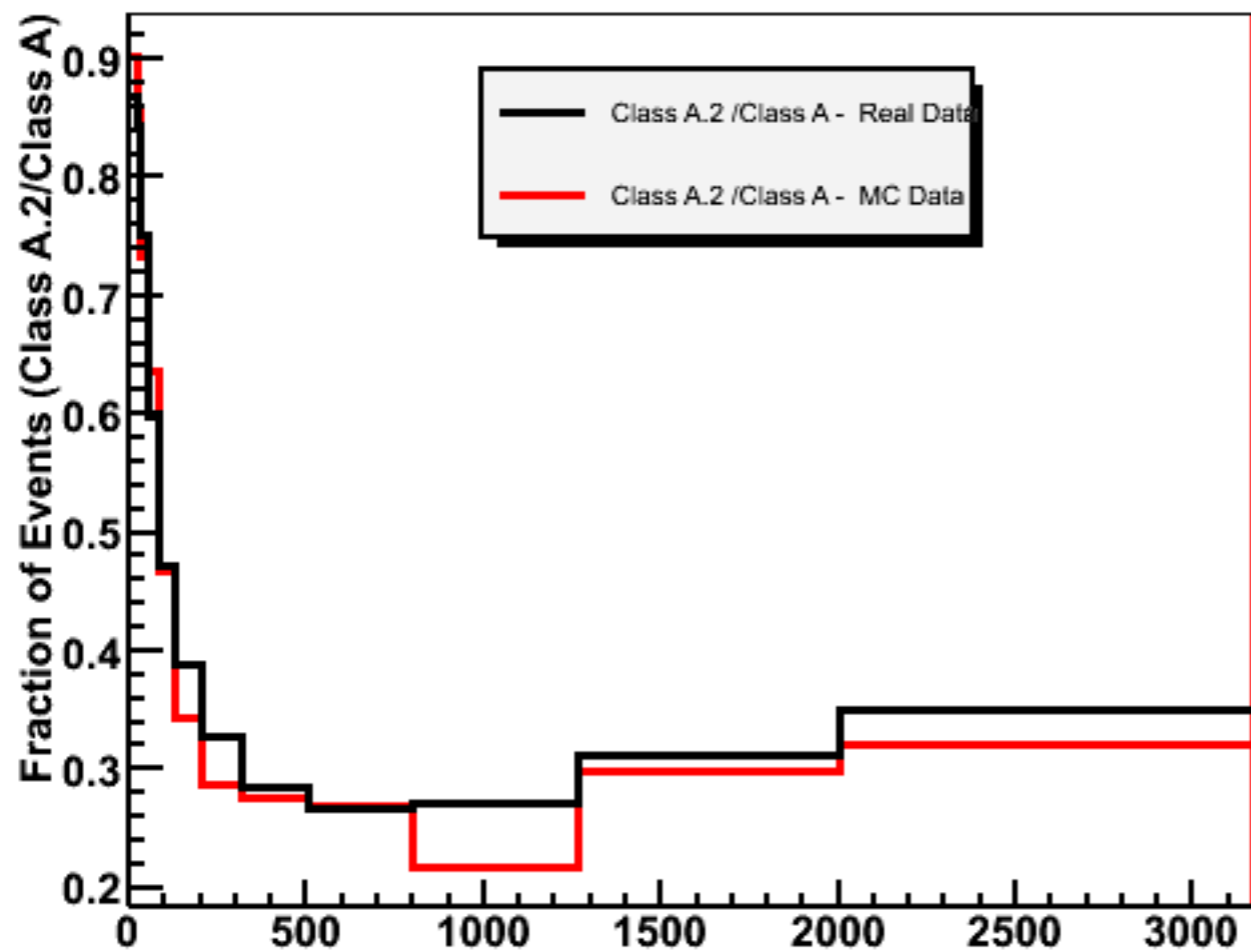
Class A.2 Event Energy corrected distribution
