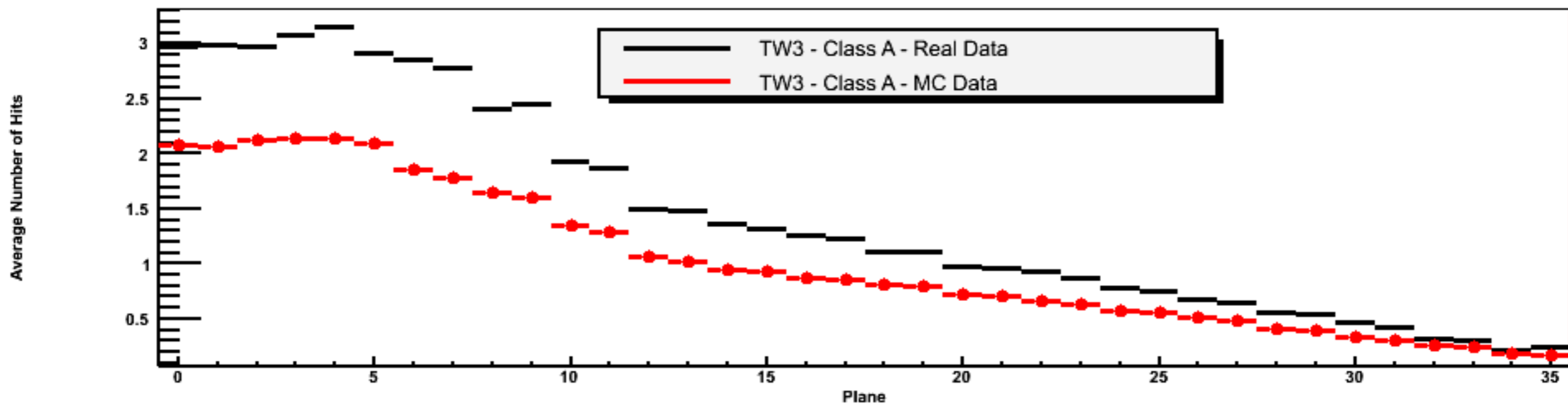
Class A - Cluster Size Profile Tower 3
