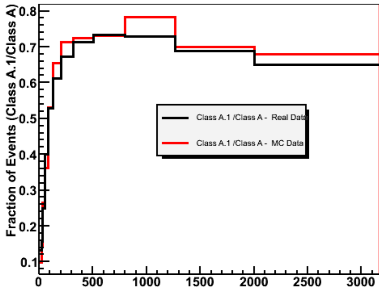
Class A.1 Event Energy corrected distribution
