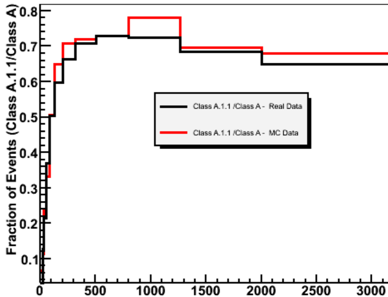
Class A.1.1 Event Energy corrected distribution
