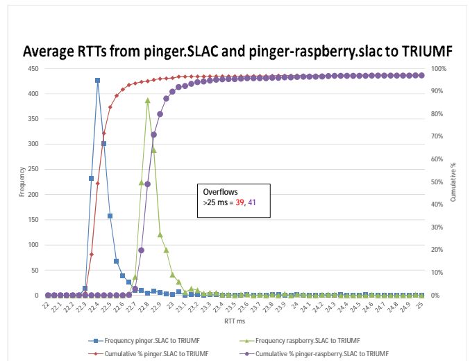
Fig. 2. Average RTTs from pinger.SLAC and pinger-raspberry.slac to TRIUMF
