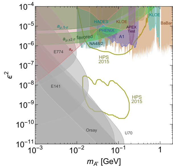
Figure 3. The HPS projected reach corresponding to the 2\sigma limit (yellow line). The green band a_{\mu} \pm 2\sigma ( a_{\mu} \pm 2\sigma ) corresponds to the region where the A' can explain the discrepancy between the experimental value of the muon anomalous magnetic moment, considering a 2\sigma ( 5\sigma ) error, and the corresponding Standard Model calculation.
