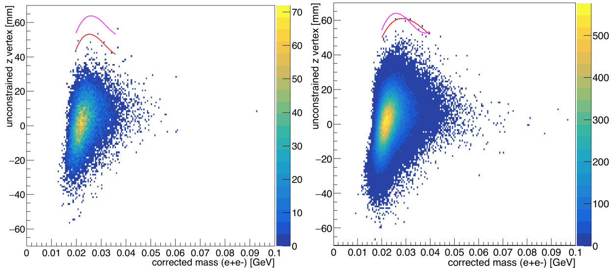
FIG. C.0.7: The unconstrained z vertex position for the L2L2 data with the SVT at \pm 1.5 mm is shown as a function of the corrected mass of the e^+e^- pair where both tracks do not pass through the active region of Layer 1. The zCut as measured for this data is shown in red and corresponds to the full 100% data set where there is less than 0.5 background event beyond. The projected zCut from the 10% of the data is shown in magenta. The relevant mass range used to measure zCut is from 0.02–0.04 GeV based on measured statistics. The 10% sample for tuning cuts is shown on the left, and the full 100% of the data is shown on the right.
