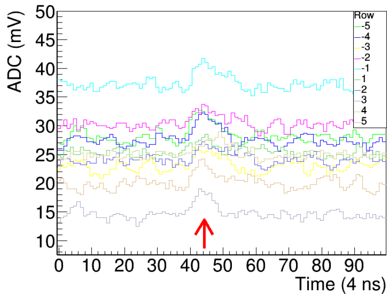
FIG. 4.2.12: The crystal signals plotted versus time for a cosmic ray signal passing vertically through all ten layers of crystals in the ECal. Each crystal's signal is separated vertically in this plot by its pedestal. The arrow indicates the approximate time that the cosmic signal passed through the detector. 1 V corresponds to 4096 FADC channels.
