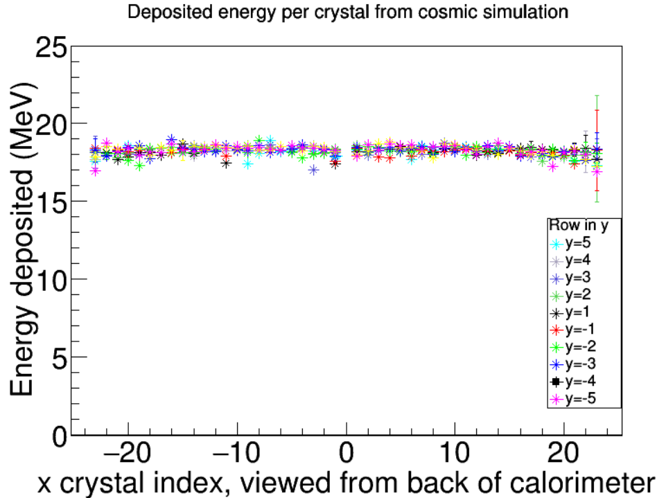
FIG. 4.2.11: The simulated cosmic ray muon energy deposition per crystal of the ECal. The mean energy was 18.3 MeV.
