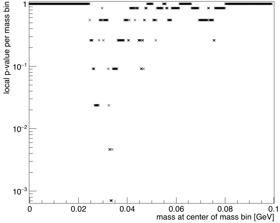
FIG. 6.0.5: The local p -values for each mass hypothesis using the data-characterized background estimate is shown. The p -value shows how well each hypothesis agrees with the background only model. The most significant p -value has a value of 0.00071 at approximately 34 MeV as this bin contains 7 high z background events.
