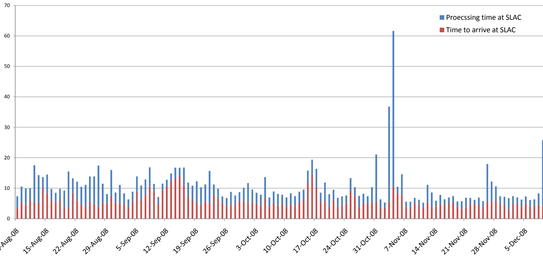
Fermi Data Processing Time (hours)
