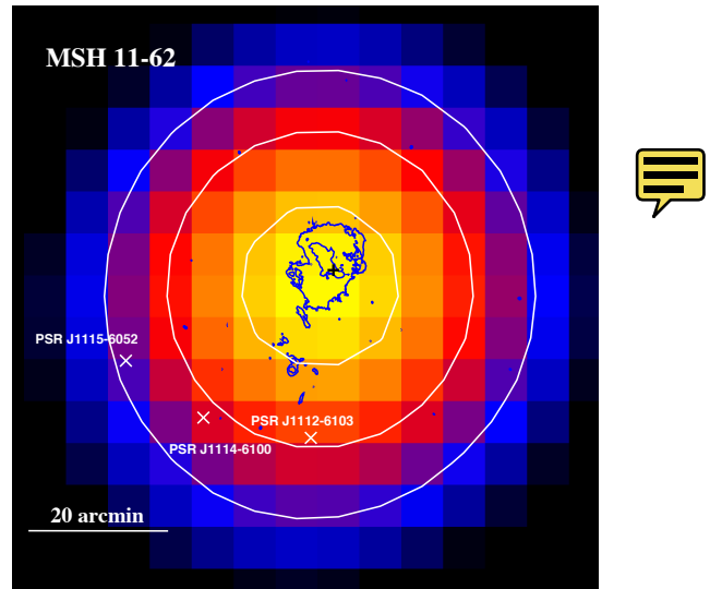
FIG. 7.— TS map of Fermi LAT emission from MSH 11–62. Blue contours correspond to the radio emission, and white contours represent the 13, 15, and 17\sigma significance levels of the flux. Positions of nearby pulsars with \dot{E} > 10^{32} erg s^{-1} are indicated (see discussion in text).
