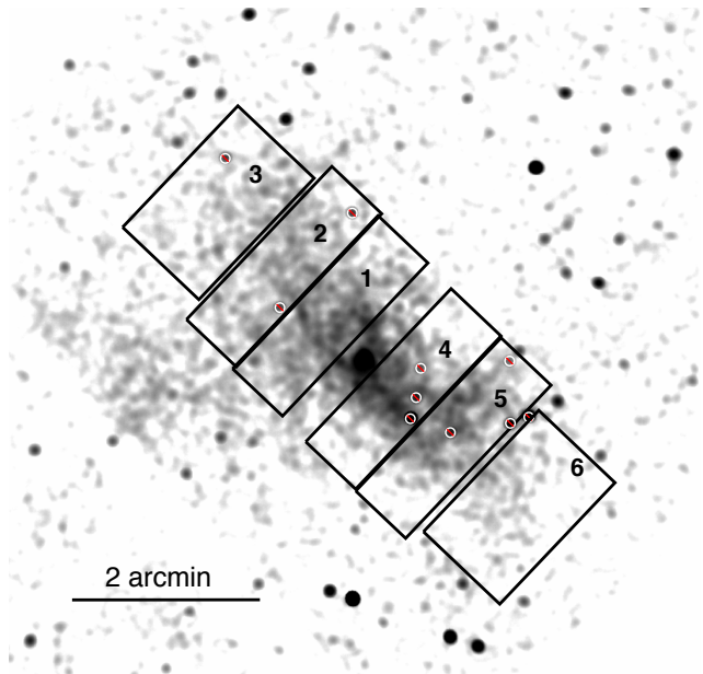
FIG. 3.— Chandra image of PWN in MSH 11–62, along with regions used for extracting spectral index along the nebula (see Table 1). The image has been smoothed with a Gaussian of 5 arcsec width. The pulsar candidate is the bright central source between regions 1 and 4.
