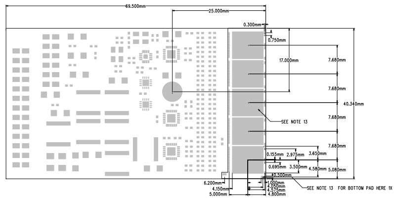
DRILL DRAWING
