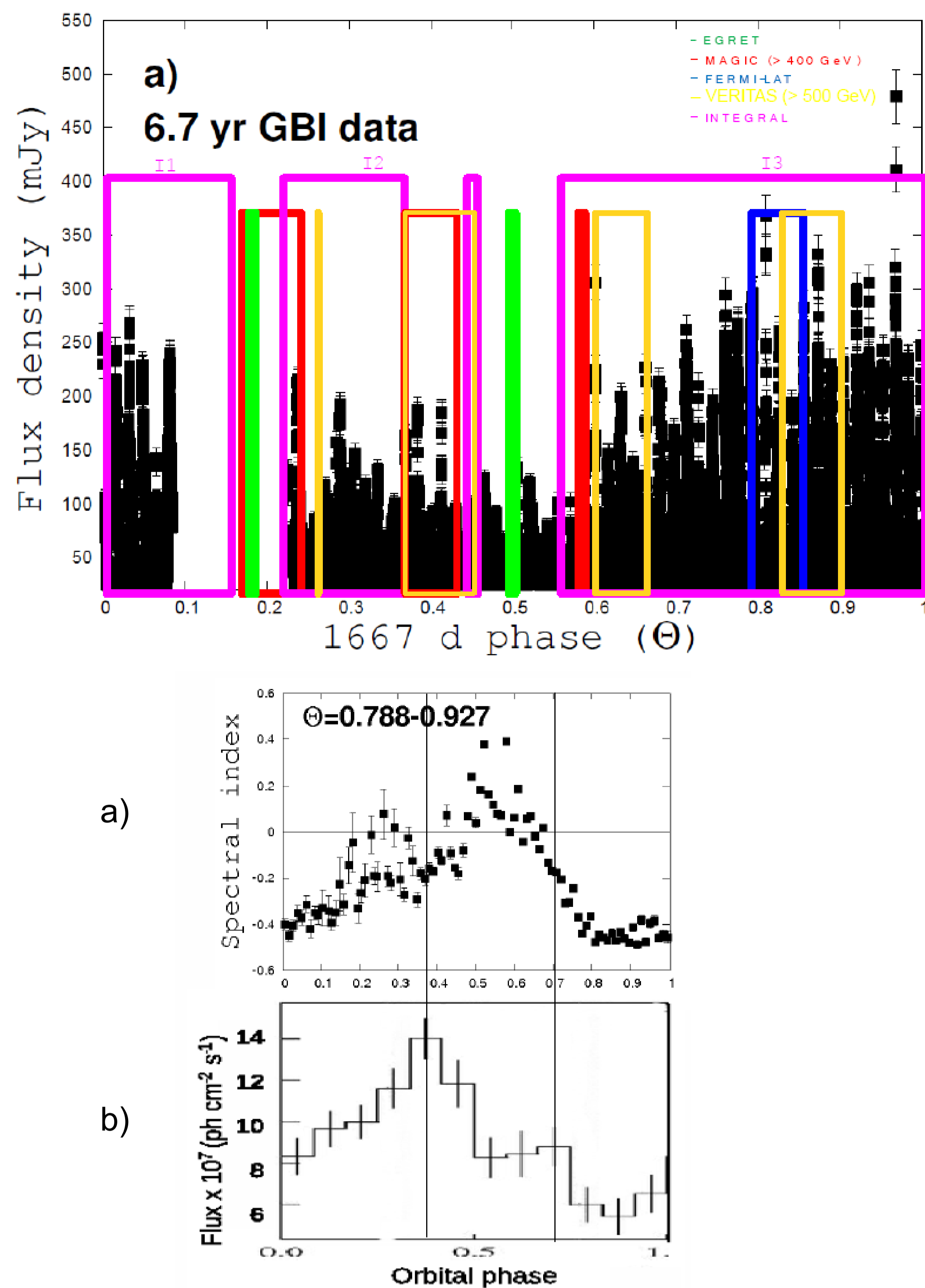
Fig.1 Top: Very high/high energy (VHE/HE) observations of LSI +61°303 by EGRET, MAGIC, Fermi -LAT, VERITAS and INTEGRAL shown in the context of the 4.6 yr radio period ( \theta ) (Zimmermann & Massi 2011, in prep.). The three largest \theta intervals where the source was observed with INTEGRAL are named here I1, I2 and I3.
