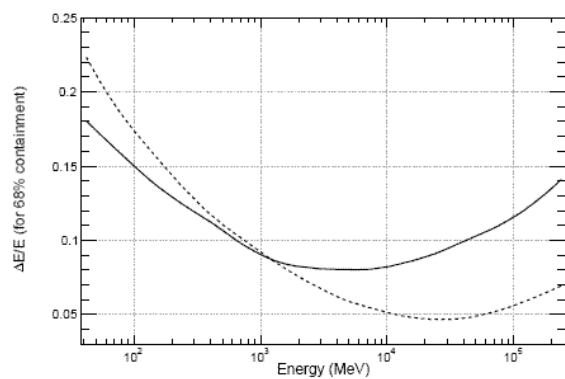
FIG. 18.— Energy resolution versus energy for normal incidence (solid curve) and at 60° off-axis (dashed curve).
